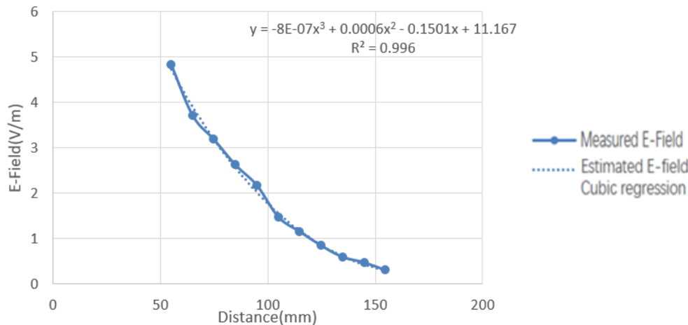
Model 3: Cubic Regression
