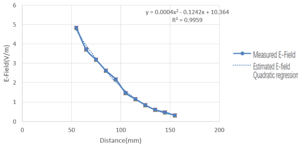
Model 2: Quadratic Regression
