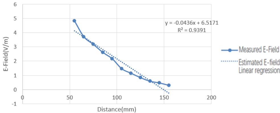
Model 1: Linear regression
