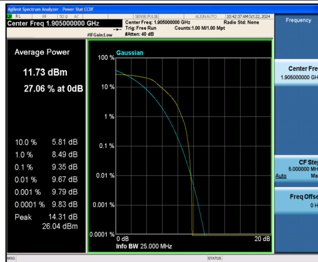
Band2-10MHz-QPSK-19150-6-0-Low-9.35-&lt;=13-PASS
