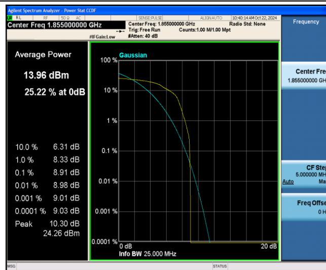
Band2-10MHz-16QAM-18650-1-0-Low-8.91-&lt;=13-PASS
