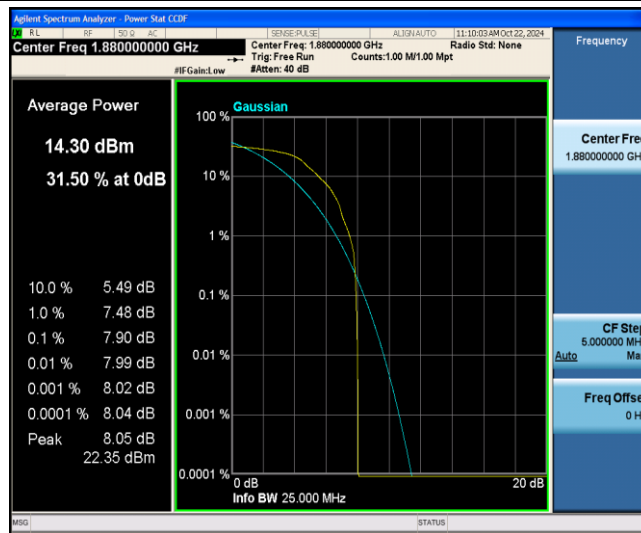
Band2-15MHz-QPSK-18900-1-0-Low-7.90-&lt;=13-PASS
