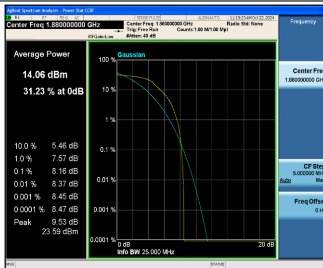
Band2-15MHz-QPSK-18900-6-0-Low-8.16-&lt;=13-PASS
