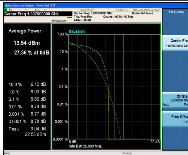
Band2-5MHz-16QAM-19175-1-0-Low-8.66-&lt;=13-PASS
