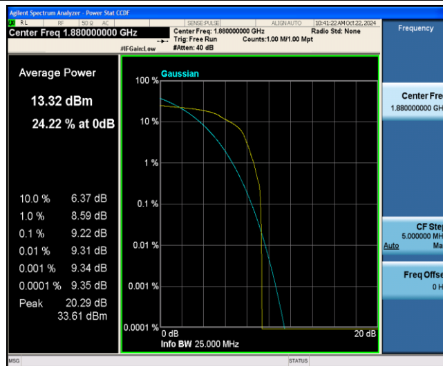
Band2-10MHz-16QAM-18900-1-0-Low-9.22-&lt;=13-PASS
