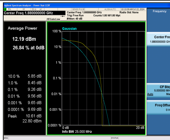
Band2-5MHz-16QAM-18900-6-0-Low-9.26-&lt;=13-PASS
