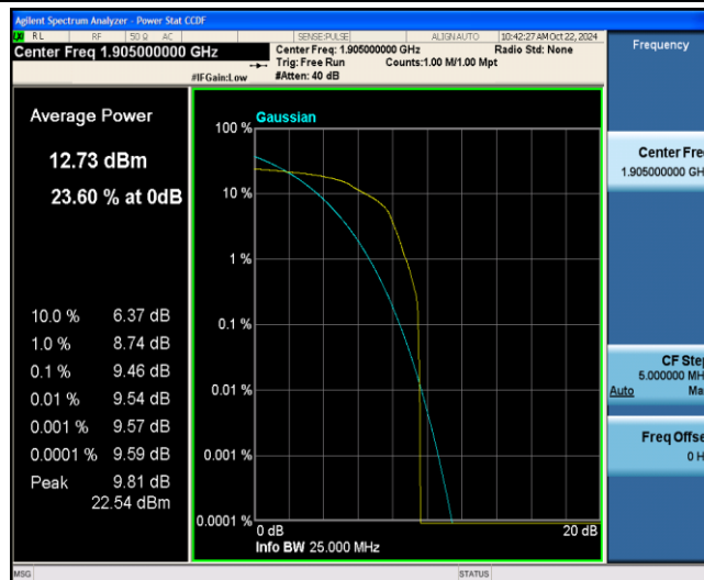
Band2-10MHz-16QAM-19150-1-0-Low-9.46-&lt;=13-PASS
