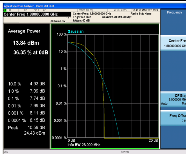
Band2-10MHz-16QAM-18900-6-0-Low-7.74-&lt;=13-PASS
