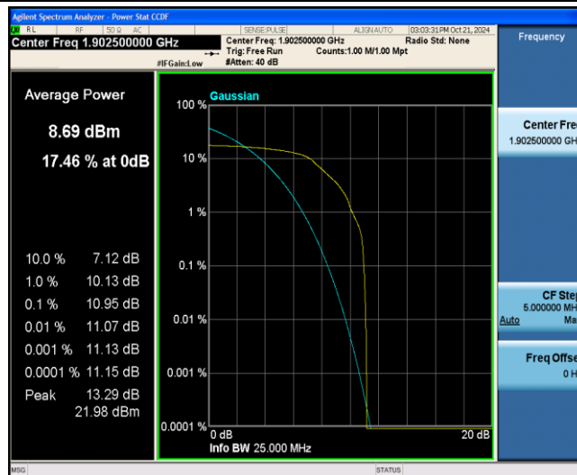
Band2-15MHz-QPSK-19125-1-0-Low-10.95-&lt;=13-PASS
