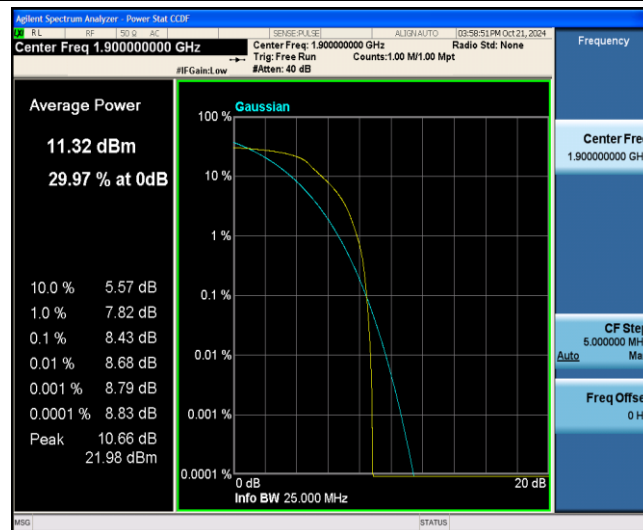
Band2-20MHz-16QAM-19100-6-0-Low-8.43-&lt;=13-PASS
