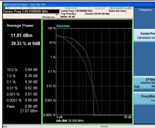
Band2-3MHz-16QAM-18615-6-0-Low-9.26-&lt;=13-PASS
