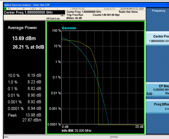
Band2-5MHz-16QAM-18900-1-0-Low-8.82-&lt;=13-PASS
