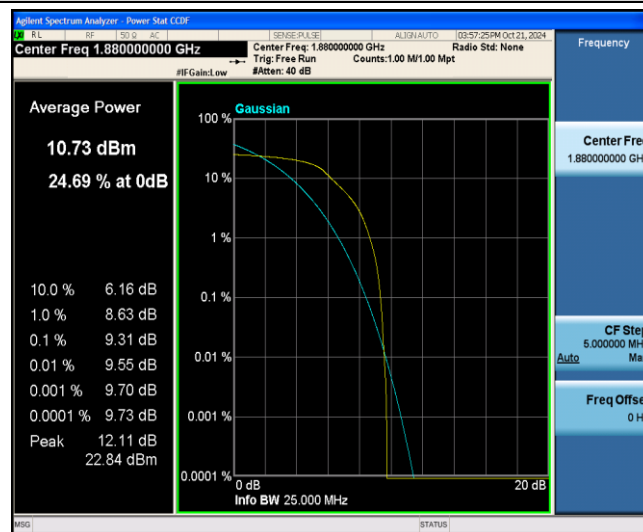
Band2-20MHz-16QAM-18900-6-0-Low-9.31-&lt;=13-PASS
