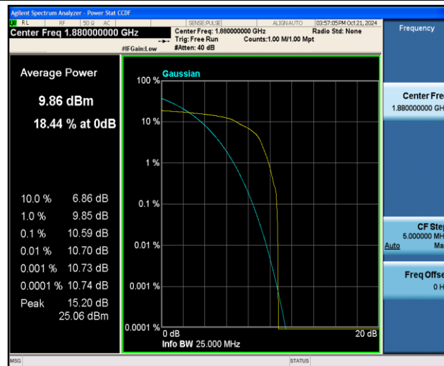
Band2-20MHz-16QAM-18900-1-0-Low-10.59-&lt;=13-PASS
