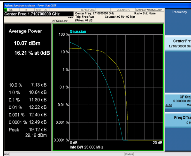
Band4-1.4MHz-QPSK-19957-6-0-Low-11.80-&lt;=13-PASS
