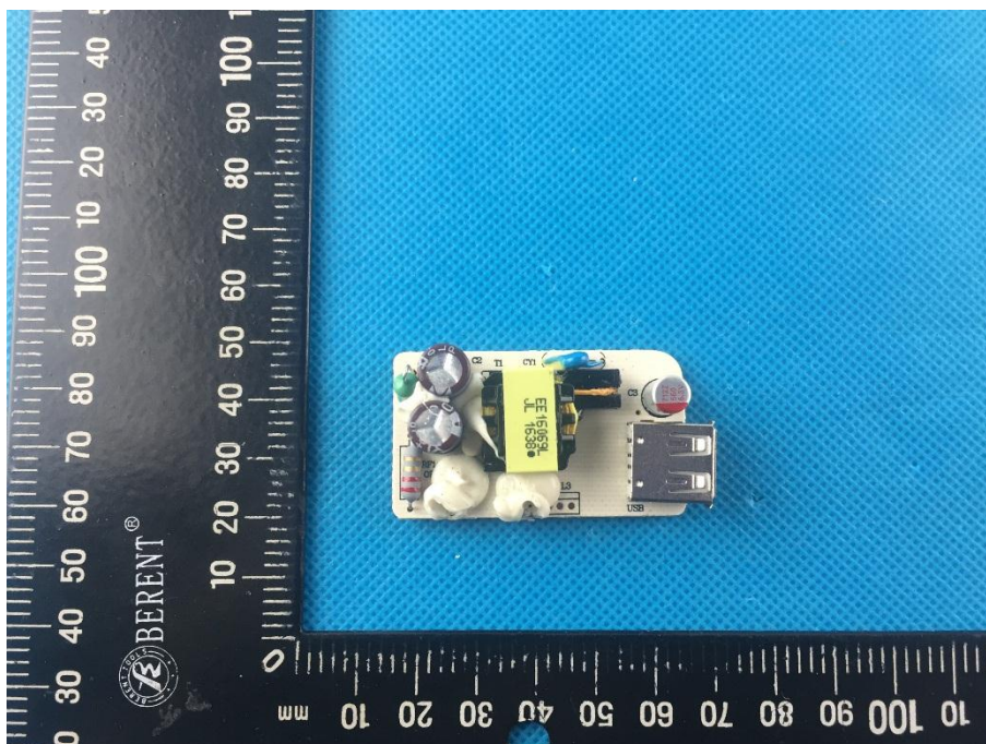
Picture10 : Front of the Adapter main board(CB01)
