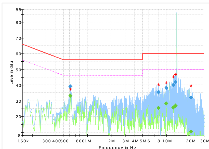
Figure 4 TX mode (150kHz-30MHz)
