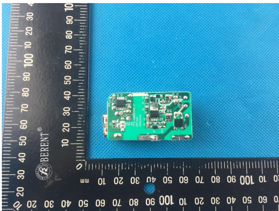
Picture11 : Back of the Adapter main board(CB01)
