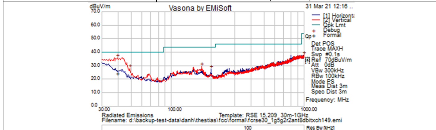
TX Spurious Emissions from 30MHz-1GHz – Ch149 (5745 MHz)
