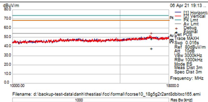
TX Spurious Emissions from 10GHz-18GHz – Ch165 (5825 MHz)
