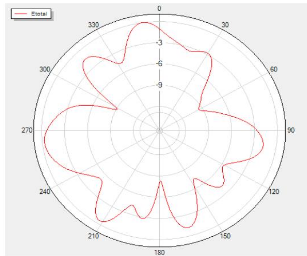
Phi=90 Freq=2472MHz
