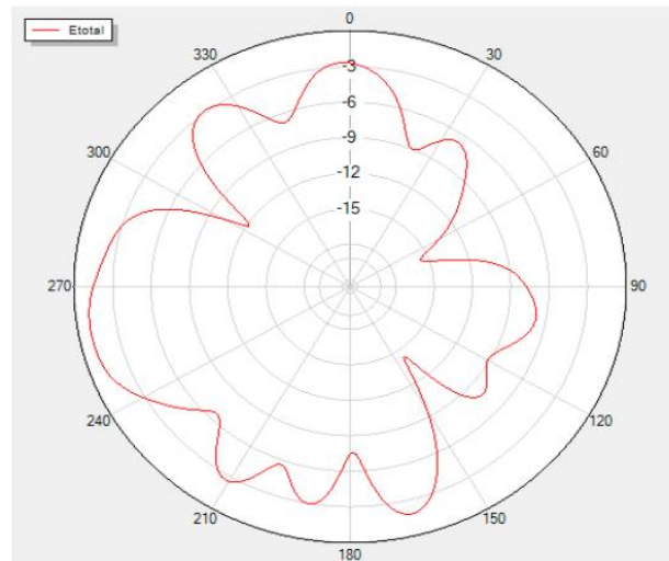
Phi=90 Freq=2402MHz
