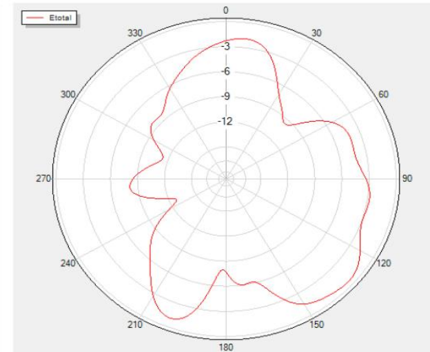
Phi=0 Freq=2410MHz
