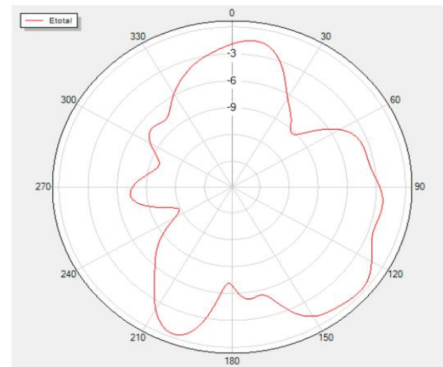
Phi=0 Freq=2416MHz
