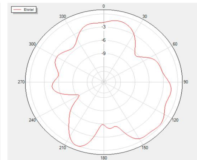
Phi=0 Freq=2454MHz
