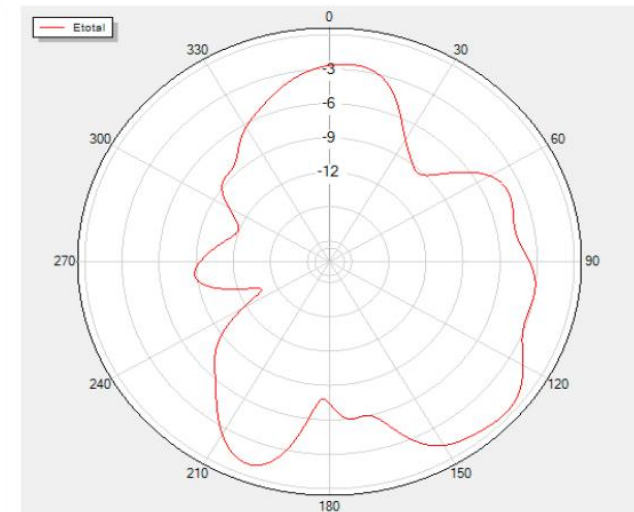
Phi=0 Freq=2402MHz
