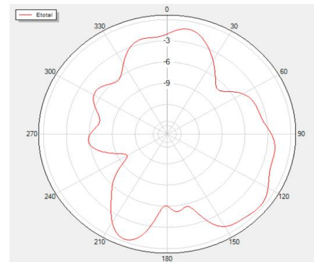
Phi=0 Freq=2440MHz
