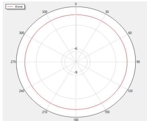
Theta=0 Freq=2422MHz
