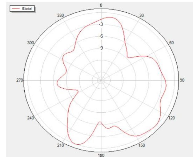
Phi=0 Freq=2422MHz
