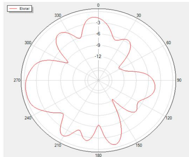
Phi=90 Freq=2422MHz
