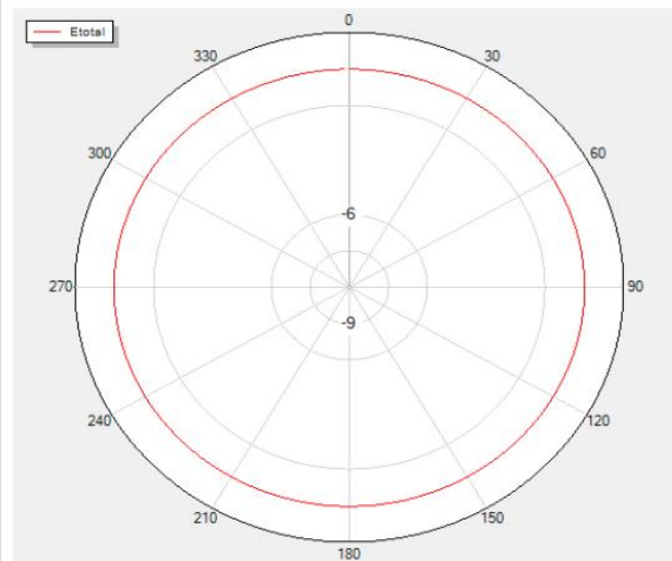
Theta=0 Freq=2440MHz
