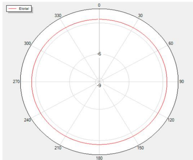
Theta=0 Freq=2402MHz
