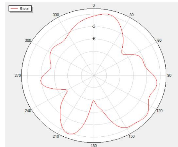
Phi=0 Freq=2480MHz
