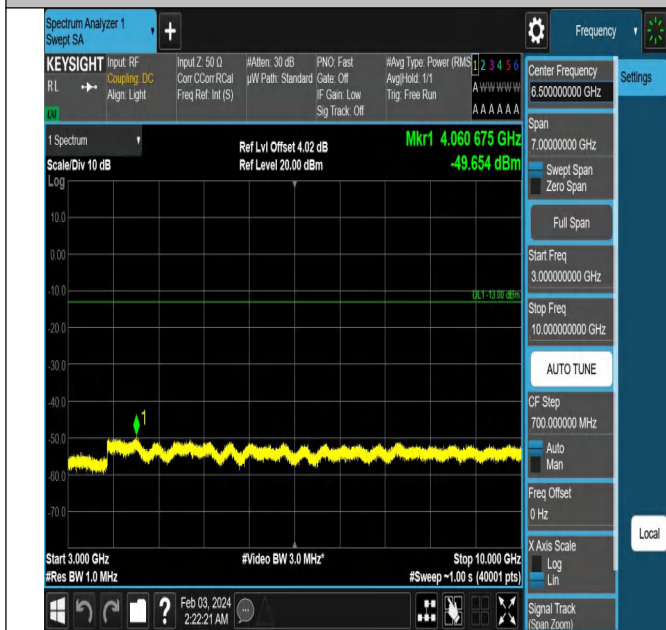
Band5_10MHz_QPSK_20525_1RB#0_3000~10000_3000~10
