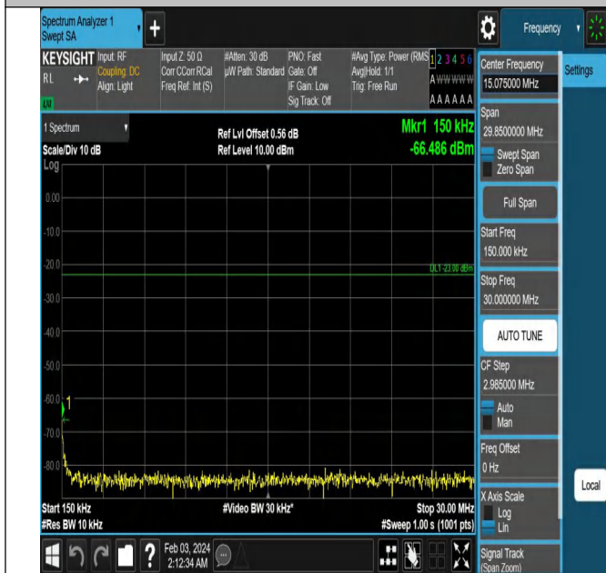
Band5_3MHz_QPSK_20635_1RB#0_0.15~30_0.15~30
