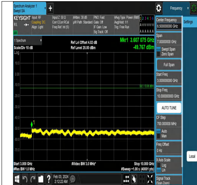
Band5_3MHz_QPSK_20525_1RB#0_3000~10000_3000~10000
