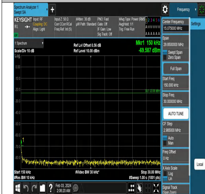
Band5_1.4MHz_QPSK_20525_1RB#0_0.15~30_0.15~30
