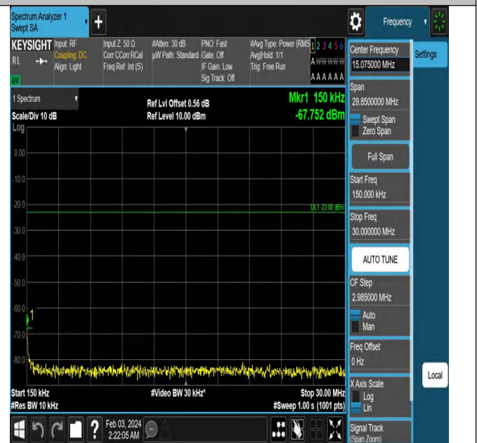
Band5_10MHz_QPSK_20525_1RB#0_0.15~30_0.15~30
