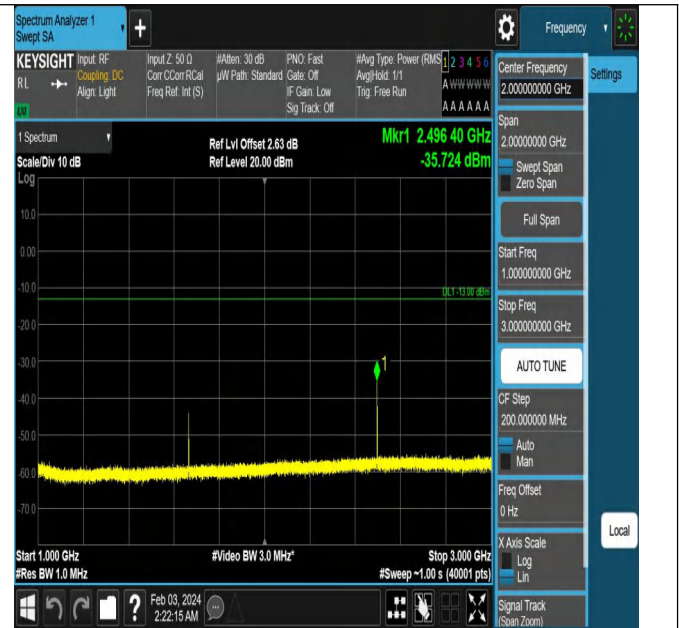
Band5_10MHz_QPSK_20525_1RB#0_1000~3000_1000~300
