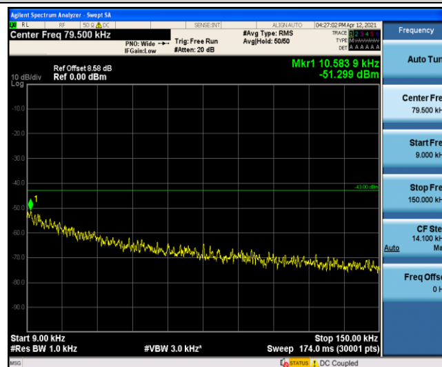
Band5-1.4MHz-16QAM-20525-1-0-Low-0.009-0.15--51.3-PASS
