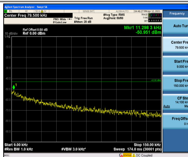
Band5-3MHz-QPSK-20415-1-0-Low-0.009-0.15--50.95-PASS
