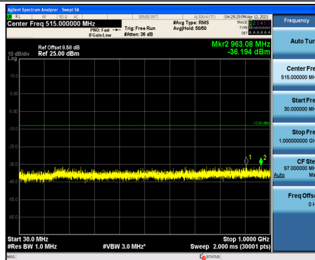
Band5-1.4MHz-QPSK-20643-1-0-High-30-1000--36.19-PASS
