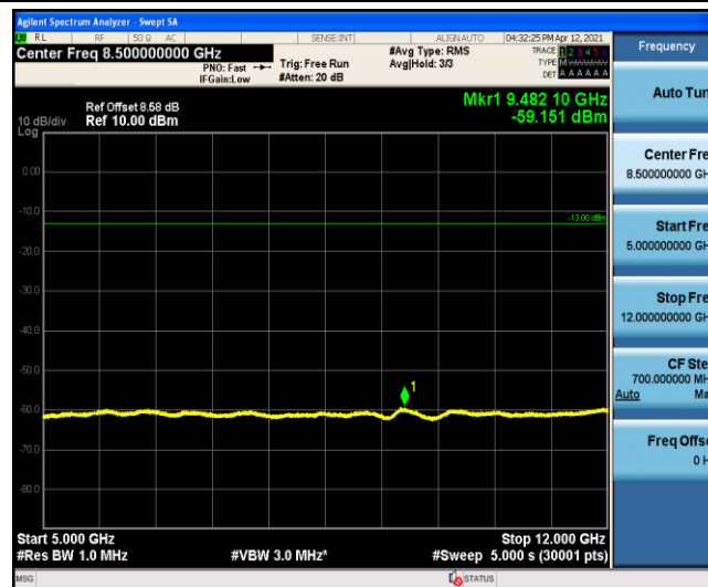
Band5-1.4MHz-16QAM-20643-1-0-High-5000-12000--59.15-PASS
