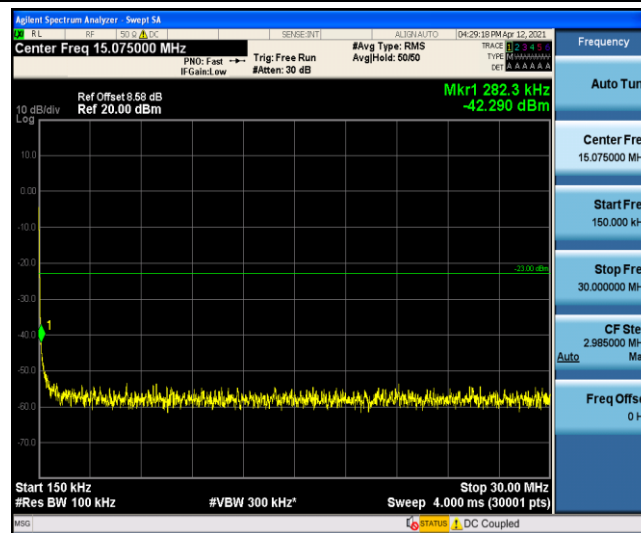
Band5-1.4MHz-QPSK-20643-1-0-High-0.15-30--42.29-PASS
