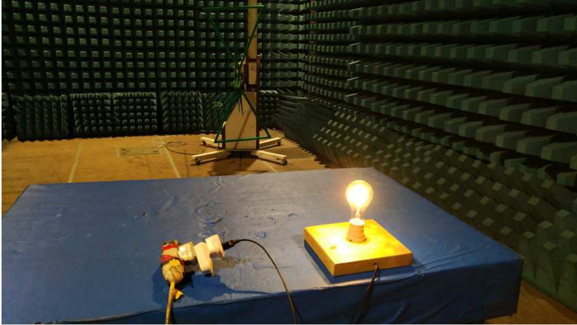
Below 1GHz
