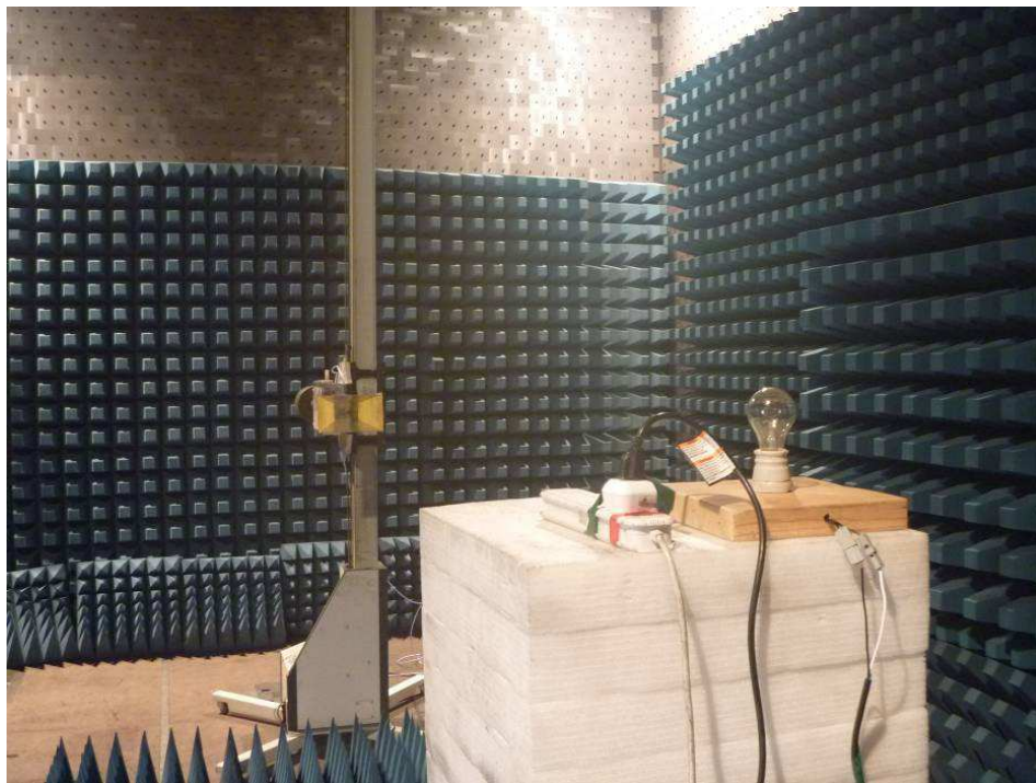
Above 1GHz
