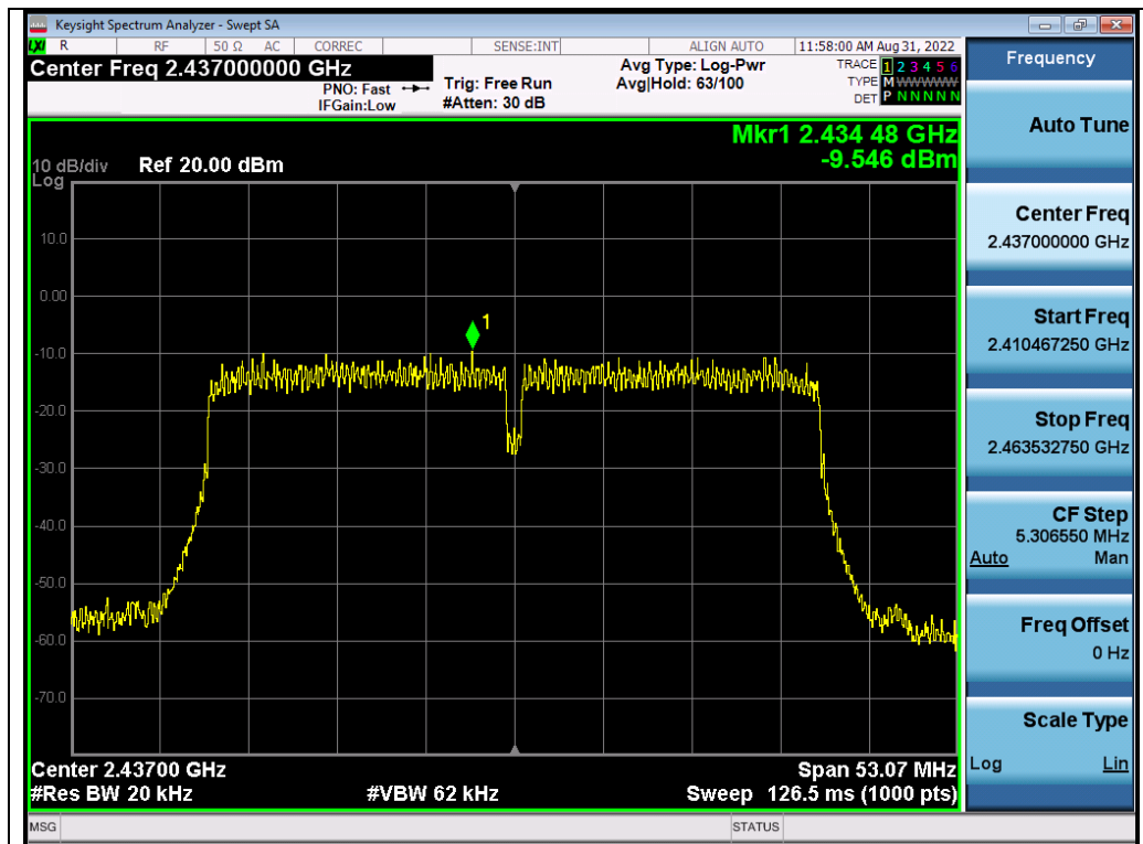
Test_Graph_802.11n40_ANT3_2437_MCS0_PSD
