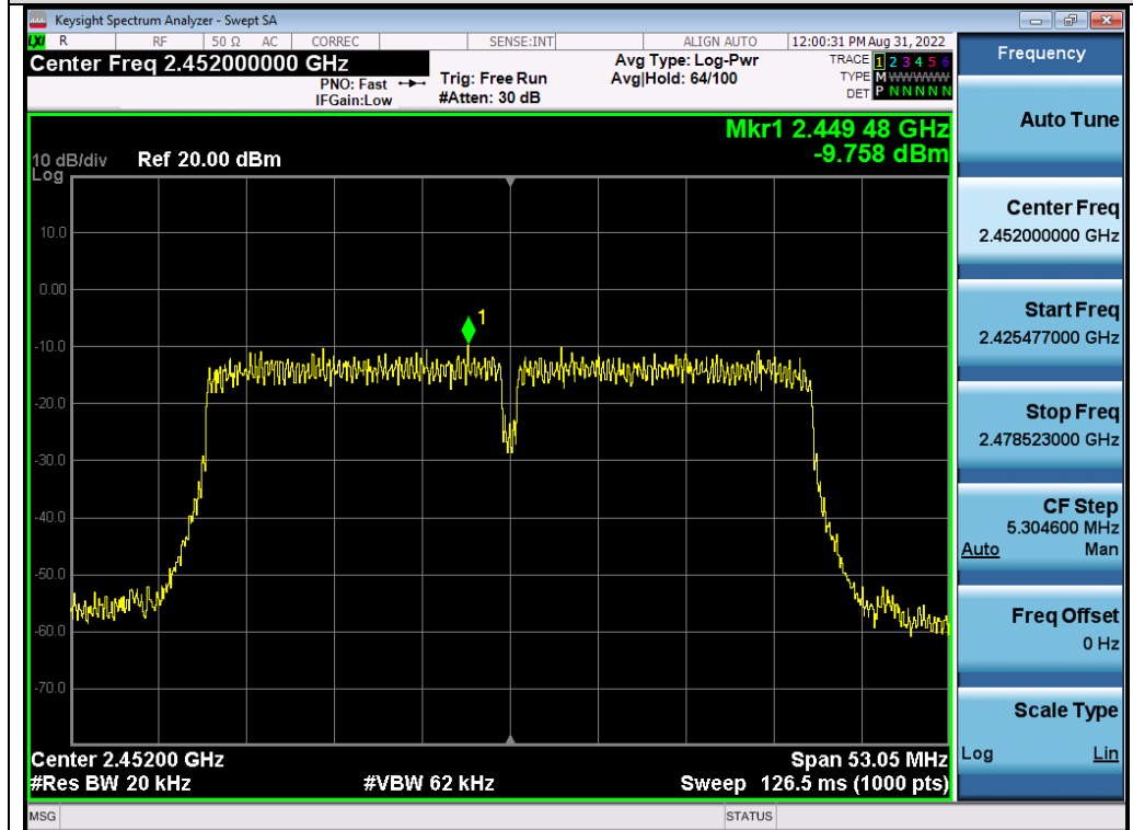
Test_Graph_802.11n40_ANT3_2452_MCS0_PSD
