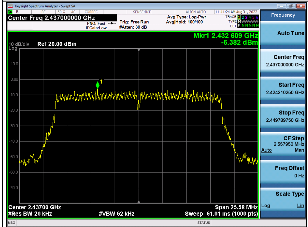
Test_Graph_802.11n20_ANT3_2437_MCS0_PSD
