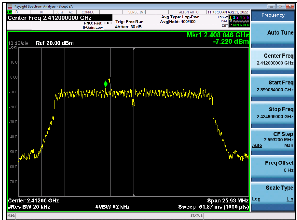
Test_Graph_802.11n20_ANT3_2412_MCS0_PSD
