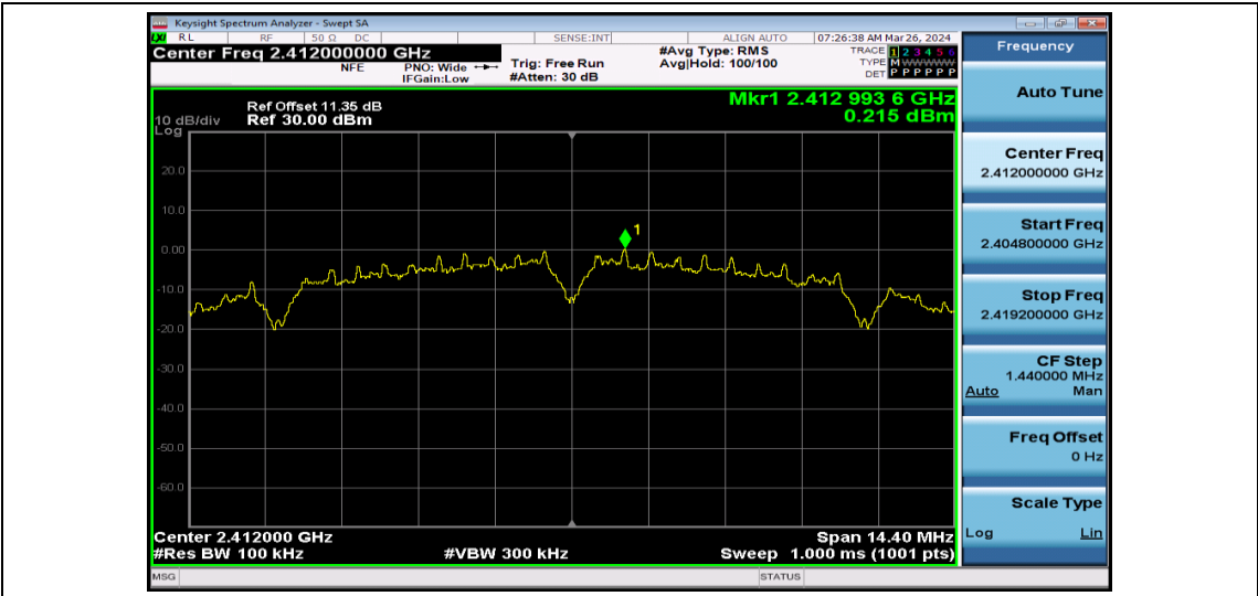
11B-Ant1-2412-PASS
