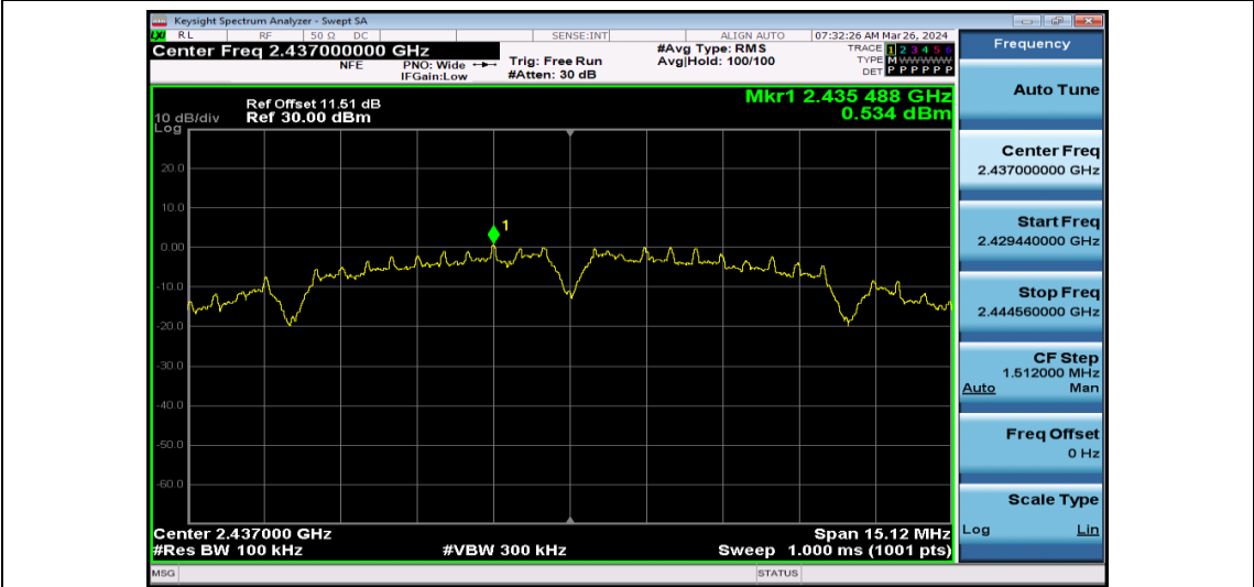
11B-Ant1-2437-PASS
