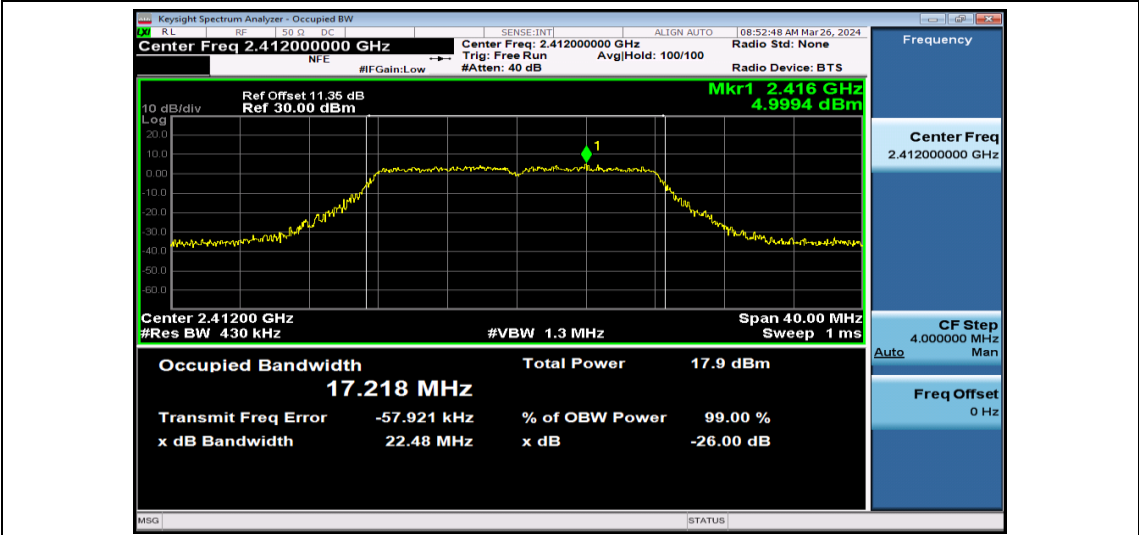
11G-Ant1-2412
