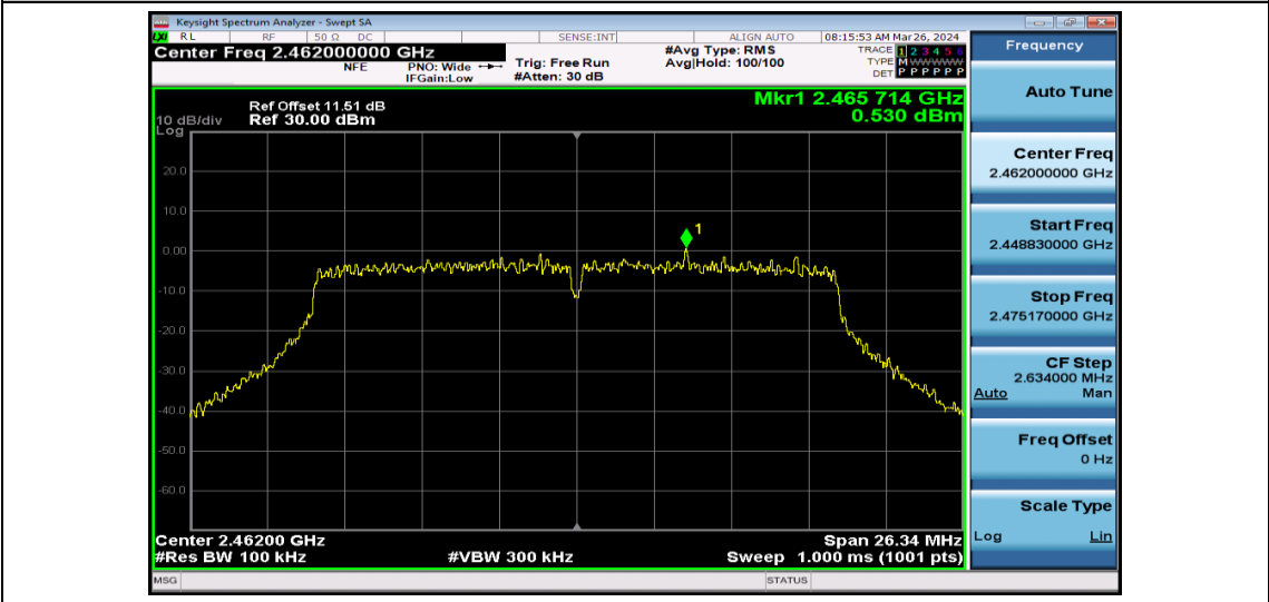
11N20SISO-Ant1-2462-PASS
