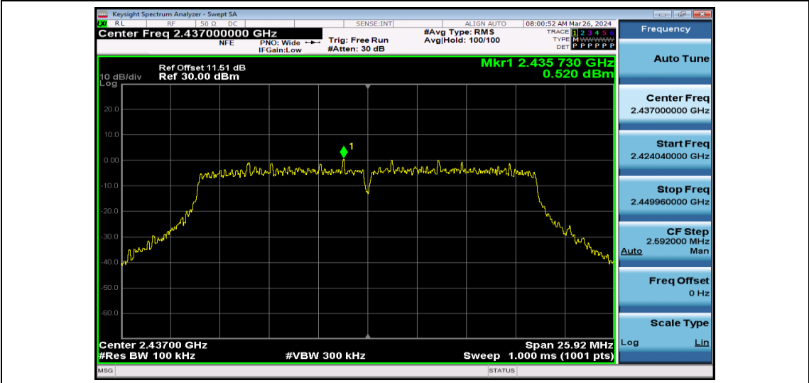
11N20SISO-Ant1-2437-PASS
