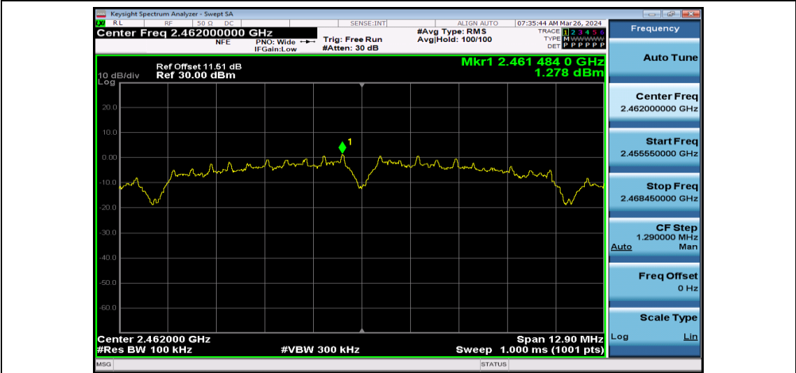
11B-Ant1-2462-PASS
