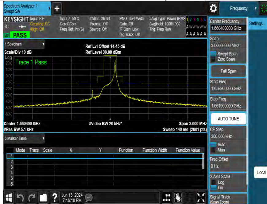
Band255-3.75kHz-MASK-H-BPSK-1@1
