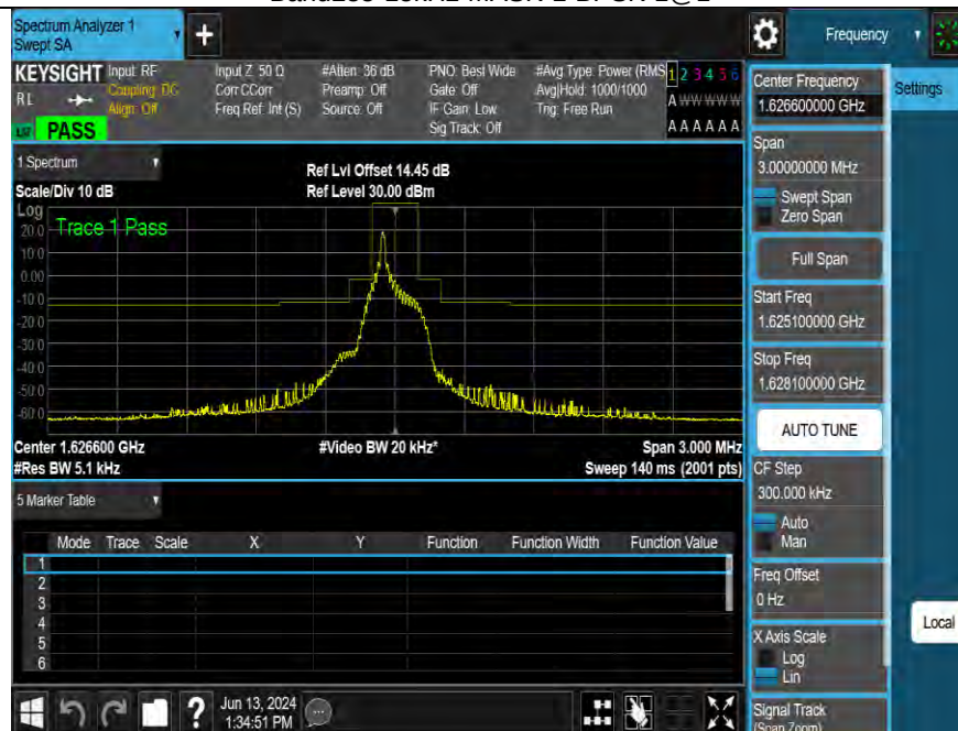
Band255-15kHz-MASK-L-BPSK-1@1
