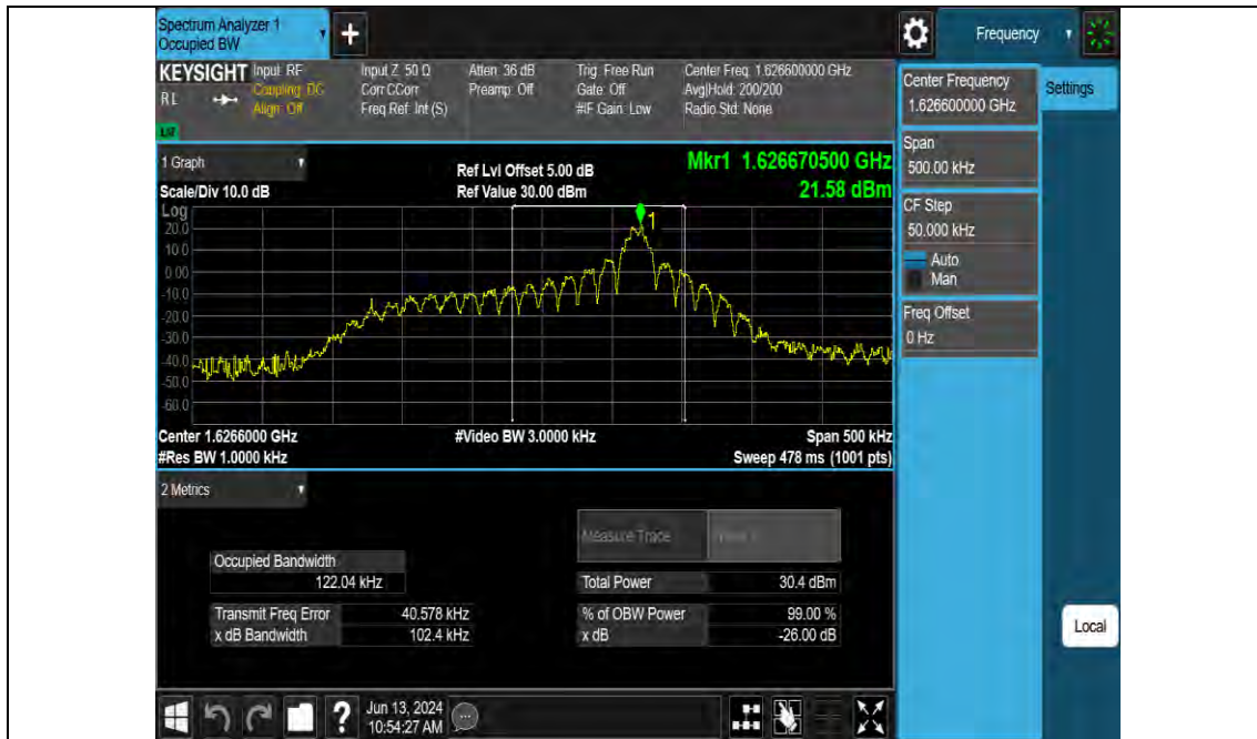
Band255-15kHz-OBW-L-BPSK-1@1
