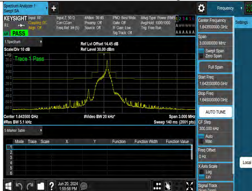
Band255-15kHz-MASK-M-BPSK-1@10
