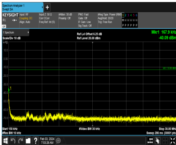
WCDMA 850_RMC 12.2kps_MCH
