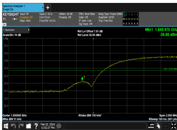
WCDMA1900_HSUPA_ Lowest Channel
