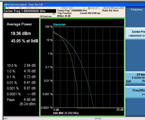
Band2-3MHz-16QAM-18900-15RB#0-PASS
