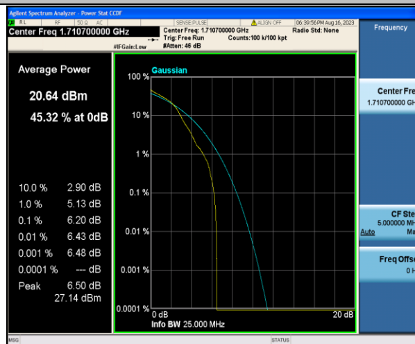
Band4-1.4MHz-16QAM-19957-1RB#0-PASS
