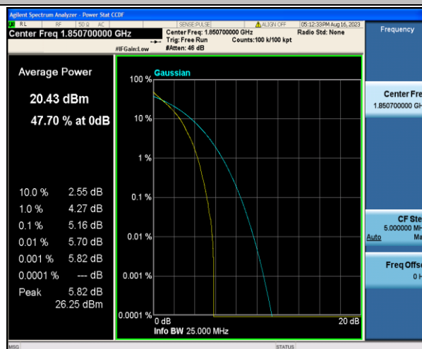
Band2-1.4MHz-QPSK-18607-6RB#0-PASS
