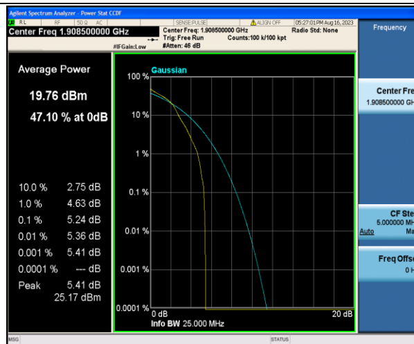
Band2-3MHz-16QAM-19185-1RB#0-PASS
