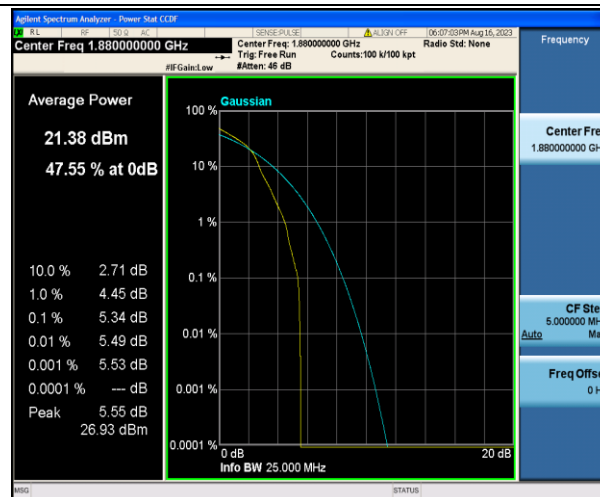
Band2-15MHz-16QAM-18900-1RB#0-PASS
