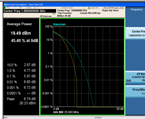
Band2-1.4MHz-16QAM-18900-6RB#0-PASS
