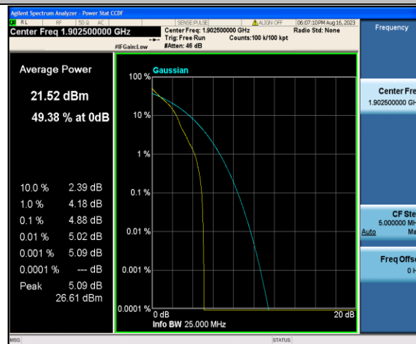
Band2-15MHz-QPSK-19125-1RB#0-PASS
