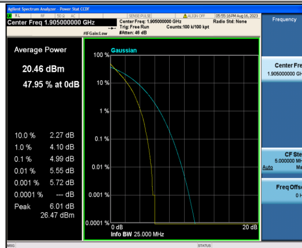
Band2-10MHz-QPSK-19150-50RB#0-PASS
