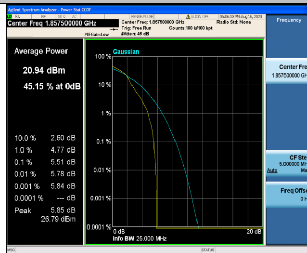
Band2-15MHz-16QAM-18675-1RB#0-PASS
