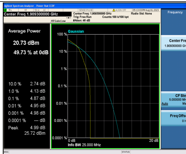
Band2-1.4MHz-16QAM-19193-1RB#0-PASS
