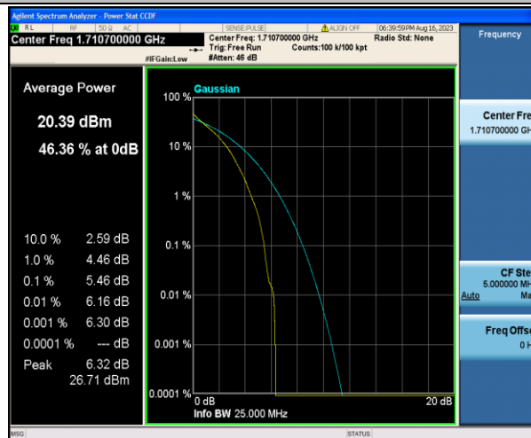
Band4-1.4MHz-QPSK-19957-6RB#0-PASS
