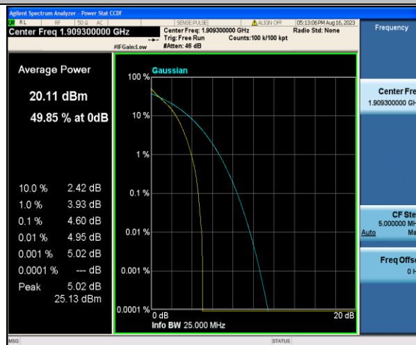
Band2-1.4MHz-QPSK-19193-6RB#0-PASS
