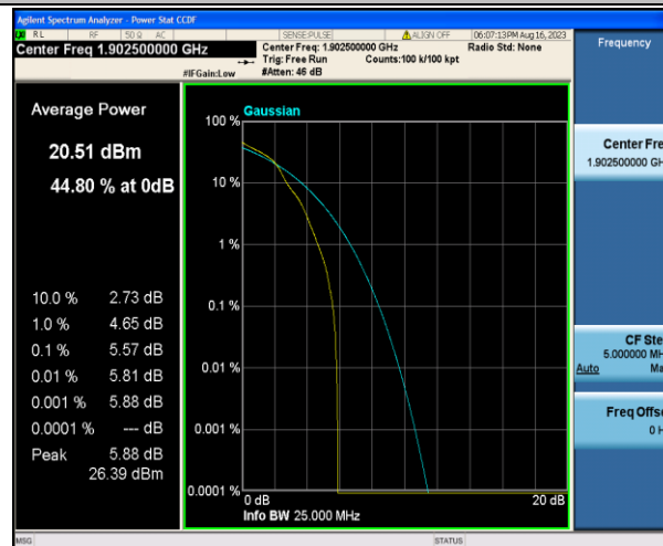
Band2-15MHz-16QAM-19125-1RB#0-PASS
