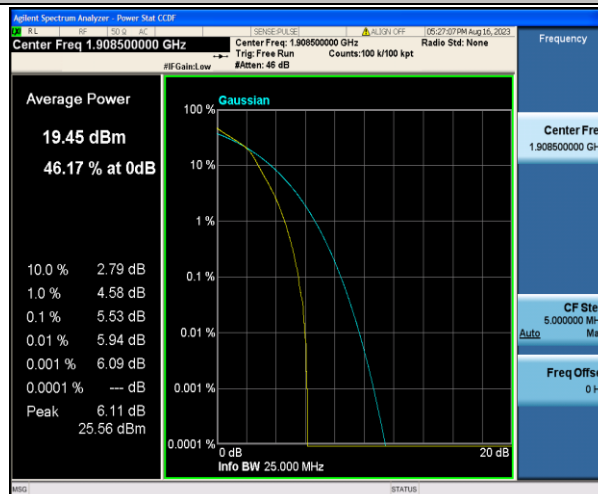
Band2-3MHz-16QAM-19185-15RB#0-PASS
