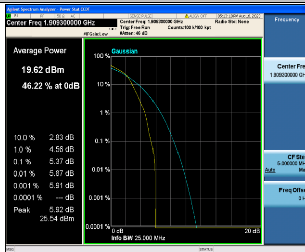
Band2-1.4MHz-16QAM-19193-6RB#0-PASS
