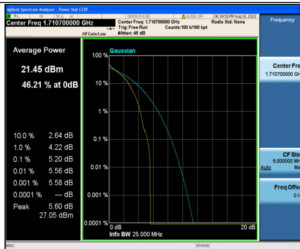
Band4-1.4MHz-QPSK-19957-1RB#0-PASS
