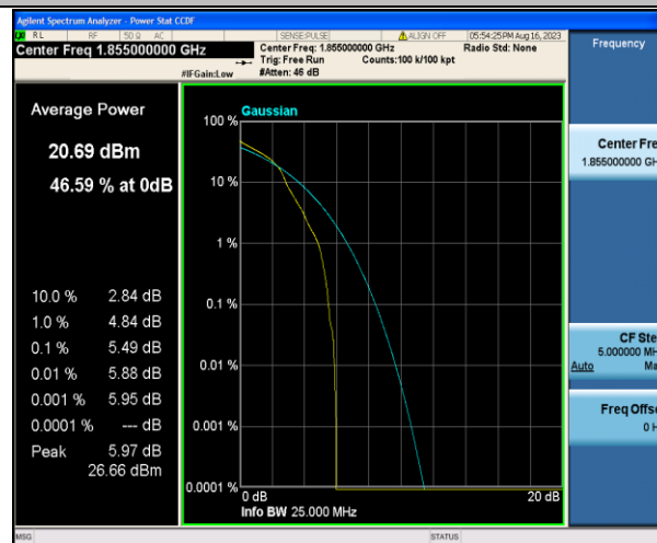
Band2-10MHz-16QAM-18650-1RB#0-PASS
