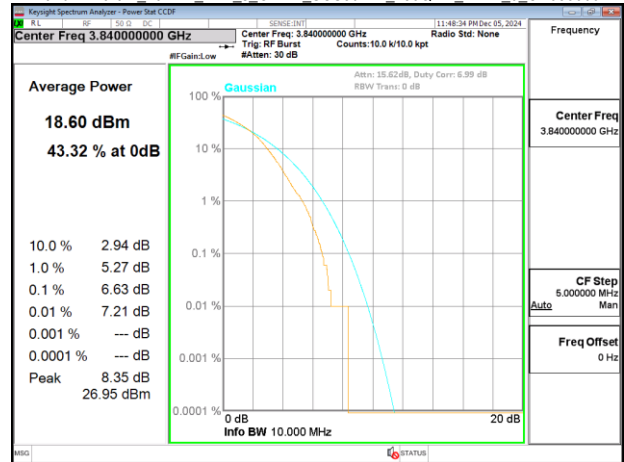
Band77-Part27_10MHz_DFT_s_OFDM_SCS30kHz_256QAM_RB24_0_CH656000
