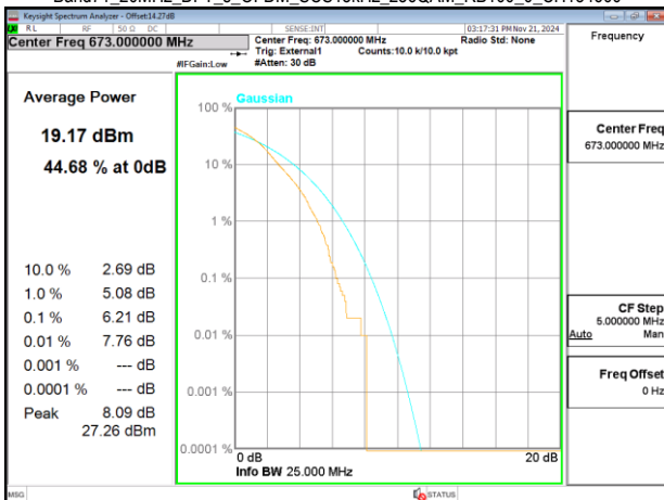
Band71_20MHz_DFT_s_OFDM_SCS15kHz_256QAM_RB100_0_CH134600
