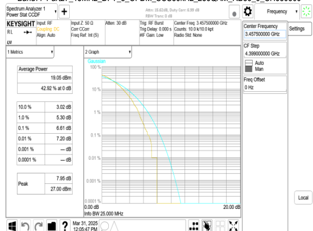
Band77-Part27_15MHz_DFT_s_OFDM_SCS30kHz_256QAM_RB36_0_CH630500
