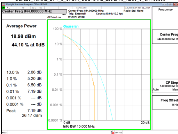
Band26_10MHz_DFT_s_OFDM_SCS15kHz_256QAM_RB50_0_CH168800
