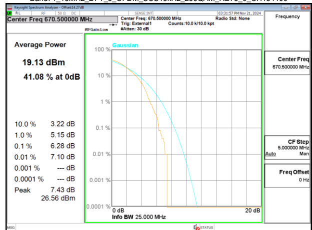
Band71_15MHz_DFT_s_OFDM_SCS15kHz_256QAM_RB75_0_CH134100
