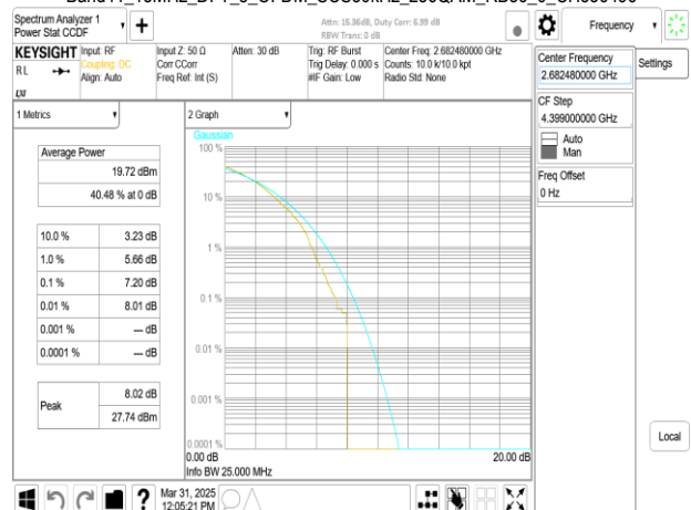
Band41_15MHz_DFT_s_OFDM_SCS30kHz_256QAM_RB36_0_CH536496
