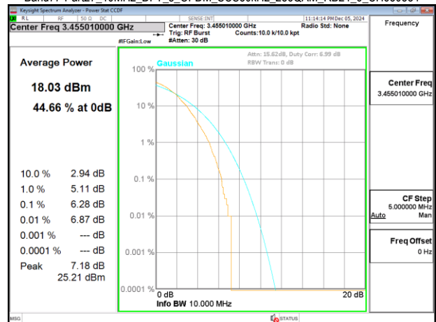
Band77-Part27_10MHz_DFT_s_OFDM_SCS30kHz_256QAM_RB24_0_CH630334
