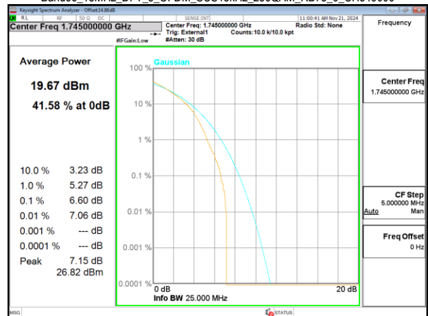
Band66_15MHz_DFT_s_OFDM_SCS15kHz_256QAM_RB75_0_CH349000
