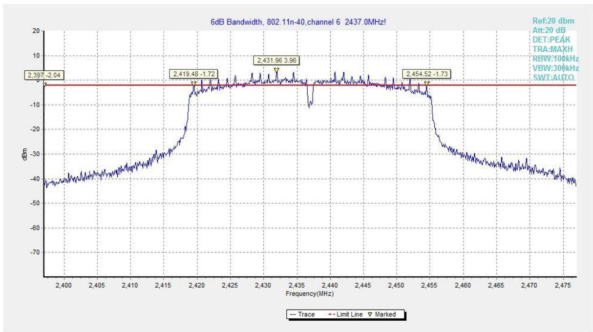
Fig.B.4.11 Occupied 6dB Bandwidth (802.11n-HT40, Ch 6)
