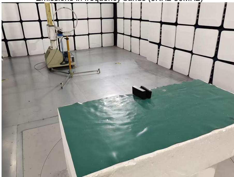
Emissions in frequency bands (9KHz-30MHz)
