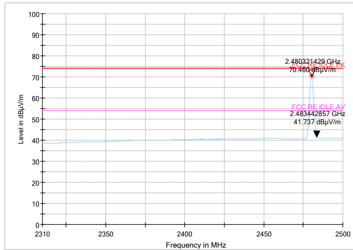
Fig 10 Radiated emission (Power): \pi/4 DQPSK, high channel
