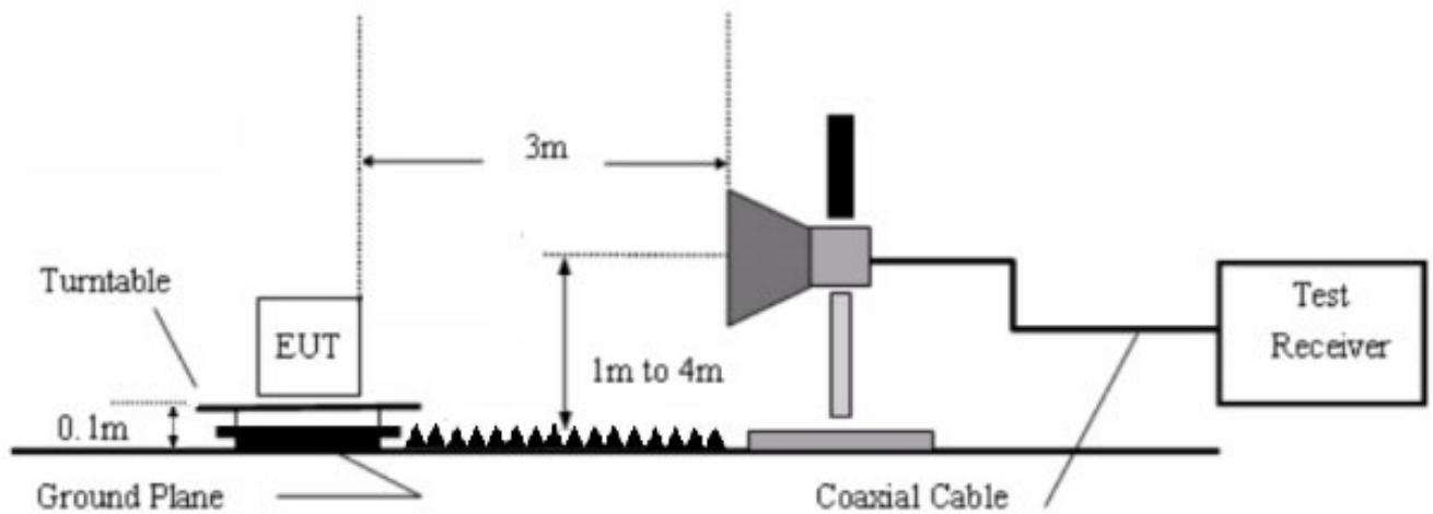
Figure 3. Above 1 GHz
