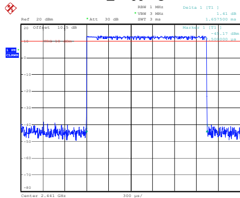
2DH3_Hopping 1.658ms
