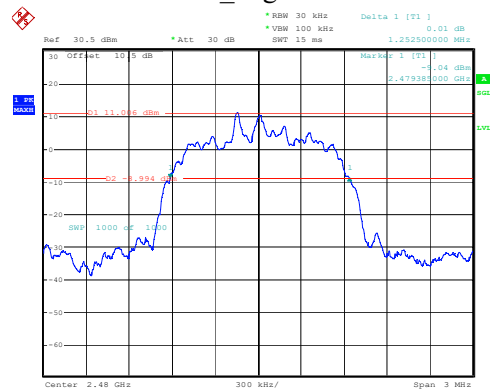
2DH1_High 1.252MHz
