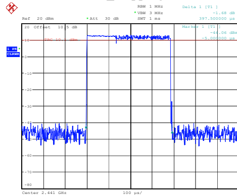
2DH1_Hopping 0.398ms
