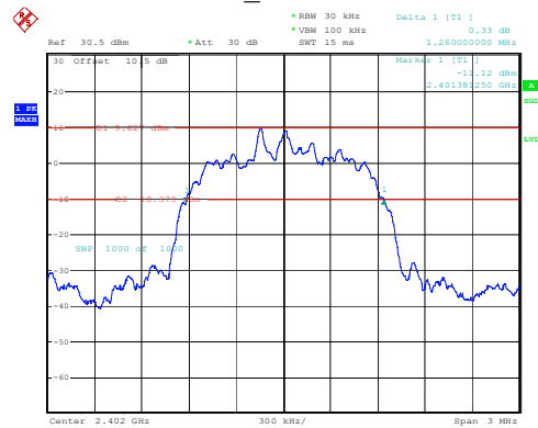
2DH1_Low 1.260MHz
