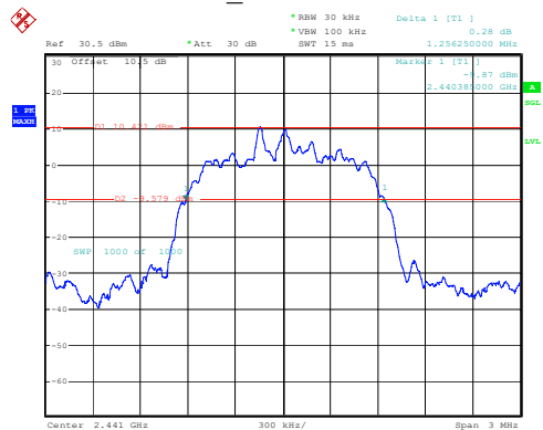
2DH1_Middle 1.256MHz
