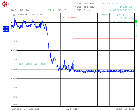
3DH1_Hopping_Upper
