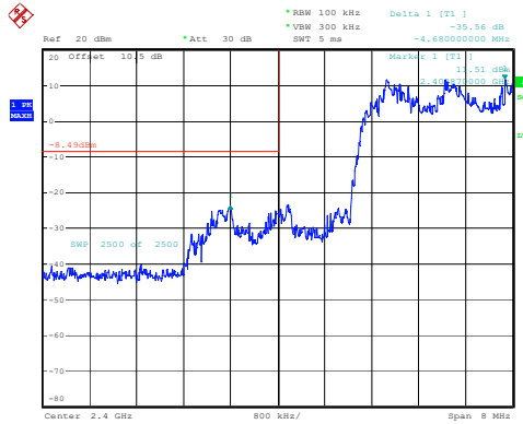
3DH1_Hopping_Lower
