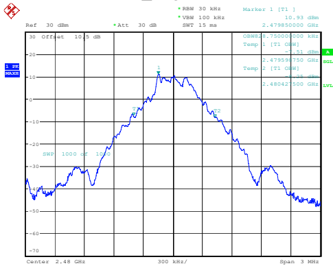
DH1_High 0.829MHz
