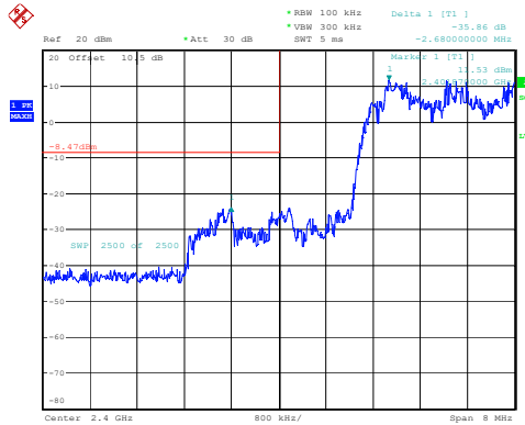
2DH1_Hopping_Lower
