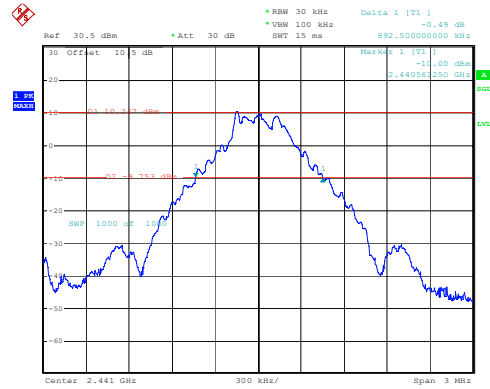
DH1_Middle 0.893MHz
