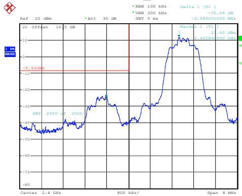
3DH1_Low
