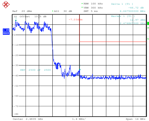
2DH1_Hopping_Upper
