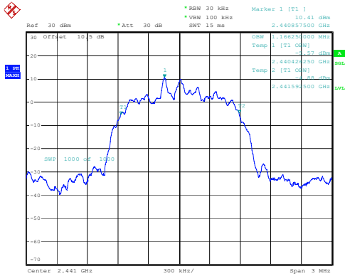
2DH1_Middle 1.166MHz
