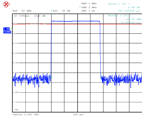
DH1_Hopping 0.388ms
