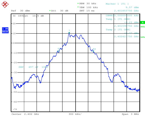
DH1_Low 0.825MHz
