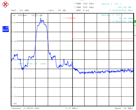
3DH1_High
