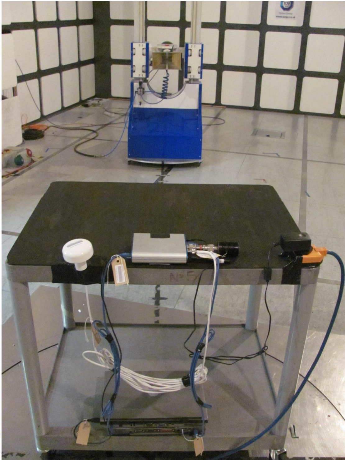
Figure 1 – EUT on back 1G-2G
