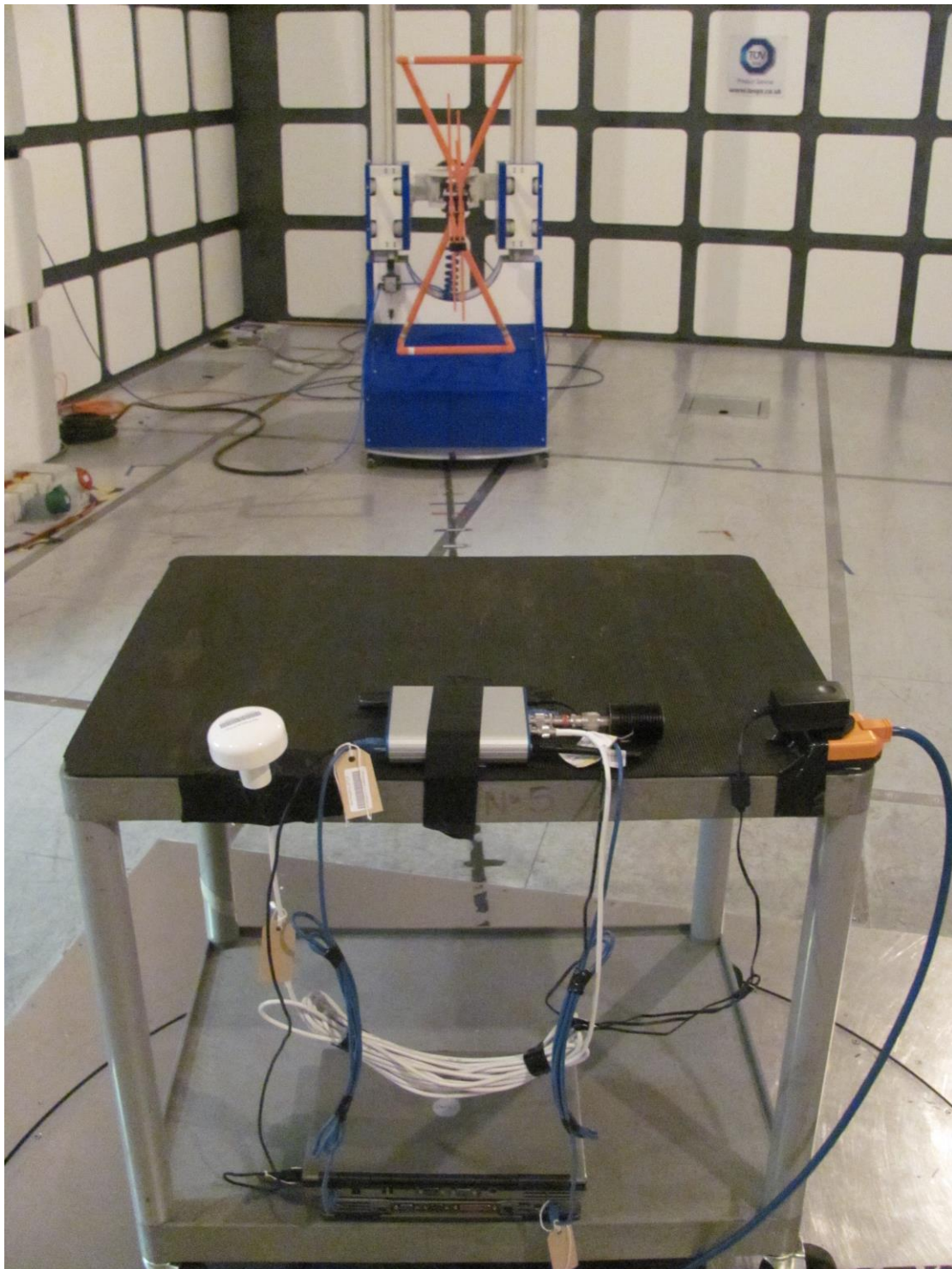
Figure 2 – EUT on back 30M-1G
