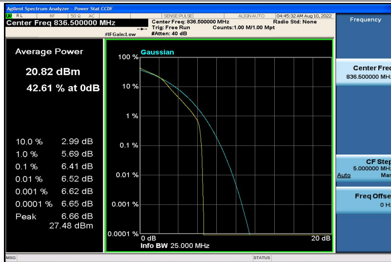
Band5-10MHz-16QAM-20525-6RB#0
