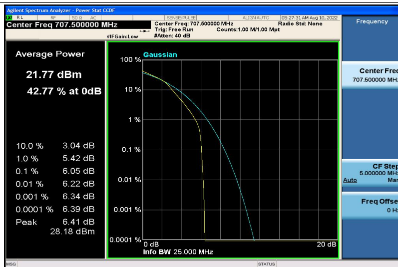
Band12-5MHz-16QAM-23095-6RB#0
