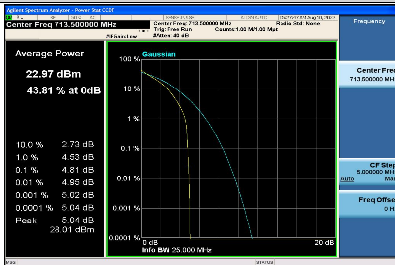
Band12-5MHz-QPSK-23155-6RB#0
