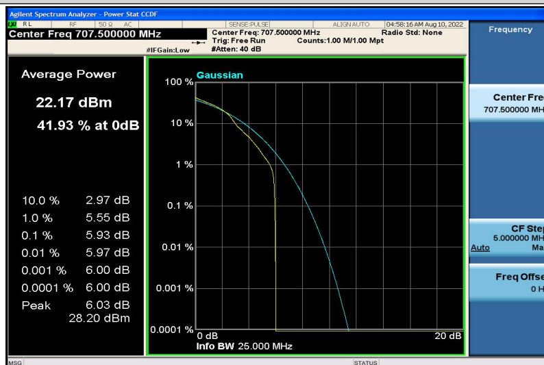
Band12-1.4MHz-16QAM-23095-1RB#0
