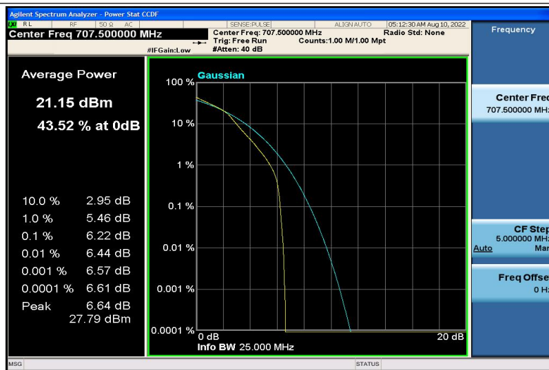
Band12-3MHz-16QAM-23095-6RB#0
