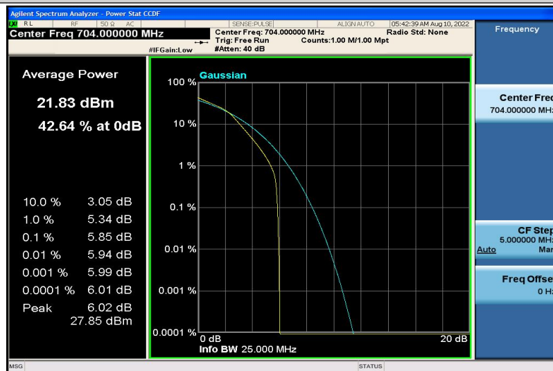
Band12-10MHz-16QAM-23060-6RB#0
