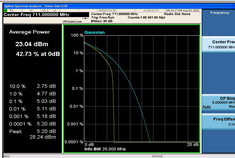
Band12-10MHz-QPSK-23130-6RB#0
