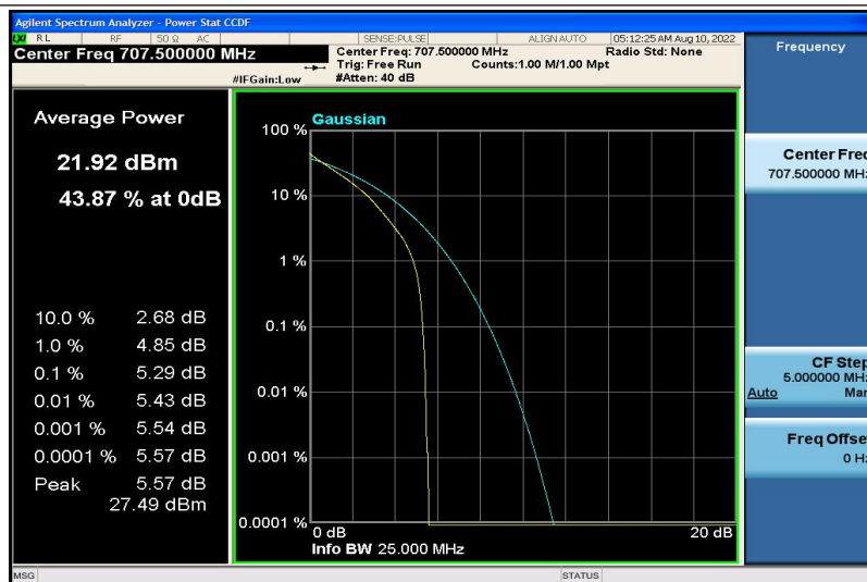
Band12-3MHz-QPSK-23095-6RB#0
