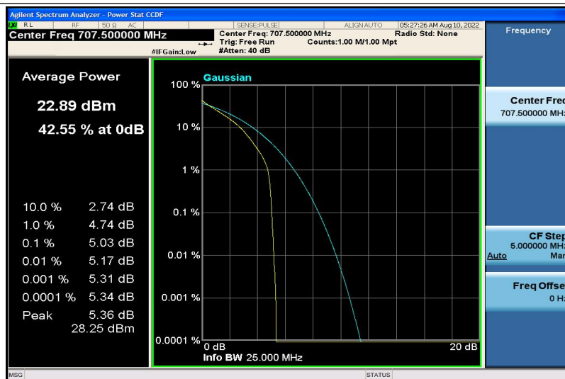
Band12-5MHz-QPSK-23095-6RB#0
