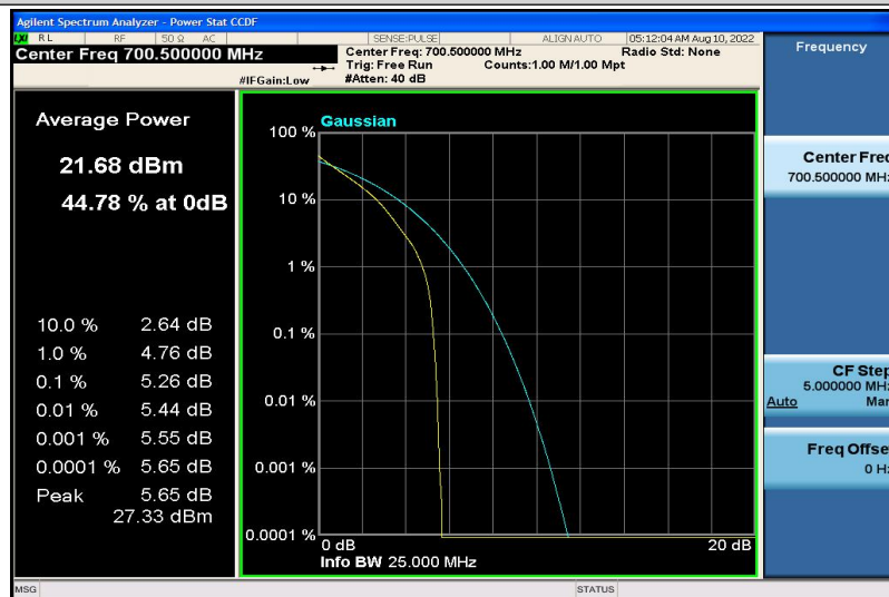
Band12-3MHz-QPSK-23025-6RB#0
