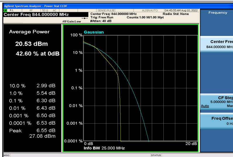
Band5-10MHz-16QAM-20600-6RB#0
