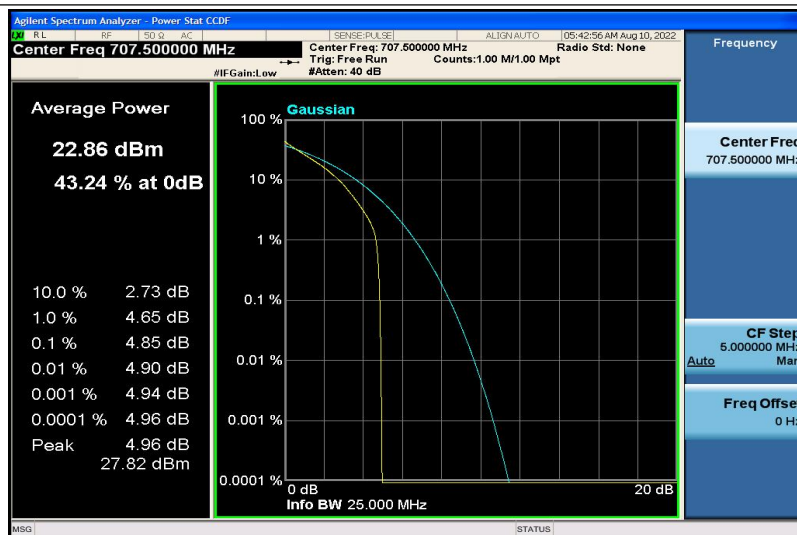
Band12-10MHz-QPSK-23095-6RB#0
