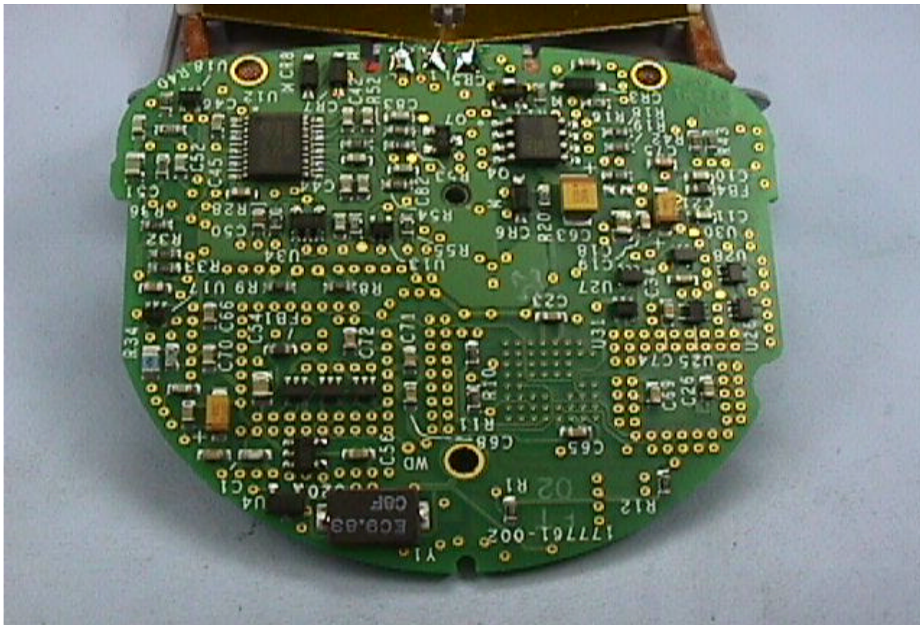
2490A Telemetry Module Circuit Board, Bottom Side
