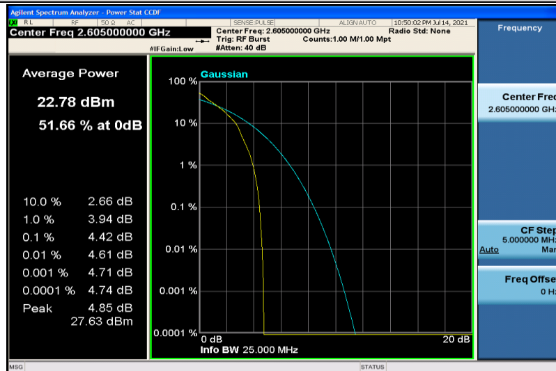
Band41-5MHz-QPSK-40740-1RB#0
