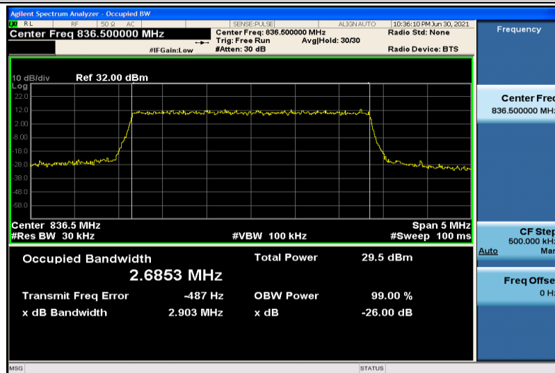
Band5-3MHz-QPSK-20525-15RB#0-2.6853
