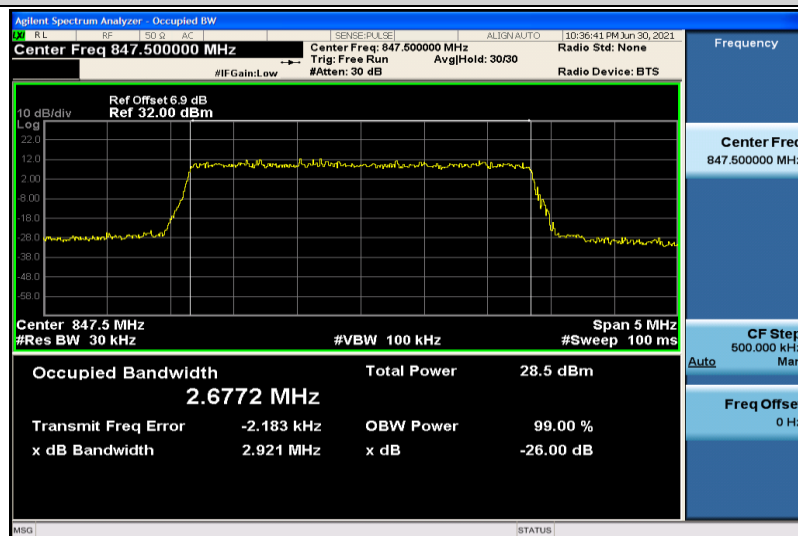
Band5-3MHz-16QAM-20635-15RB#0-2.6772
