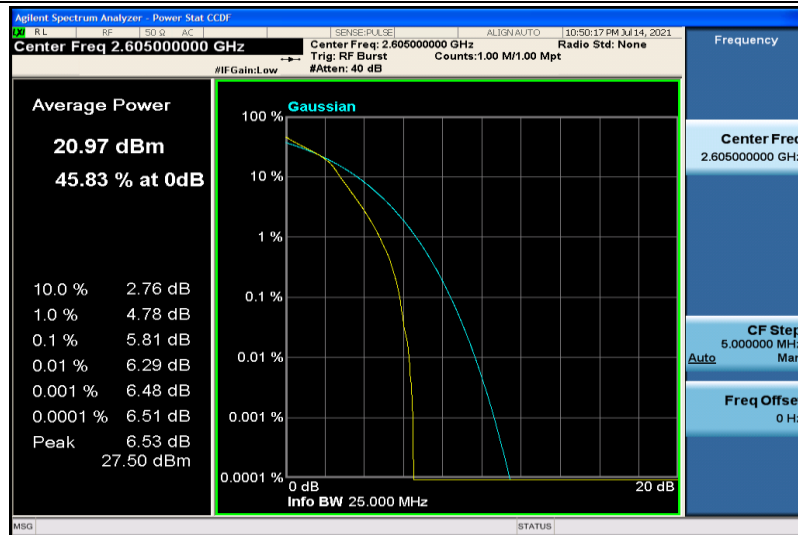
Band41-5MHz-16QAM-40740-25RB#0
