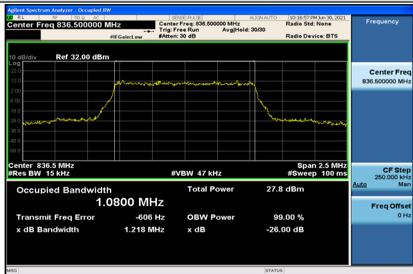
Band5-1.4MHz-16QAM-20525-6RB#0-1.0800
