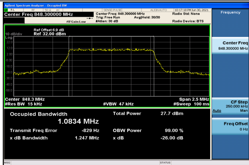
Band5-1.4MHz-16QAM-20643-6RB#0-1.0834
