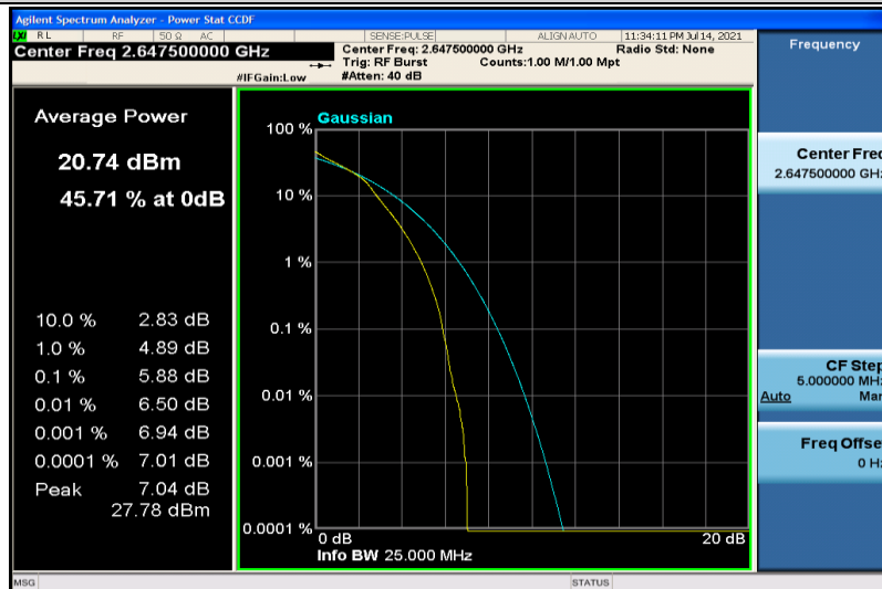
Band41-15MHz-16QAM-41165-75RB#0
