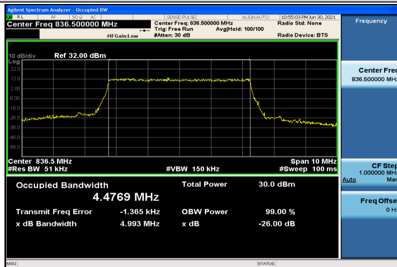
Band5-5MHz-QPSK-20525-25RB#0-4.4769
