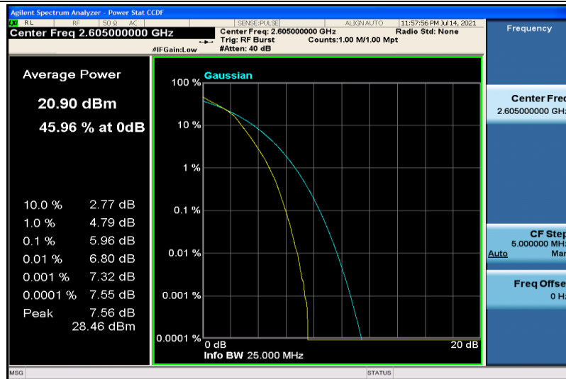
Band41-20MHz-16QAM-40740-100RB#0
