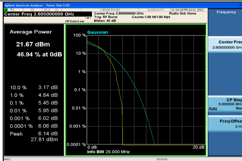
Band41-10MHz-16QAM-40740-1RB#0
