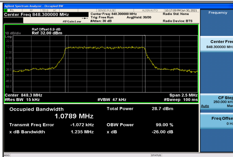
Band5-1.4MHz-QPSK-20643-6RB#0-1.0789
