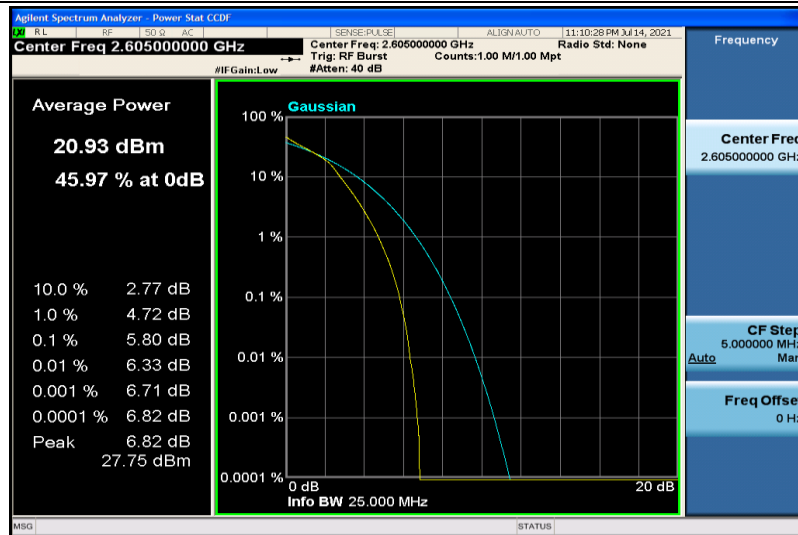
Band41-10MHz-16QAM-40740-50RB#0
