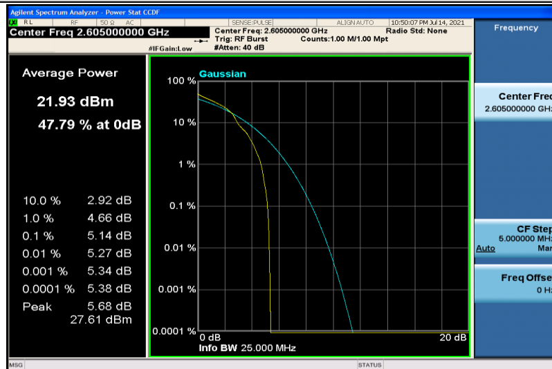
Band41-5MHz-16QAM-40740-1RB#0
