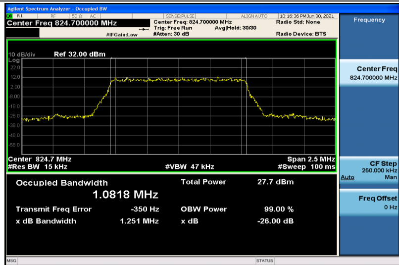
Band5-1.4MHz-16QAM-20407-6RB#0-1.0818
