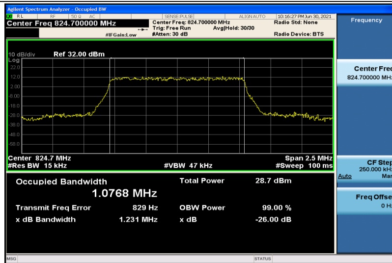
Band5-1.4MHz-QPSK-20407-6RB#0-1.0768
