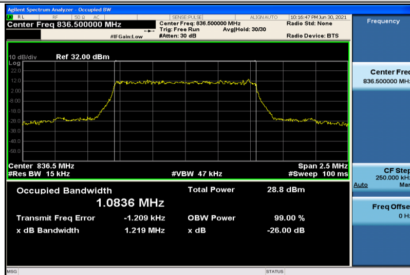
Band5-1.4MHz-QPSK-20525-6RB#0-1.0836
