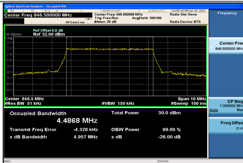
Band5-5MHz-QPSK-20625-25RB#0-4.4868
