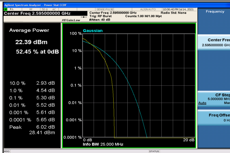
Band38-15MHz-QPSK-38000-1RB#0
