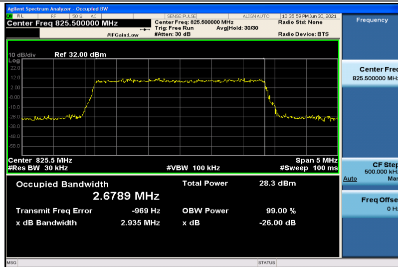
Band5-3MHz-16QAM-20415-15RB#0-2.6789
