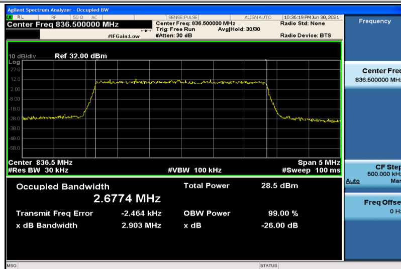
Band5-3MHz-16QAM-20525-15RB#0-2.6774
