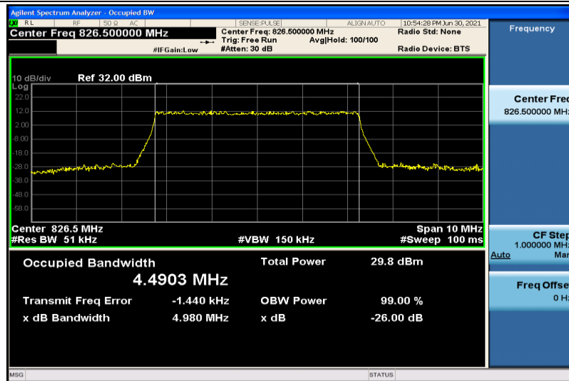
Band5-5MHz-QPSK-20425-25RB#0-4.4903
