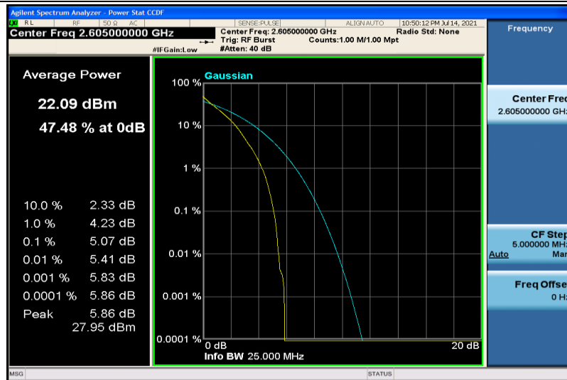
Band41-5MHz-QPSK-40740-25RB#0
