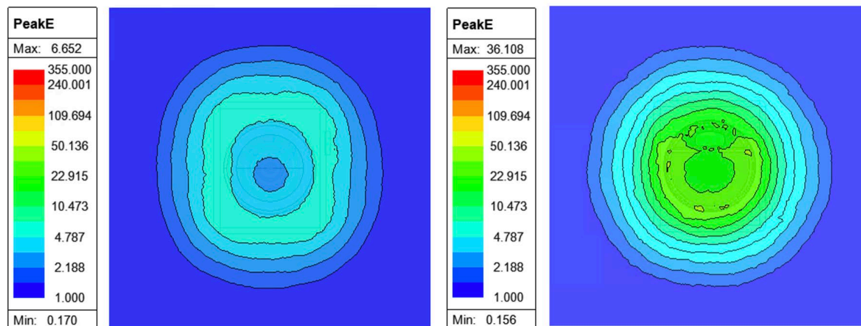
Figure 15: E-field on the two planes from WPT Charger WPT simulation model at 1.778 MHz
