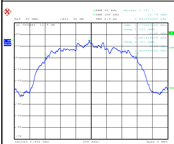
99% Occupied Bandwidth Plot on Channel 00
