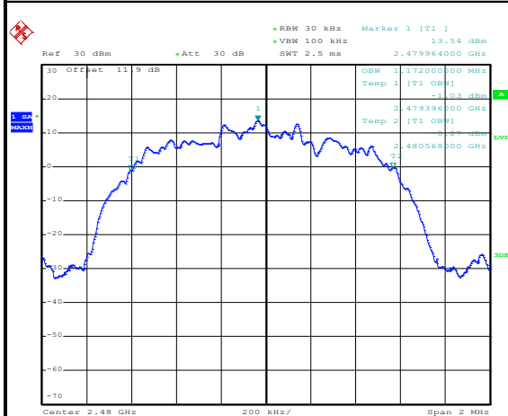
99% Occupied Bandwidth Plot on Channel 78
