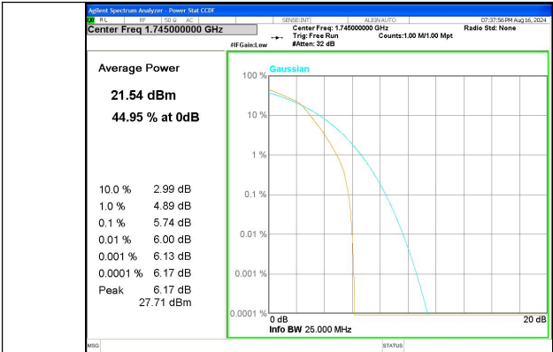
Band 66 1.4MHz/1745.0/Mid 16QAM 6@0
