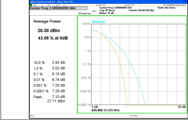
Band 38 20MHz/2580.0/Low 16QAM 100@0
