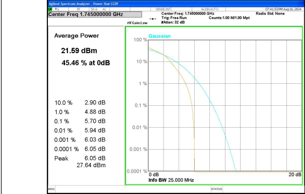
Band 66 5MHz/1745.0/Mid 16QAM 25@0
