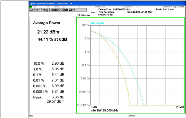
Band 25 20MHz/1860.0/Low 16QAM 100@0
