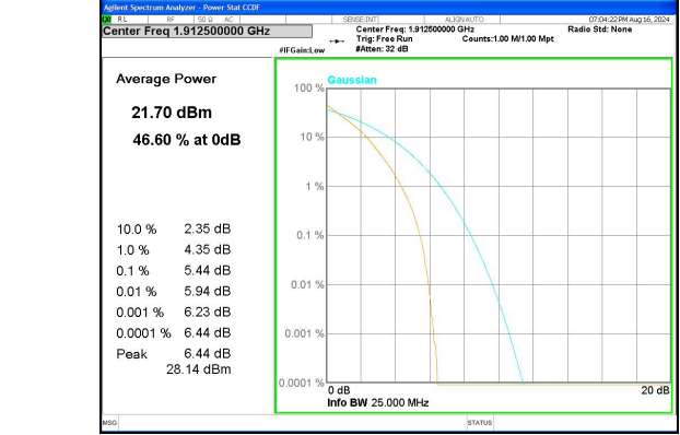
Band 25 5MHz/1912.5/High QPSK 25@@
