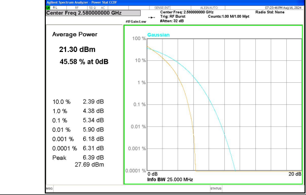
Band 38 20MHz/2580.0/Low QPSK 100@0
