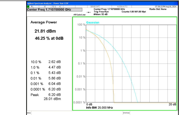
Band 66 1.4MHz/1710.7/Low QPSK 6@0
