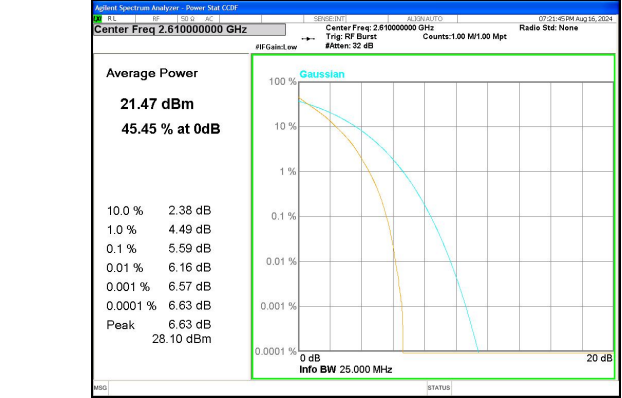
Band 38 20MHz/2610.0/High QPSK 100@0
