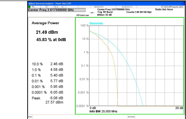
Band 38 5MHz/2617.5/High QPSK 25@0
