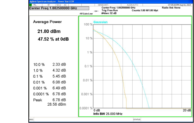
Band 25 5MHz/1882.5/Mid QPSK 25@@
