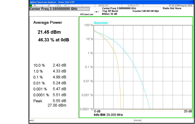
Band 38 5MHz/2595.0/Mid QPSK 25@0
