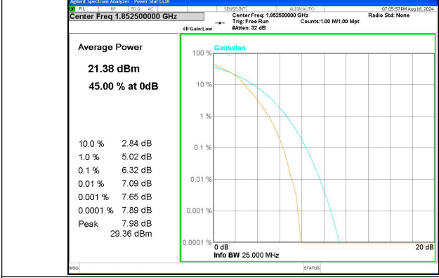
Band 25 5MHz/1852.5/Low 16QAM 25@@
