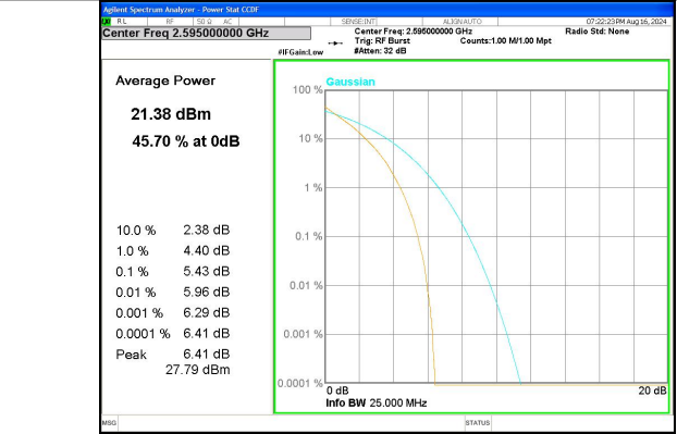
Band 38 20MHz/2595.0/Mid QPSK 100@0
