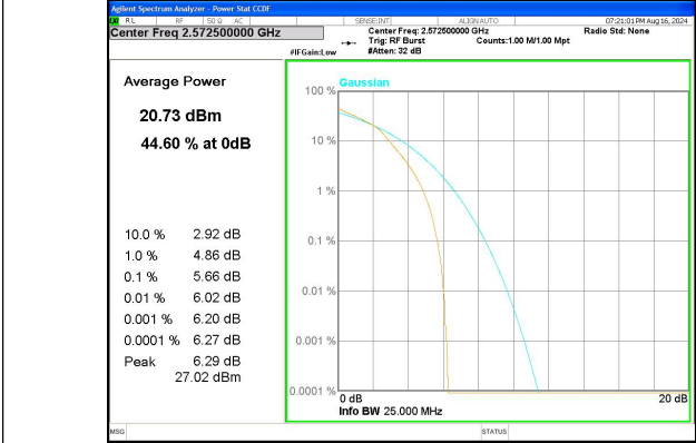
Band 38 5MHz/2572.5/Low 16QAM 25@0
