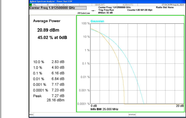
Band 25 5MHz/1912.5/High 16QAM 25@@
