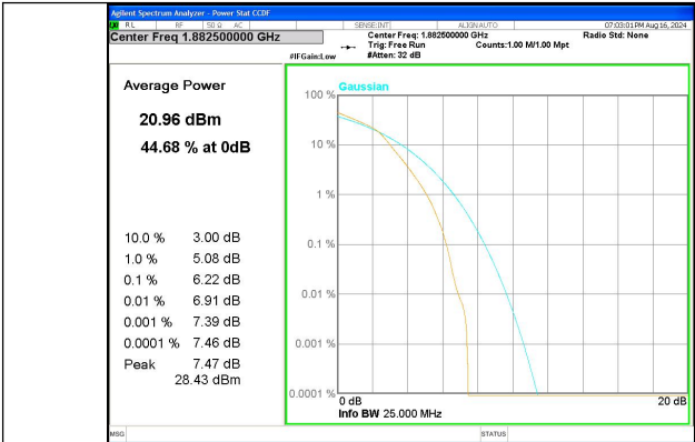
Band 25 1.4MHz/1882.5/Mid 16QAM 6@@
