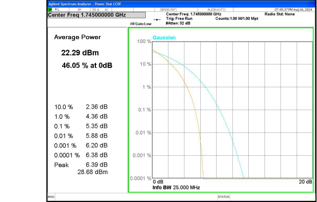
Band 66 20MHz/1745.0/Mid QPSK 100@0
