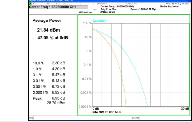
Band 25 20MHz/1882.5/Mid QPSK 100@@
