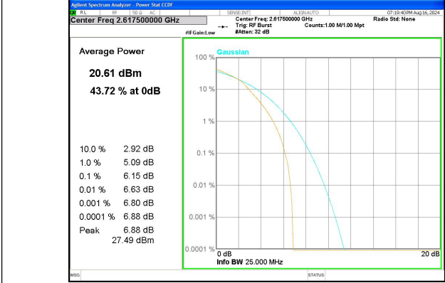
Band 38 5MHz/2617.5/High 16QAM 25@0
