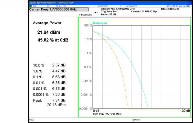
Band 66 20MHz/1770.0/High QPSK 100@0
