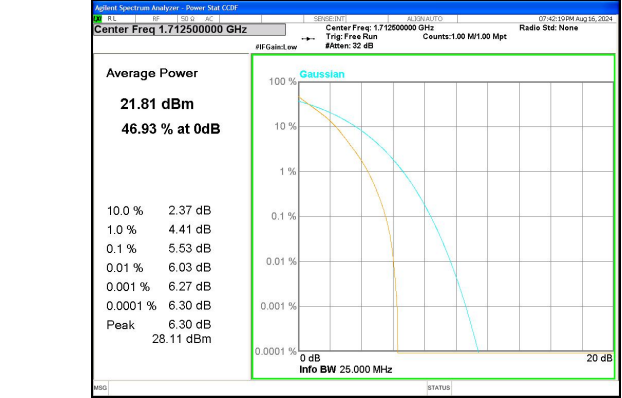
Band 66 5MHz/1712.5/Low QPSK 25@0
