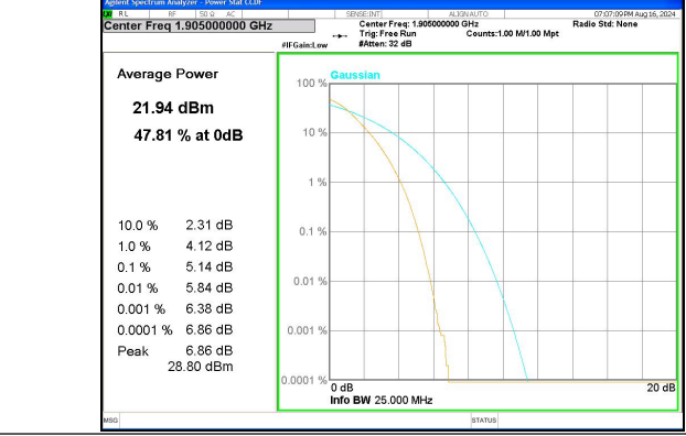
Band 25 20MHz/1905.0/High QPSK 100@@
