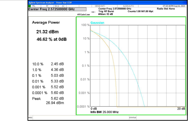
Band 38 5MHz/2572.5/Low QPSK 25@0
