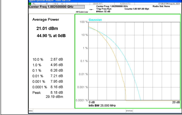
Band 25 20MHz/1882.5/Mid 16QAM 100@@
