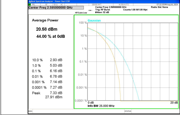
Band 38 20MHz/2595.0/Mid 16QAM 100@0
