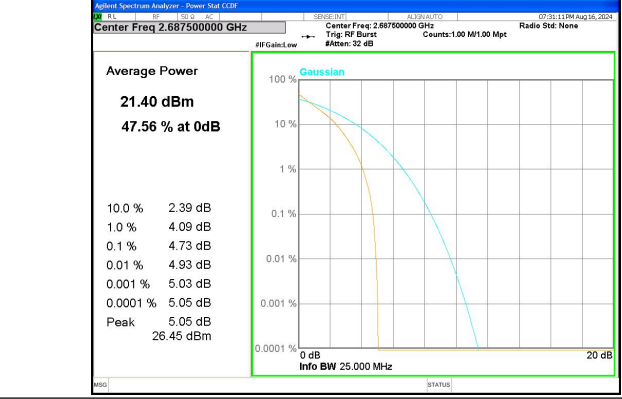
Band 41 5MHz/2687.5/High QPSK 25@0
