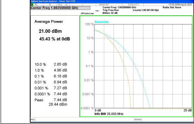
Band 25 5MHz/1882.5/Mid 16QAM 25@@
