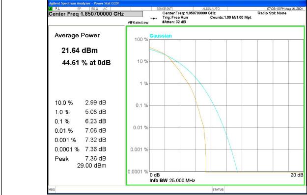
Band 25 1.4MHz/1850.7/Low 16QAM 6@@
