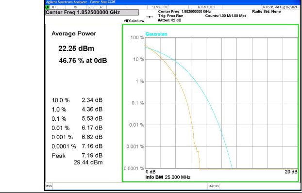
Band 25 5MHz/1852.5/Low QPSK 25@@
