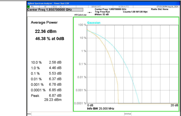
Band 25 1.4MHz/1850.7/Low QPSK 6@@
