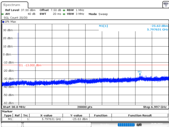
1.4MHz_Low_QPSK_1@0 -25.63dBm
