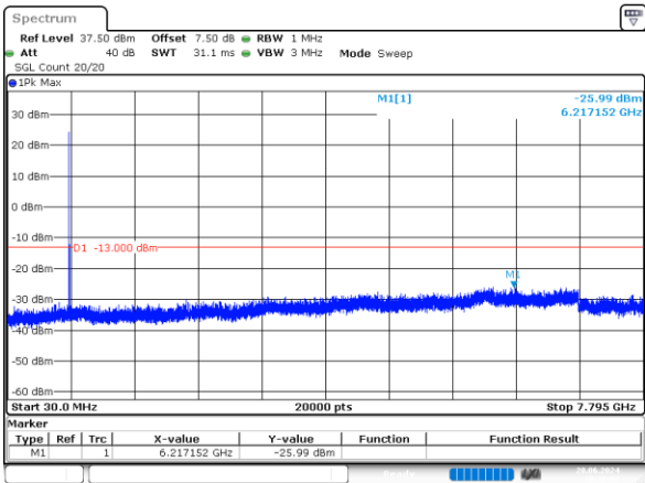
5MHz_Low_QPSK_1@0 -25.99dBm
