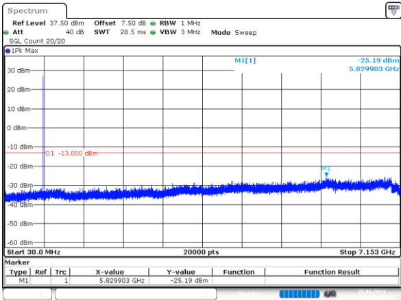
1.4MHz_High_QPSK_1@0 -25.19dBm
