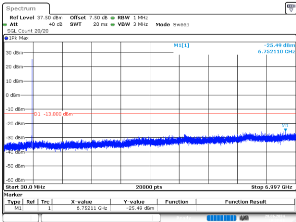
1.4MHz_Low_QPSK_6@0 -25.49dBm
