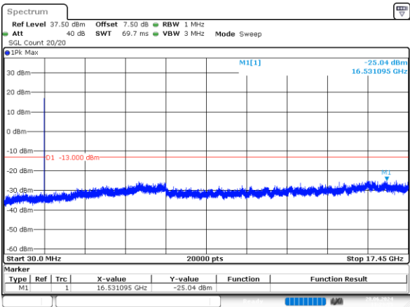
1.4MHz_Middle_QPSK_6@0 -25.04dBm
