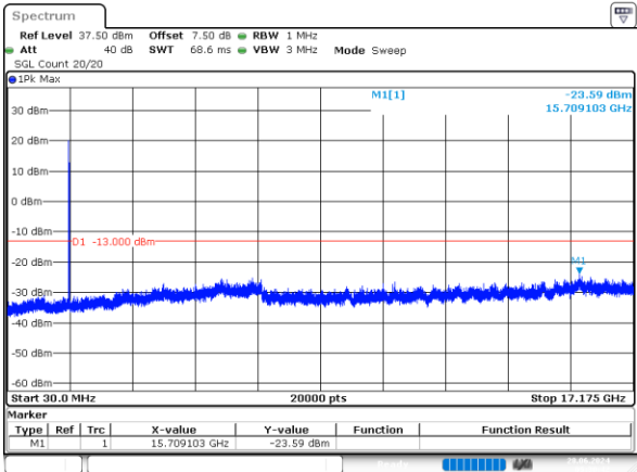
15MHz_Low_QPSK_1@0 -23.59dBm
