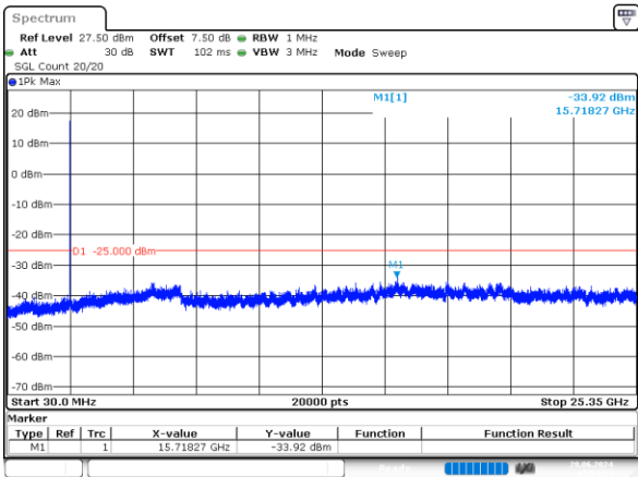
5MHz_Middle_QPSK_1@0 -33.92dBm
