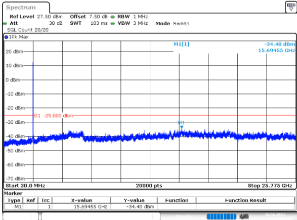
15MHz_Low_QPSK_75@0 -34.40dBm
