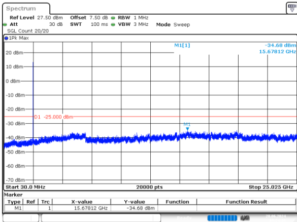
5MHz_Low_QPSK_25@0 -34.68dBm
