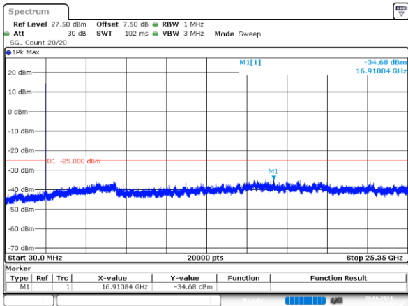
5MHz_Middle_QPSK_25@0 -34.68dBm
