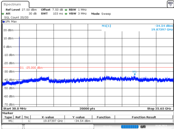
10MHz_High_QPSK_50@0 -34.54dBm
