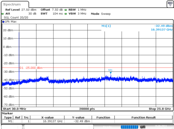
20MHz_Low_QPSK_1@0 -32.49dBm
