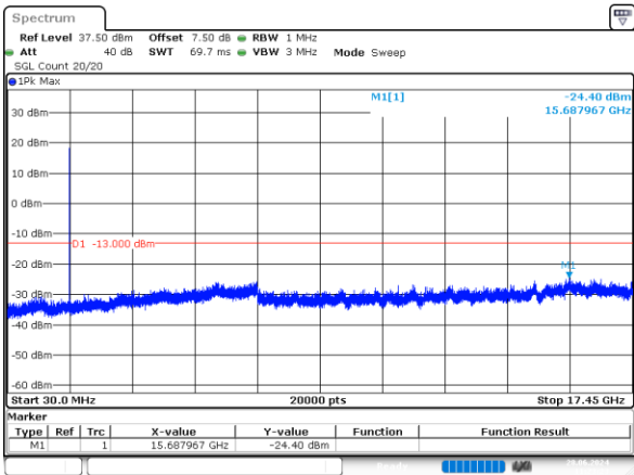
1.4MHz_Middle_QPSK_1@0 -24.40dBm
