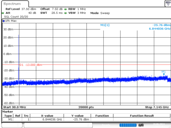
3MHz_High_QPSK_15@0 -25.76dBm
