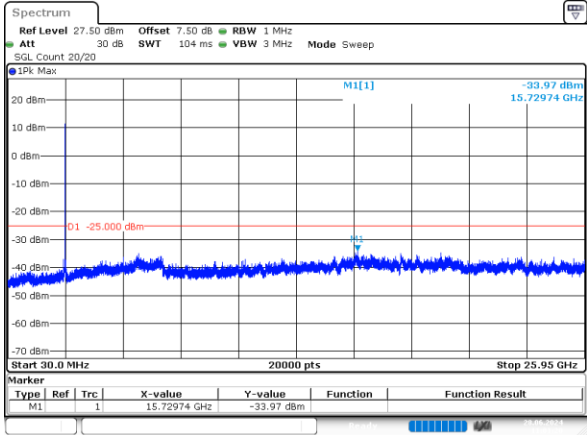
15MHz_Middle_QPSK_75@0 -33.97dBm
