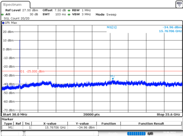
20MHz_High_QPSK_100@0 -34.96dBm
