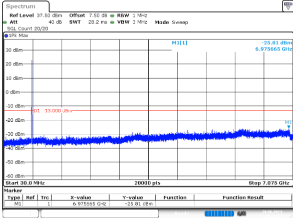
3MHz_Middle_QPSK_15@0 -25.81dBm
