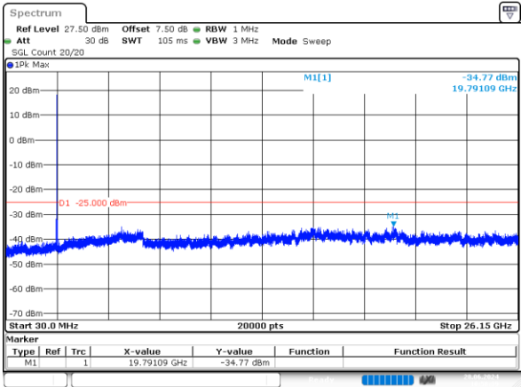
10MHz_High_QPSK_1@0 -34.77dBm
