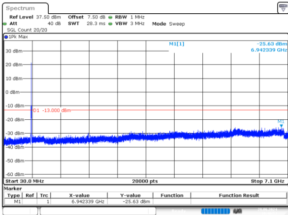
5MHz_Middle_QPSK_25@0 -25.63dBm
