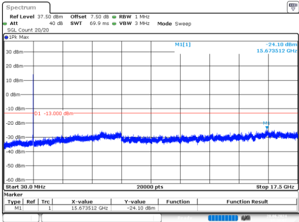
10MHz_High_QPSK_50@0 -24.10dBm
