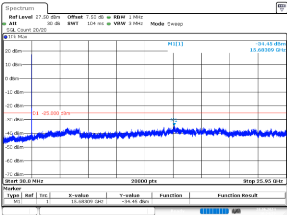
5MHz_Middle_QPSK_1@0 -34.45dBm
