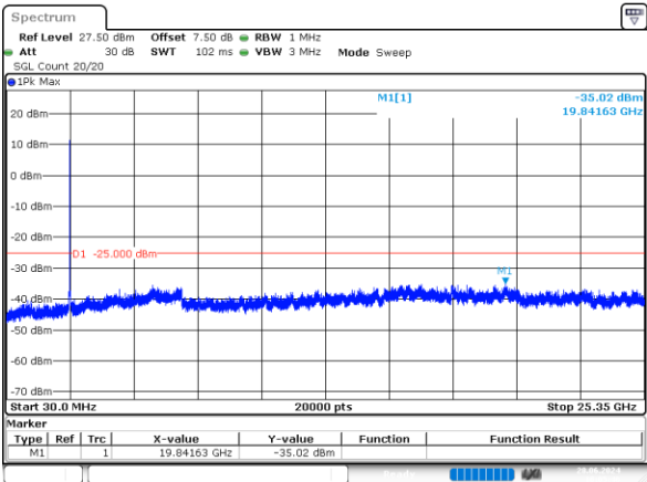
20MHz_Middle_QPSK_100@0 -35.02dBm
