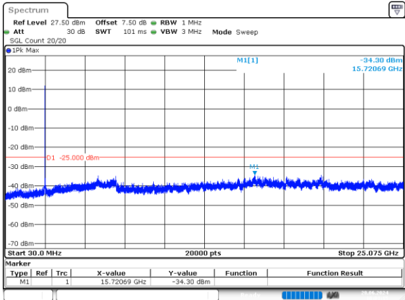
15MHz_Low_QPSK_75@0 -34.30dBm
