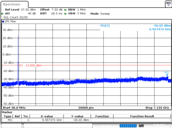
5MHz_High_QPSK_25@0 -26.02dBm
