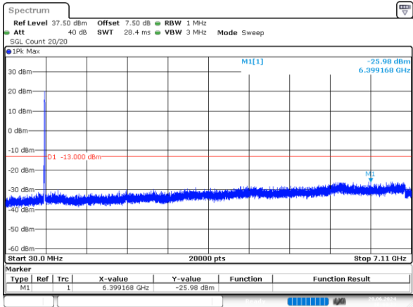
10MHz_High_QPSK_50@0 -25.98dBm
