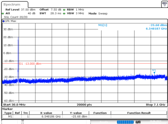
10MHz_Middle_QPSK_50@0 -25.68dBm
