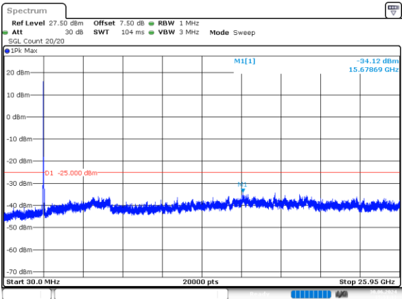
20MHz_Middle_QPSK_100@0 -34.12dBm
