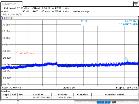
1.4MHz_Low_QPSK_6@0 -24.37dBm
