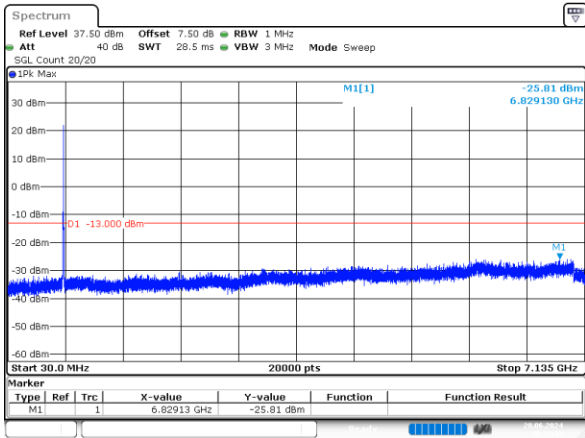
5MHz_High_QPSK_25@0 -25.81dBm
