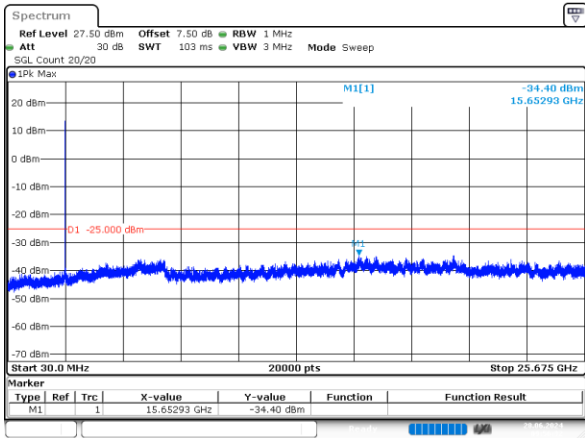
5MHz_High_QPSK_25@0 -34.40dBm
