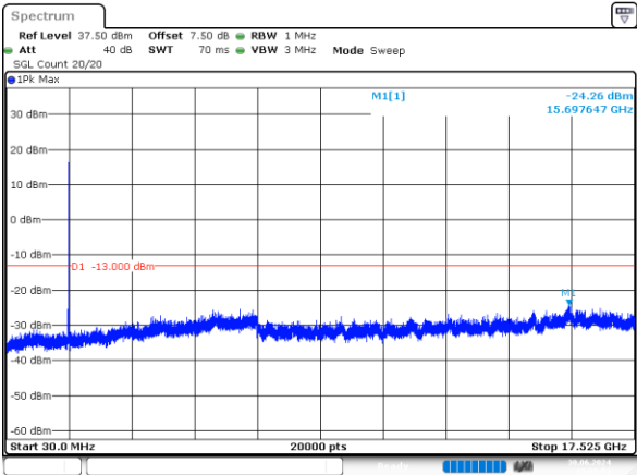
5MHz_High_QPSK_25@0 -24.26dBm
