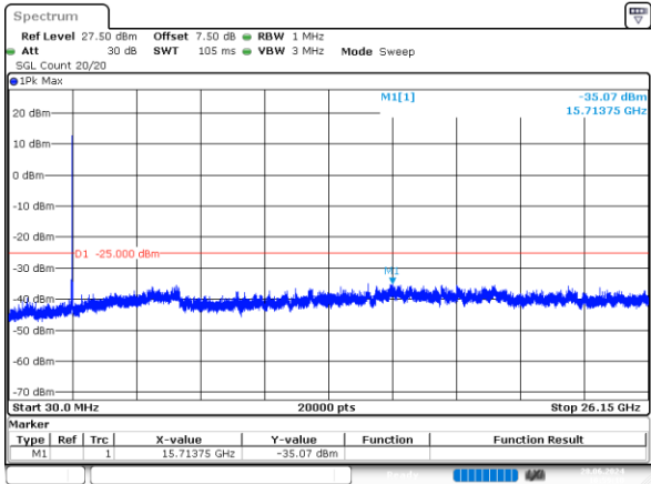
10MHz_High_QPSK_50@0 -35.07dBm
