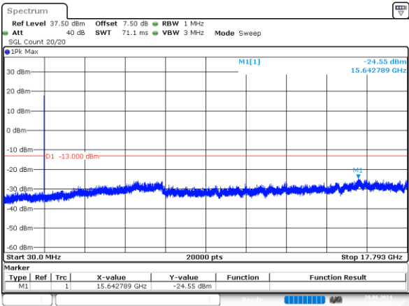
1.4MHz_High_QPSK_6@0 -24.55dBm
