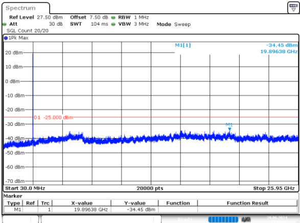
20MHz_Middle_QPSK_1@0 -34.45dBm
