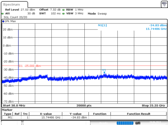
10MHz_Middle_QPSK_1@0 -34.83dBm
