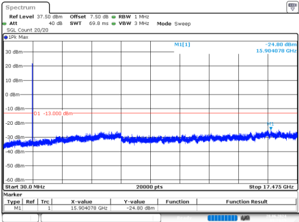
15MHz_High_QPSK_1@0 -24.80dBm
