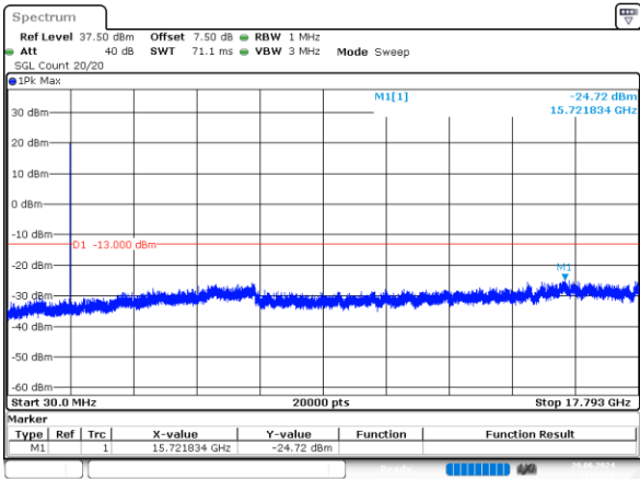
1.4MHz_High_QPSK_1@0 -24.72dBm
