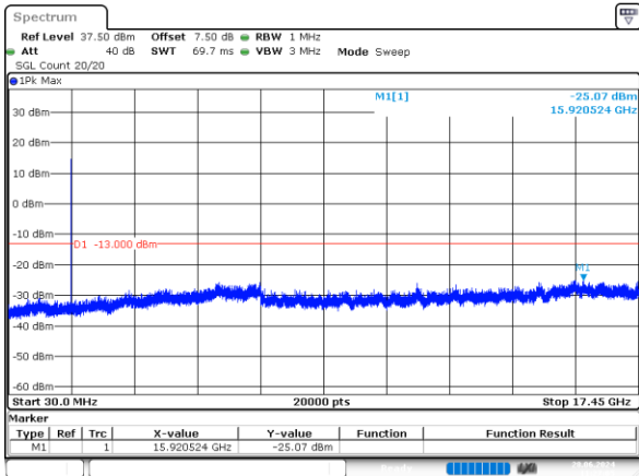
3MHz_Middle_QPSK_15@0 -25.07dBm
