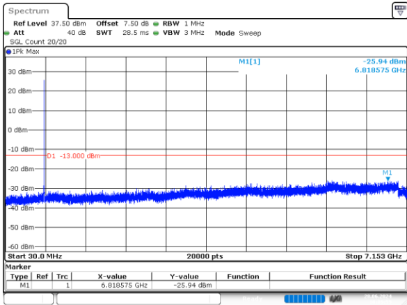
1.4MHz_High_QPSK_6@0 -25.94dBm
