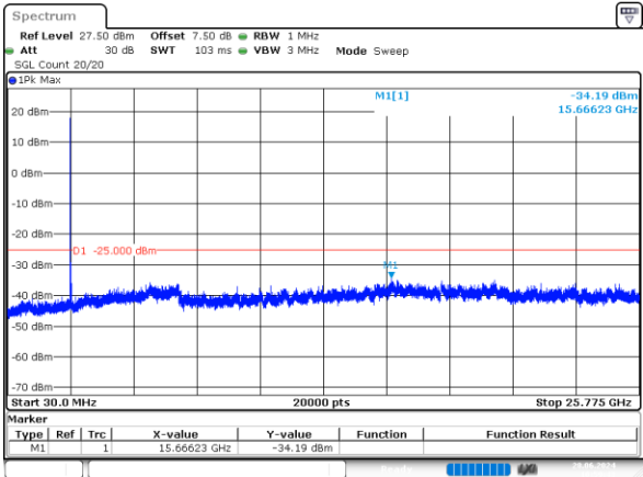
15MHz_Low_QPSK_1@0 -34.19dBm
