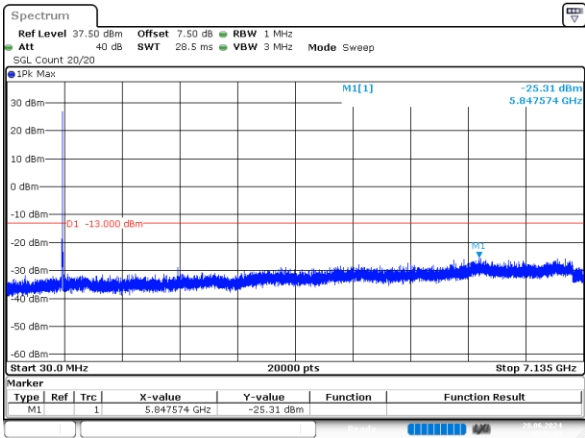
5MHz_High_QPSK_1@0 -25.31dBm
