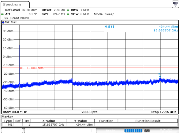
20MHz_High_QPSK_100@0 -24.44dBm
