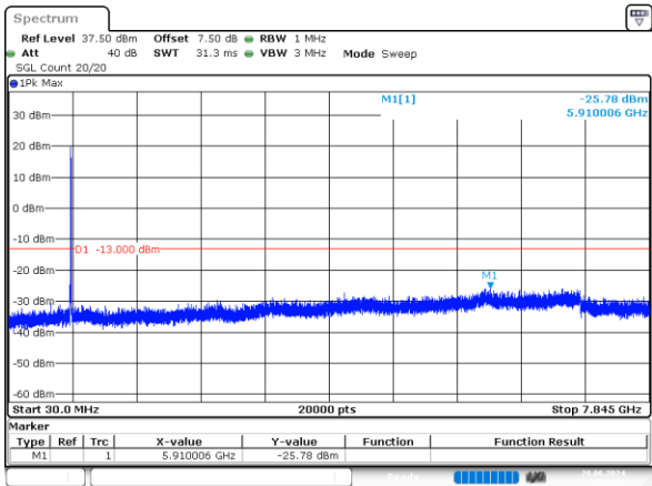
5MHz_High_QPSK_25@0 -25.78dBm
