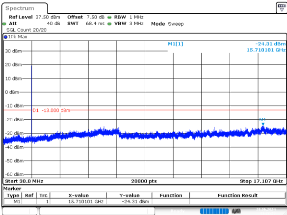
1.4MHz_Low_QPSK_1@0 -24.31dBm
