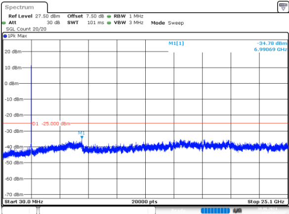
20MHz_Low_QPSK_100@0 -34.78dBm
