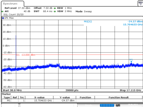
3MHz_Low_QPSK_15@0 -24.57dBm
