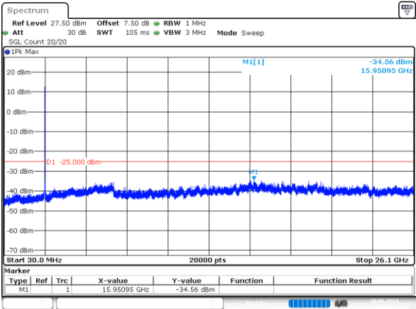
20MHz_High_QPSK_100@0 -34.56dBm
