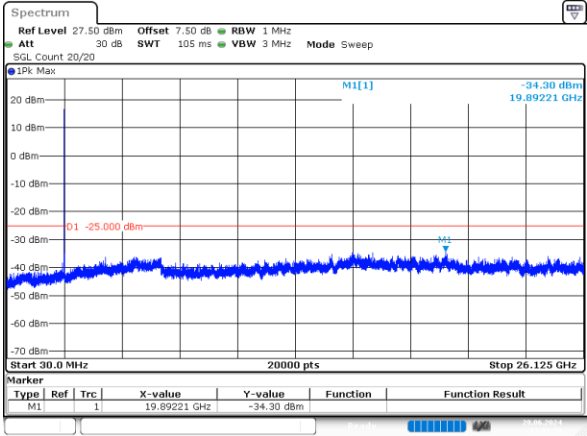
15MHz_High_QPSK_1@0 -34.30dBm
