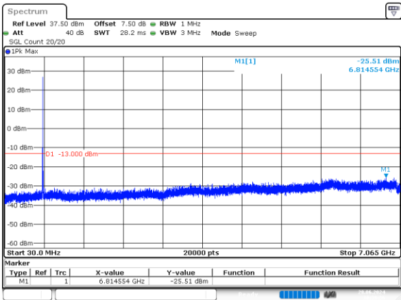
5MHz_Low_QPSK_1@0 -25.51dBm
