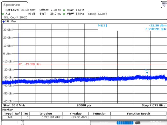
1.4MHz_Middle_QPSK_6@0 -25.38dBm
