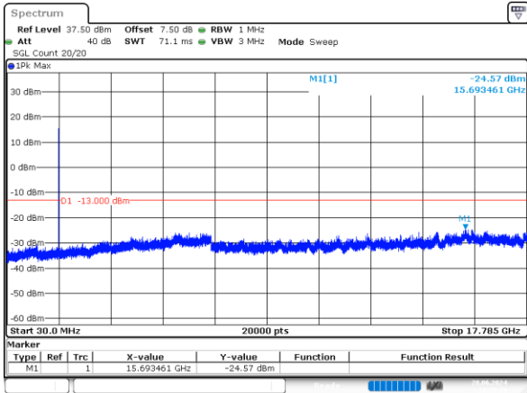
3MHz_High_QPSK_15@0 -24.57dBm
