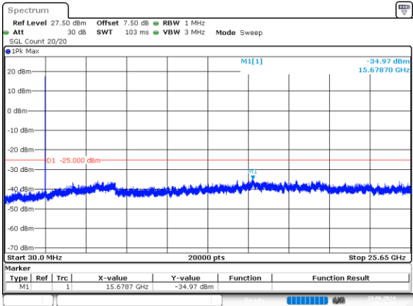
10MHz_High_QPSK_1@0 -34.97dBm
