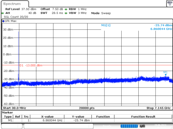
3MHz_High_QPSK_1@0 -25.74dBm
