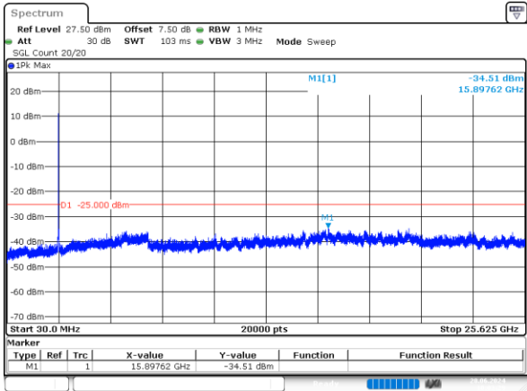
15MHz_High_QPSK_75@0 -34.51dBm
