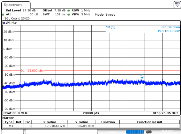
15MHz_Middle_QPSK_75@0 -35.04dBm
