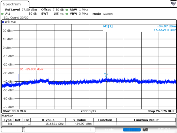
5MHz_High_QPSK_25@0 -34.97dBm
