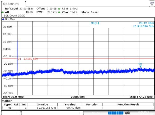
15MHz_High_QPSK_75@0 -24.42dBm
