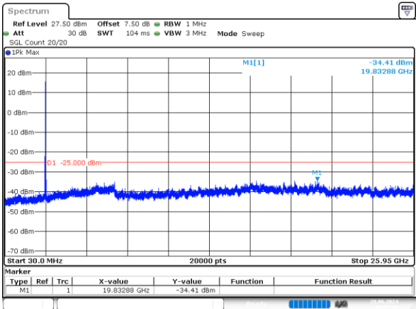
10MHz_Middle_QPSK_1@0 -34.41dBm
