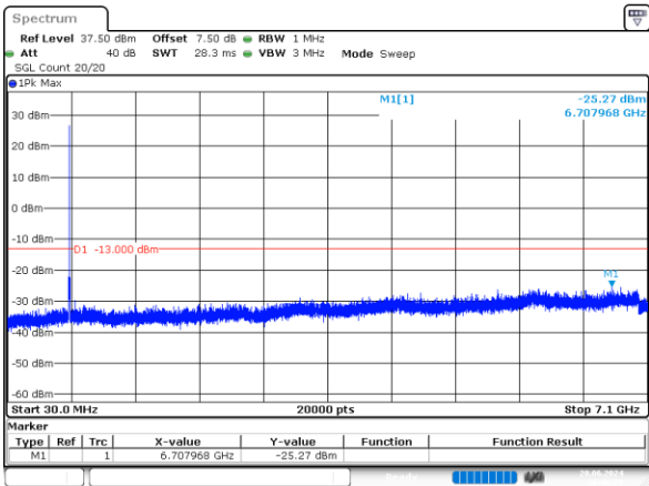
5MHz_Middle_QPSK_1@0 -25.27dBm
