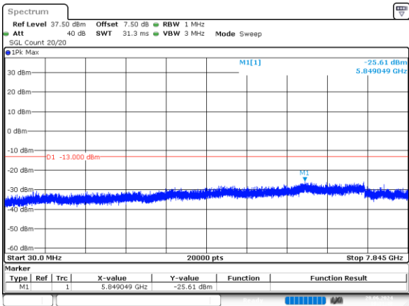
5MHz_High_QPSK_1@0 -25.61dBm
