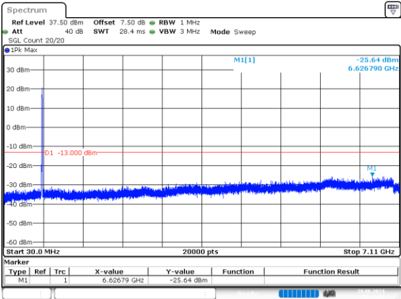
10MHz_High_QPSK_50@0 -25.64dBm
