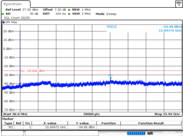
15MHz_Middle_QPSK_1@0 -34.68dBm
