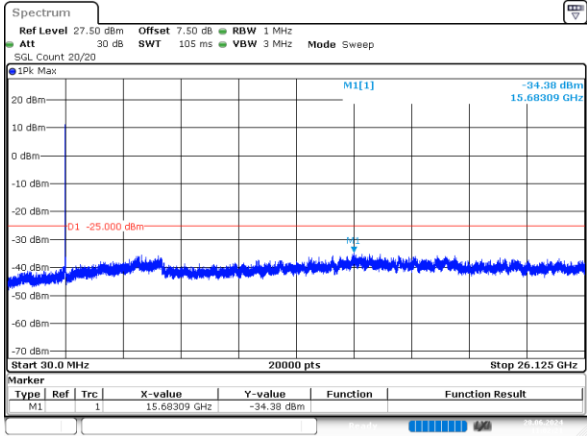
15MHz_High_QPSK_75@0 -34.38dBm
