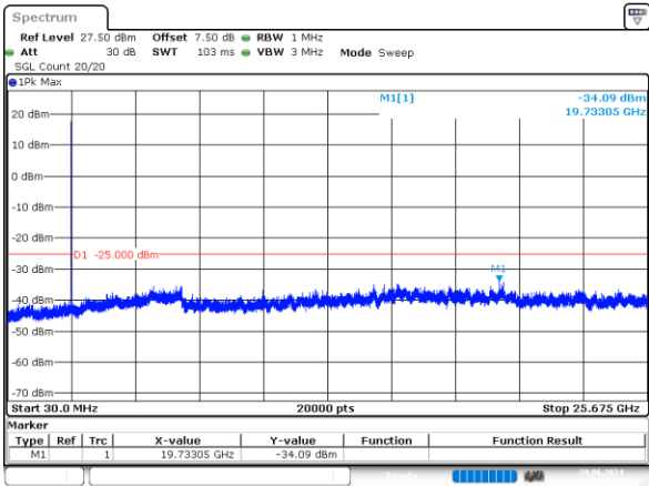
5MHz_High_QPSK_1@0 -34.09dBm
