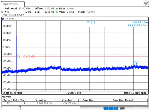
15MHz_Middle_QPSK_1@0 -24.73dBm
