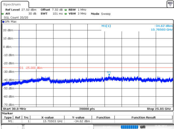
10MHz_Low_QPSK_1@0 -34.62dBm
