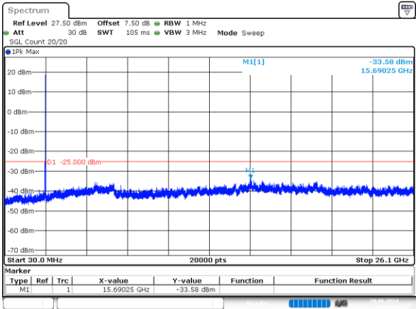
20MHz_High_QPSK_1@0 -33.58dBm
