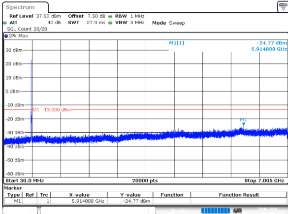
3MHz_Low_QPSK_15@0 -24.77dBm
