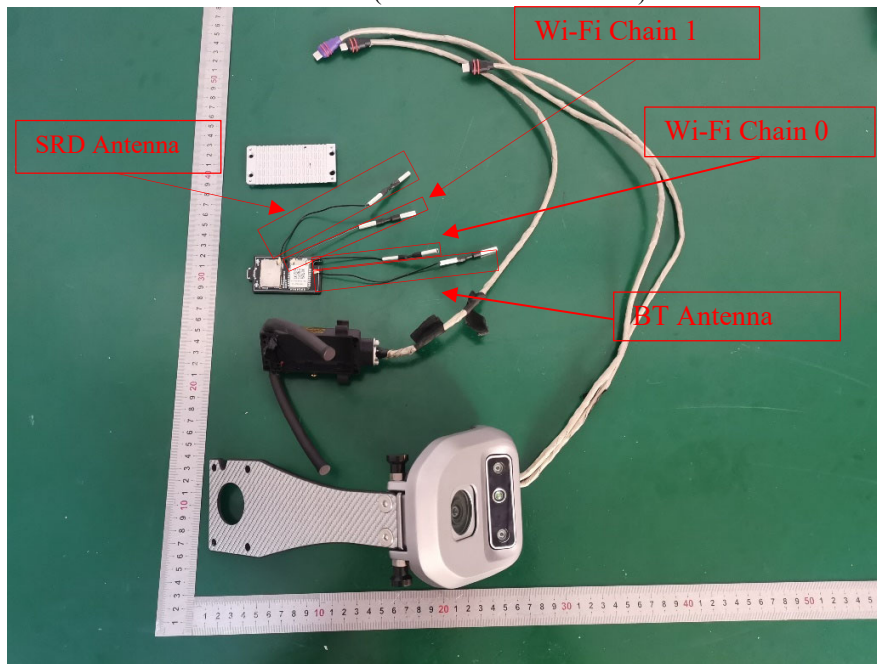
ANTENNA(All the antenna are same)
