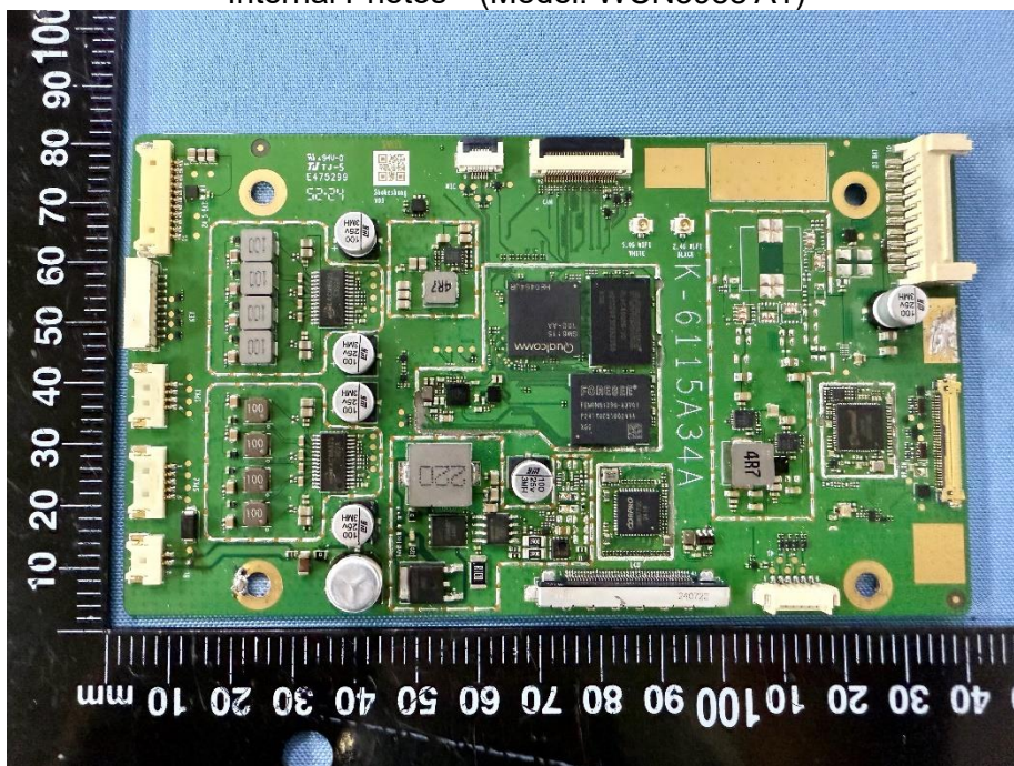
Internal Photos (Model: WCN3988 A1)
