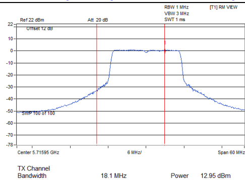
802.11an (20MHz)_Chain 1: CH 144 (For U-NII-2C)
