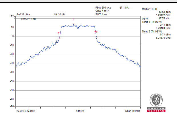
802.11ax (20MHz) / Chain 0 / CH 48
