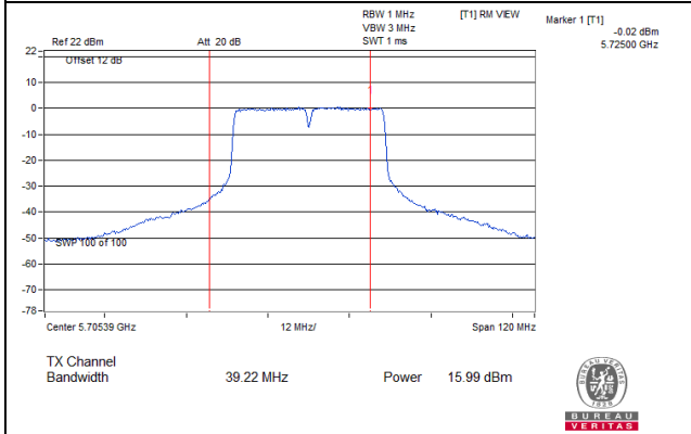
802.11ac (40MHz)_Chain 3: CH 142 (For U-NII-2C)
