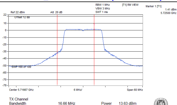
802.11a_Chain 3: CH 144 (For U-NII-2C)
