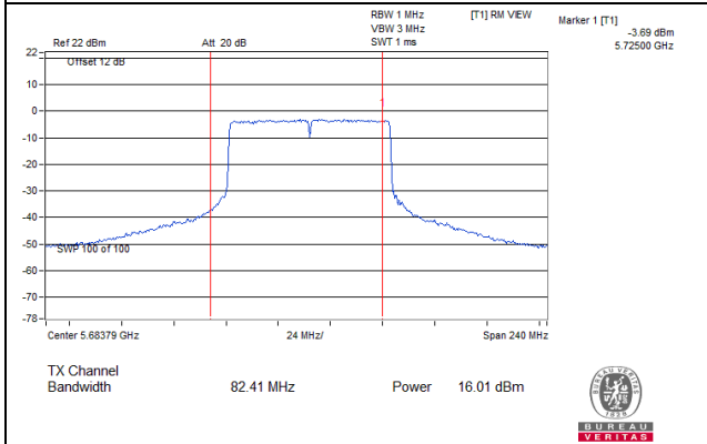
802.11ac (80MHz)_Chain 1: CH 138 (For U-NII-2C)
