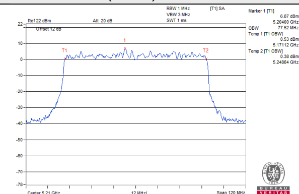
802.11ax (80MHz) / Chain 3 / CH 42
