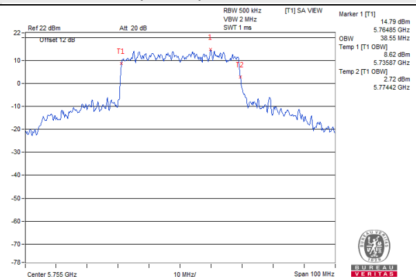
802.11ax (40MHz) / Chain 3 / CH 151
