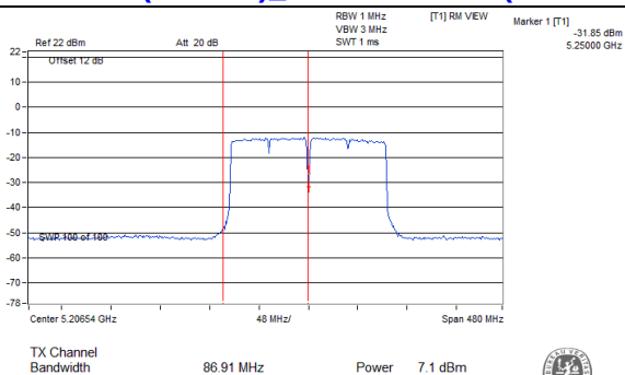
802.11ac (160MHz)_Chain 2: CH 50 (For U-NII-1)
