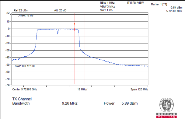
802.11ac (40MHz)_Chain 1: CH 142(For U-NII-3)
