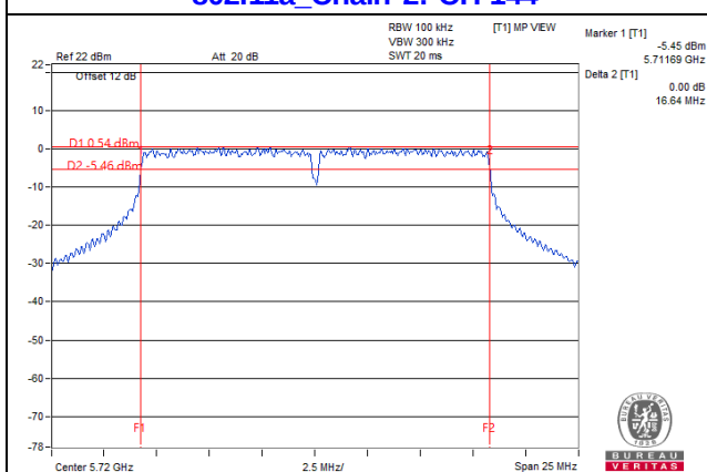
802.11a_Chain 2: CH 144
