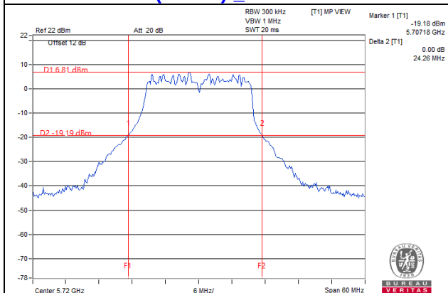
802.11ax (20MHz) _Chain 2: CH 144
