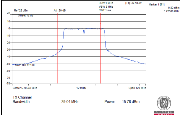
802.11ac (40MHz)_Chain 1: CH 142 (For U-NII-2C)
