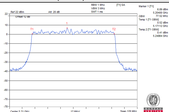
802.11ax (80MHz) / Chain 2 / CH 42
