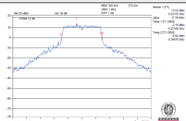
802.11ax (20MHz) / Chain 1 / CH 48
