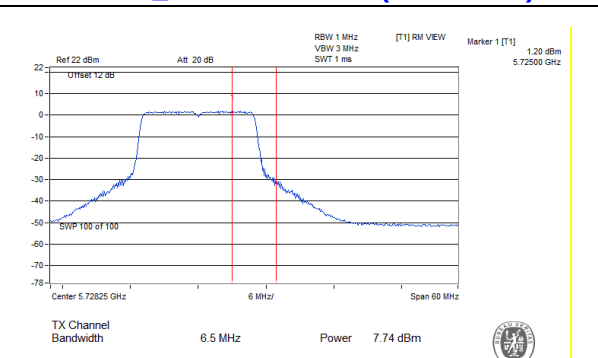
802.11a_Chain 0: CH 144 (For U-NII-3)
