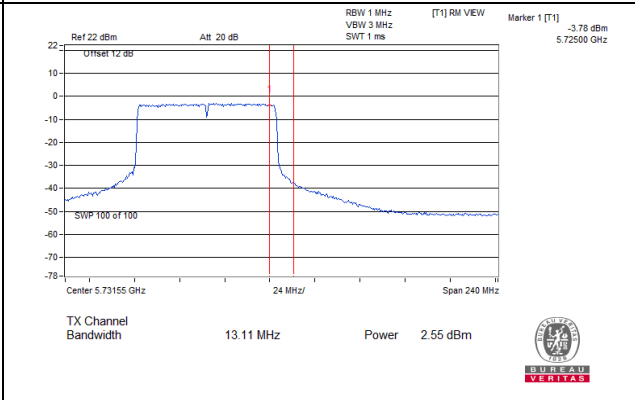
802.11ac (80MHz)_Chain 1: CH 138(For U-NII-3)
