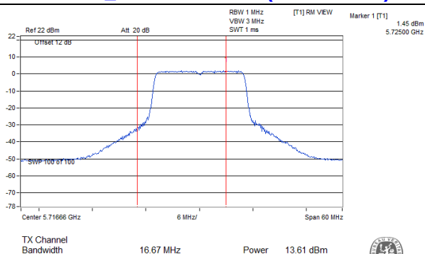
802.11a_Chain 0: CH 144 (For U-NII-2C)
