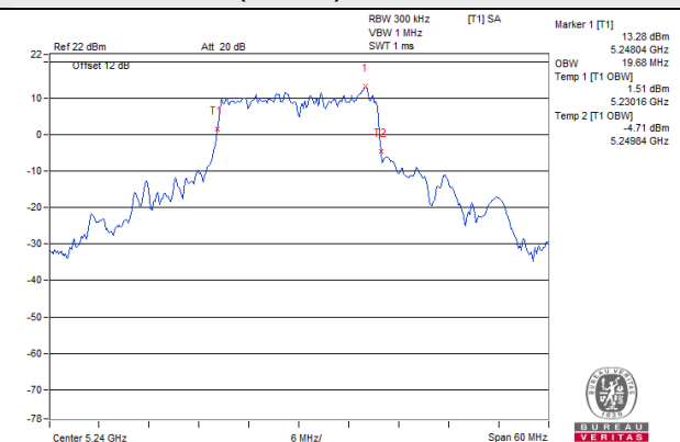
802.11ax (20MHz) / Chain 2 / CH 48
