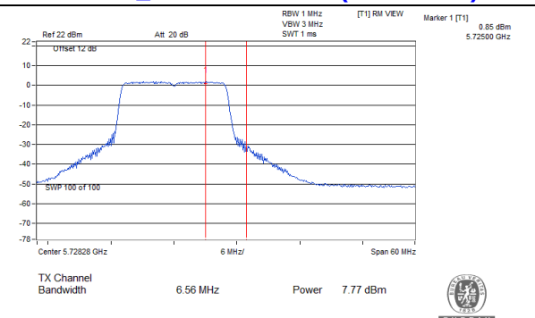
802.11a_Chain 2: CH 144 (For U-NII-3)
