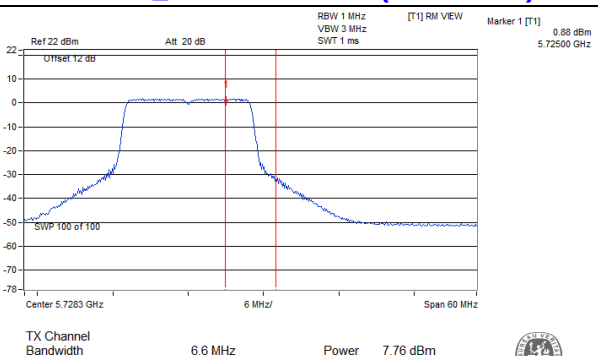
802.11a_Chain 3: CH 144 (For U-NII-3)
