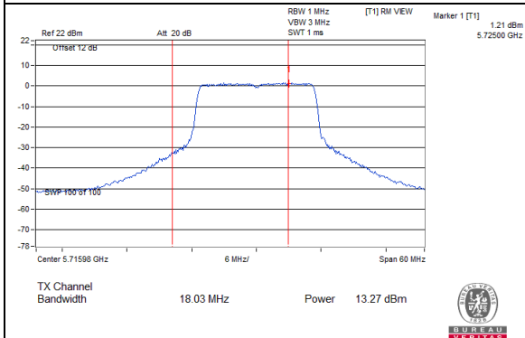
802.11ac (20MHz)_Chain 3: CH 144 (For U-NII-2C)
