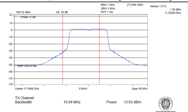
802.11a_Chain 2: CH 144 (For U-NII-2C)
