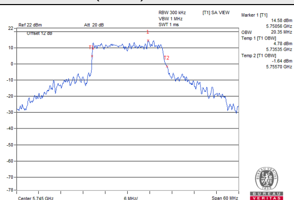
802.11ax (20MHz) / Chain 0 / CH 149
