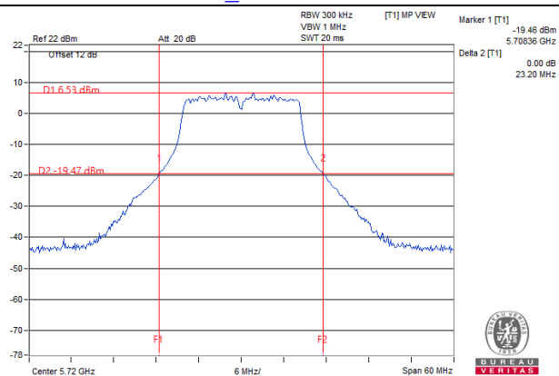
802.11a_Chain 3: CH 144
