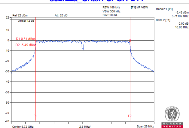
802.11a_Chain 3: CH 144
