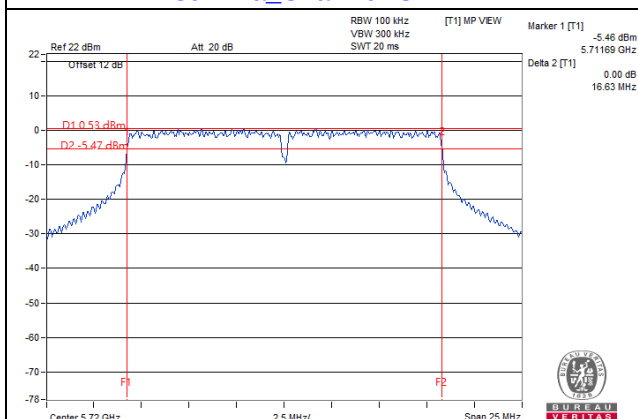
802.11a_Chain 2: CH 144
