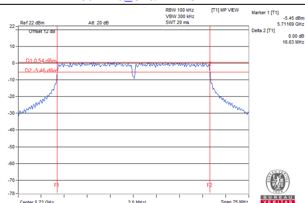
802.11a_Chain 3: CH 144
