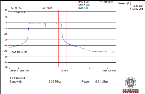
802.11ac (40MHz)_Chain 2: CH 142(For U-NII-3)
