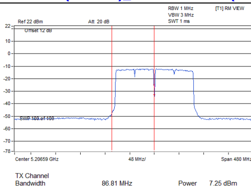
802.11ac (160MHz)_Chain 1: CH 50 (For U-NII-1)
