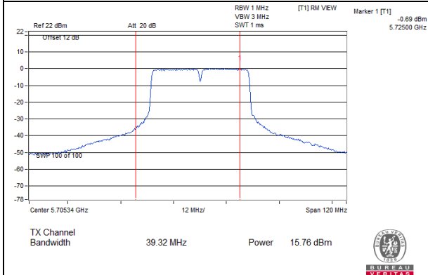
802.11ac (40MHz)_Chain 2: CH 142 (For U-NII-2C)
