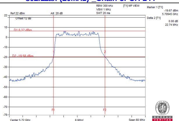
802.11ax (20MHz) _Chain 3: CH 144
