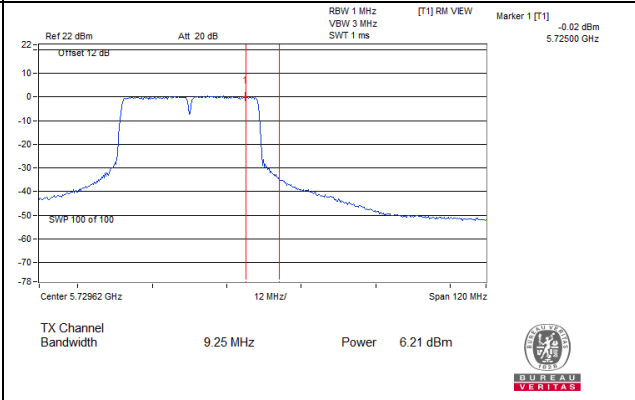
802.11ac (40MHz)_Chain 3: CH 142(For U-NII-3)
