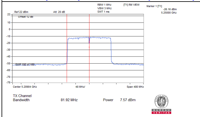
802.11ax (160MHz)_Chain 3: CH 50 (For U-NII-1)
