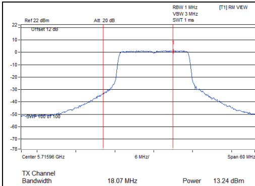
802.11ac (20MHz)_Chain 3: CH 144 (For U-NII-2C)
