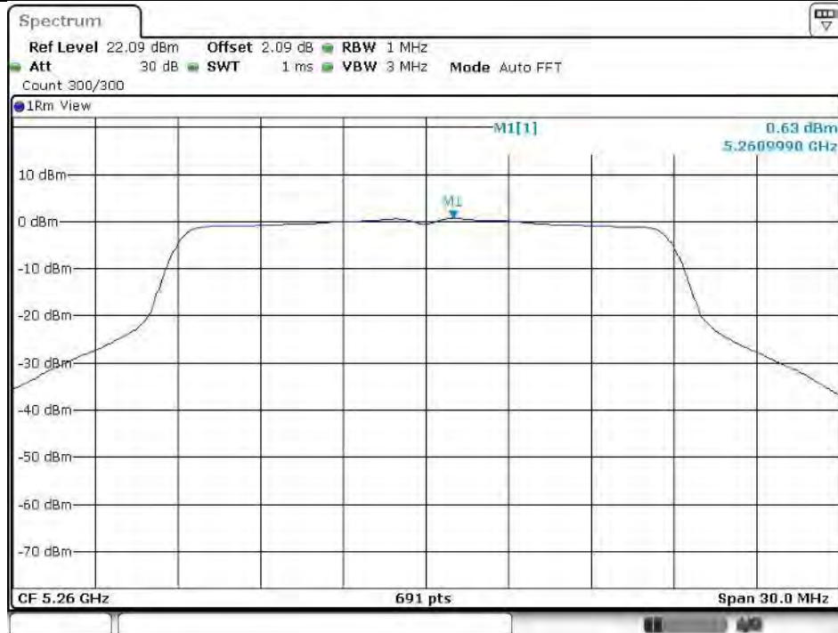
11AC20SISO_Ant2_5260
