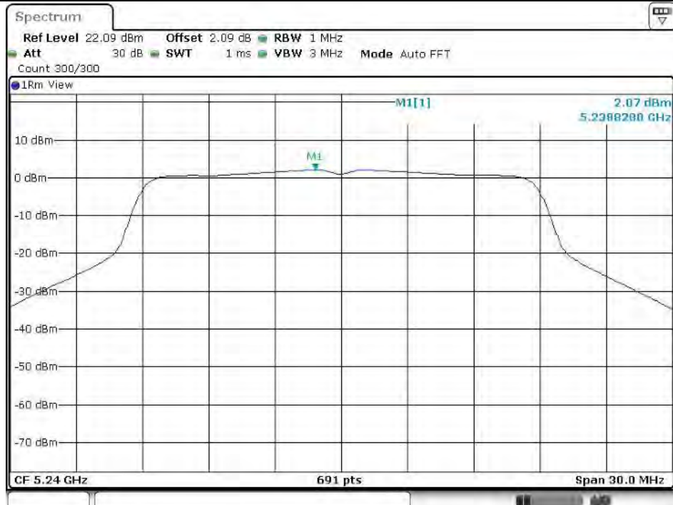
11N20SISO_Ant1_5240
