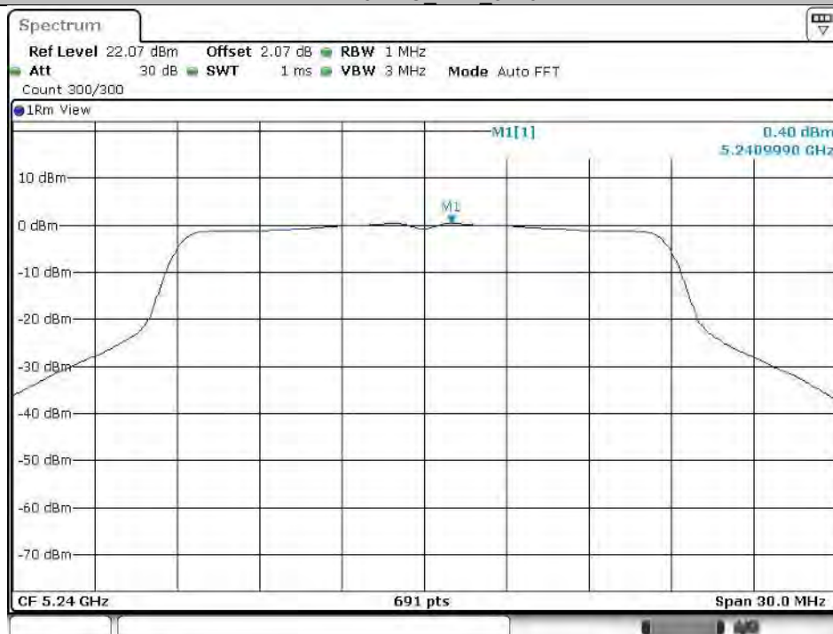
11N20SISO_Ant2_5240
