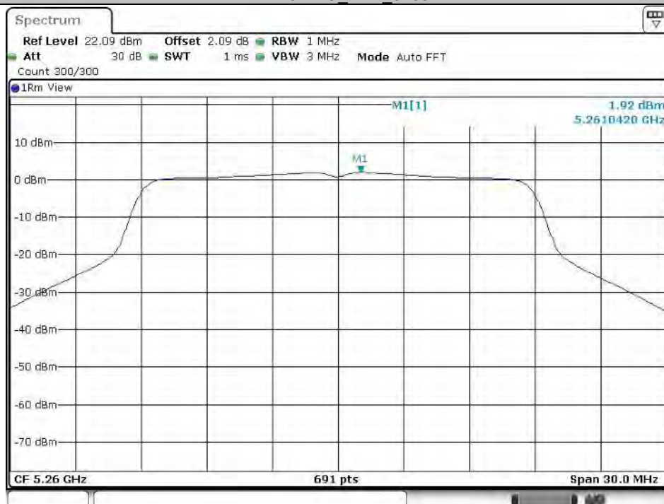
11N20SISO_Ant1_5260
