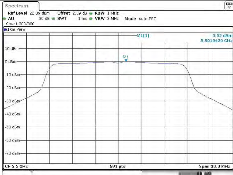
11AC20SISO_Ant1_5500
