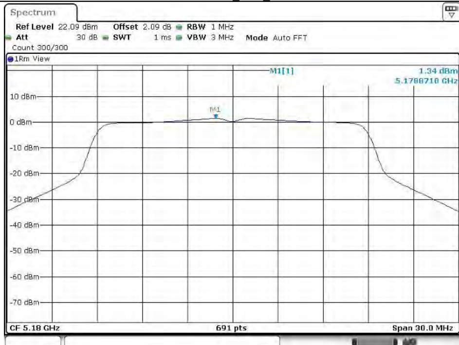
11N20SISO_Ant1_5180
