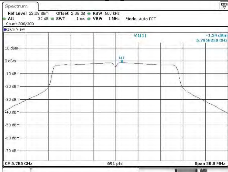
11A_Ant1_5785
