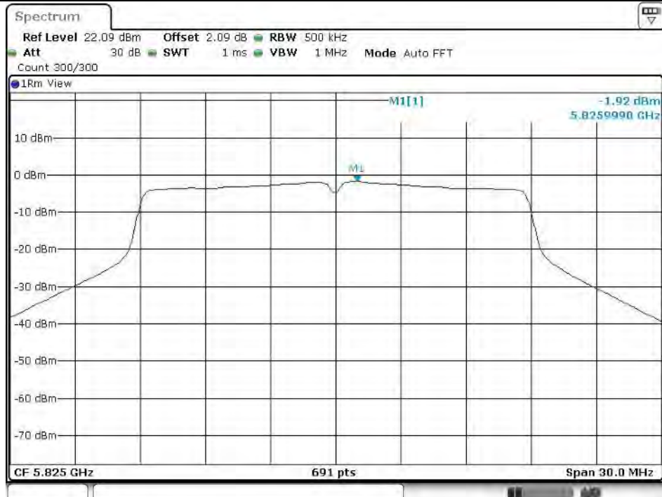
11AC20SISO_Ant1_5825
