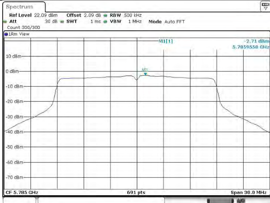
11AC20SISO_Ant2_5785
