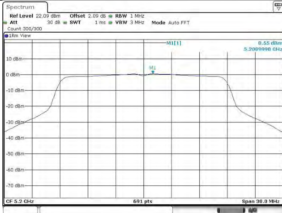
11AC20SISO_Ant2_5200
