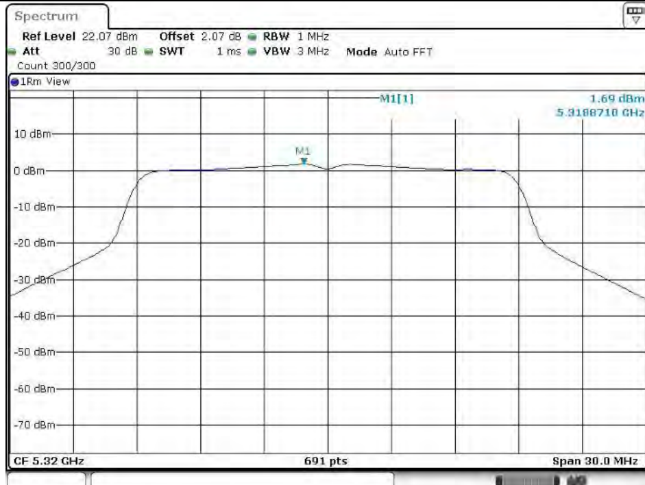
11N20SISO_Ant1_5320
