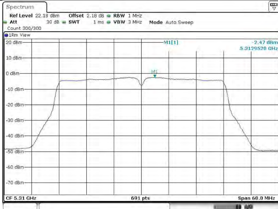
11N40SISO_Ant2_5310
