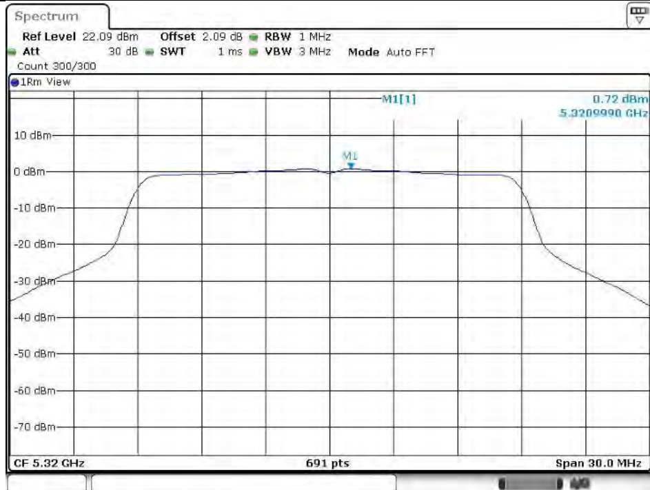
11AC20SISO_Ant2_5320
