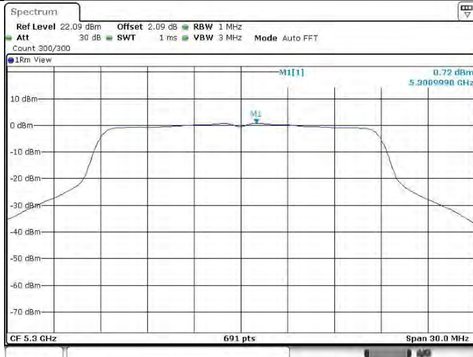
11AC20SISO_Ant2_5300
