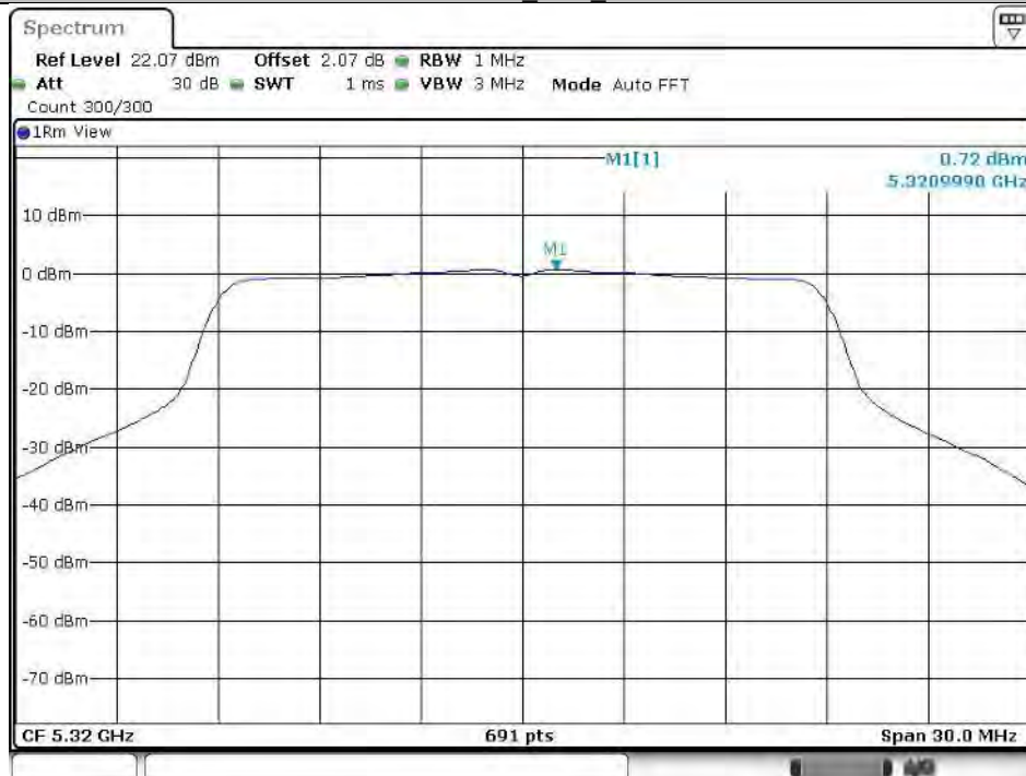
11N20SISO_Ant2_5320
