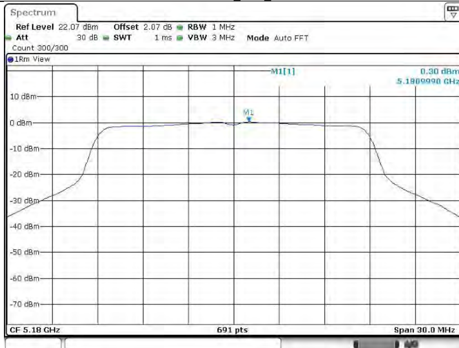
11N20SISO_Ant2_5180
