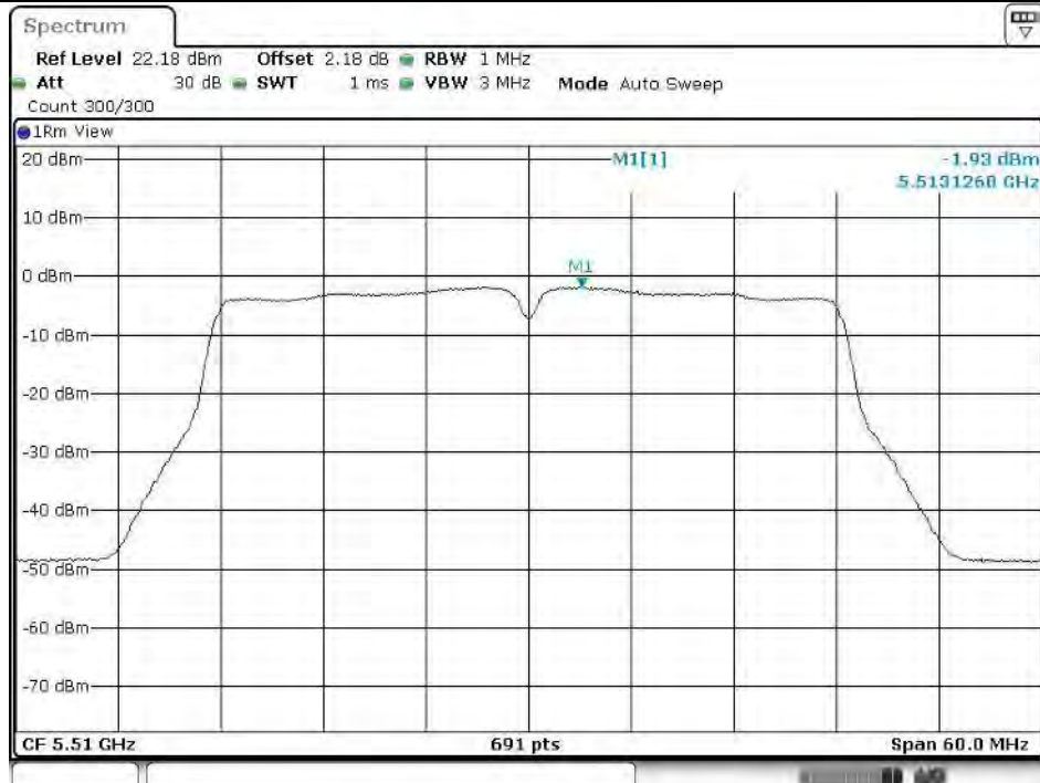
11N40SISO_Ant1_5510
