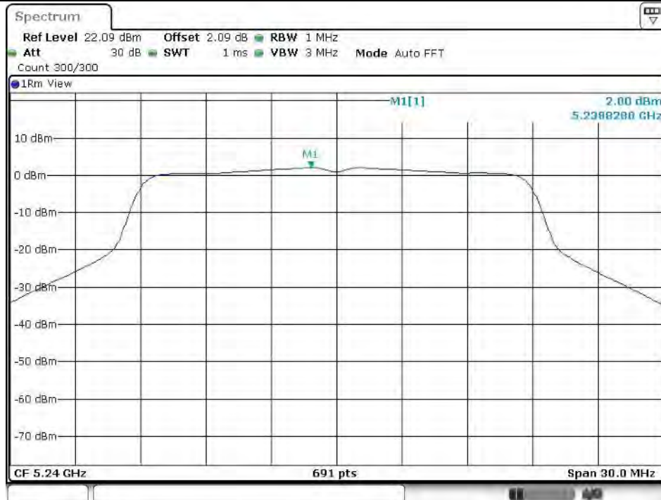
11AC20SISO_Ant1_5240
