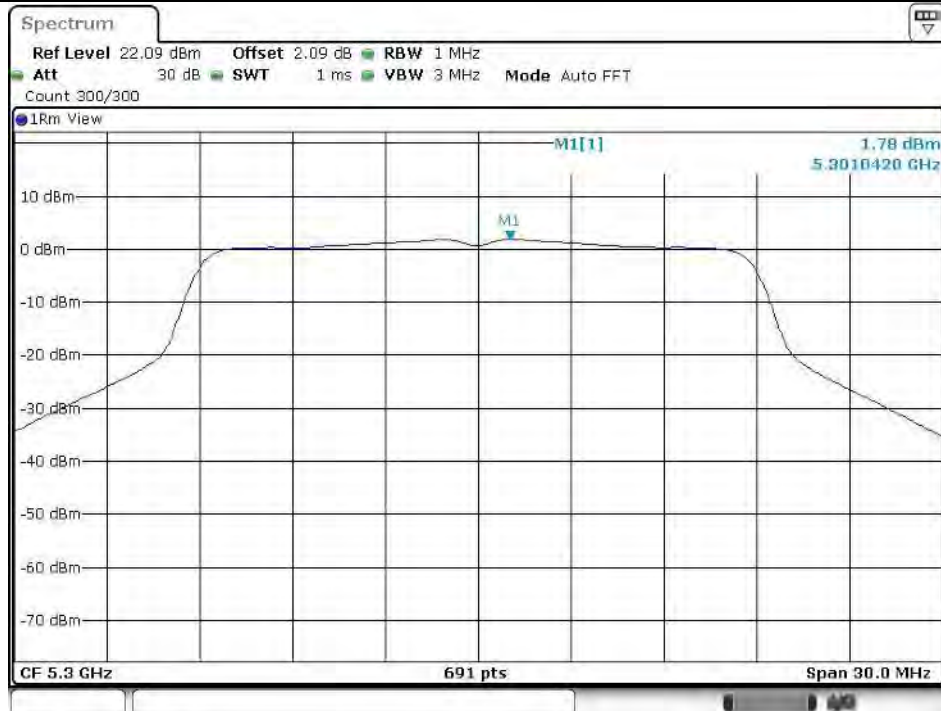
11AC20SISO_Ant1_5300
