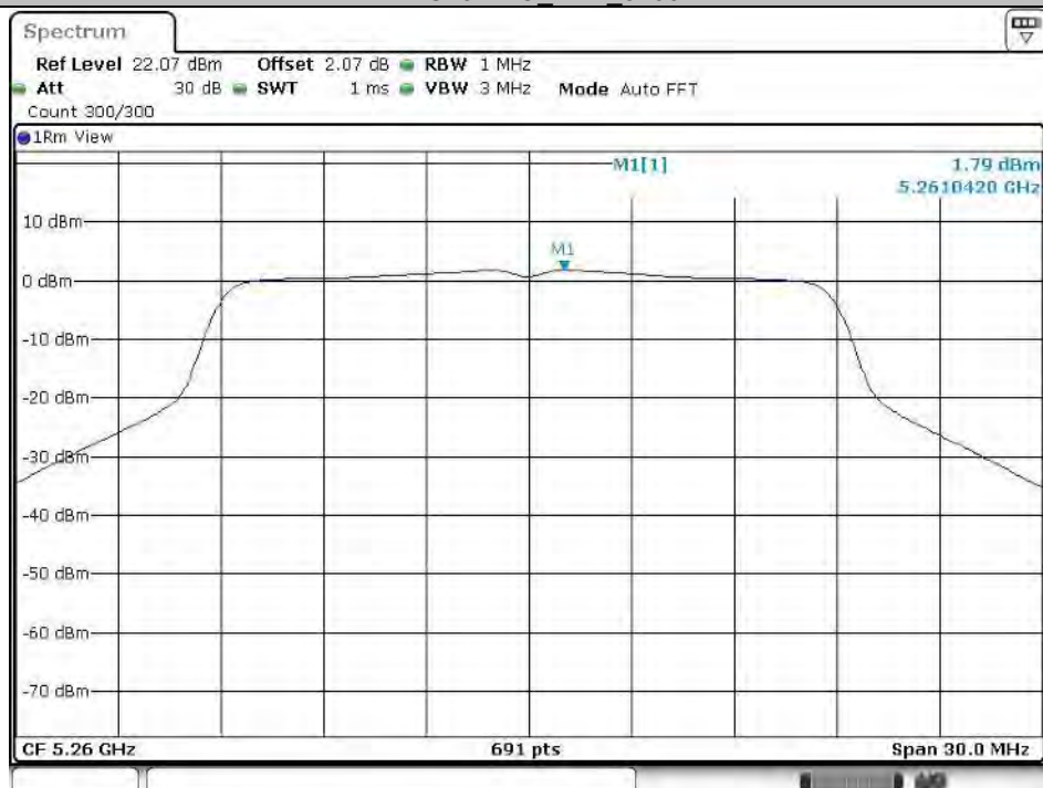
11AC20SISO_Ant1_5260
