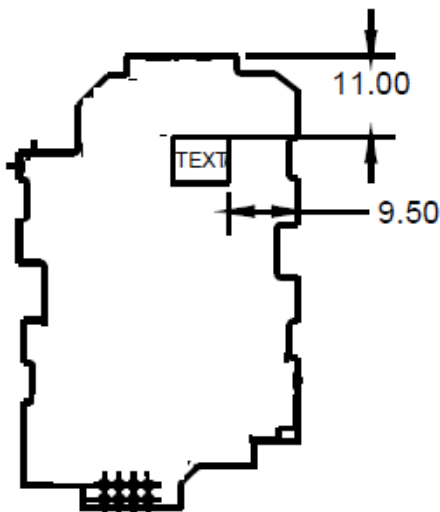
COMPLIANCE LABEL LOCATION BACK VIEW OF B8224
