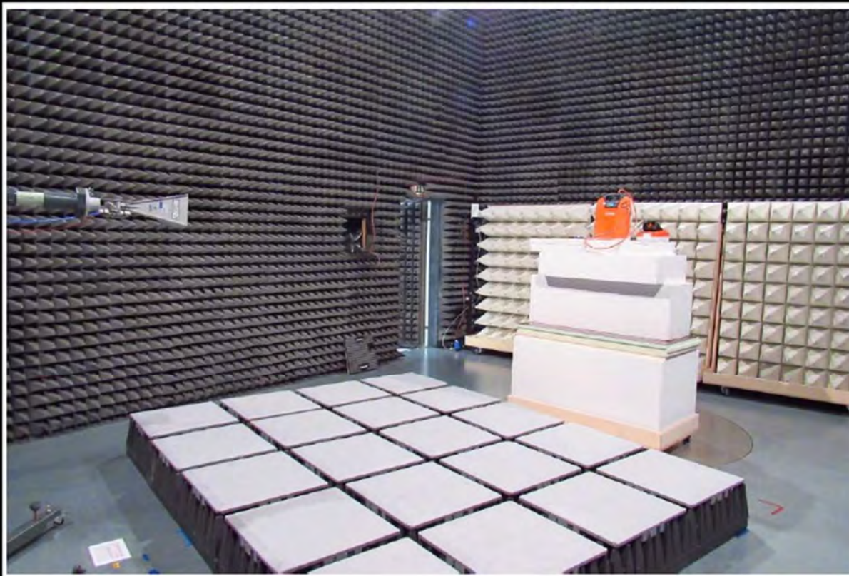
Radiated emission Tx – 6.5 GHz to 18 GHz
