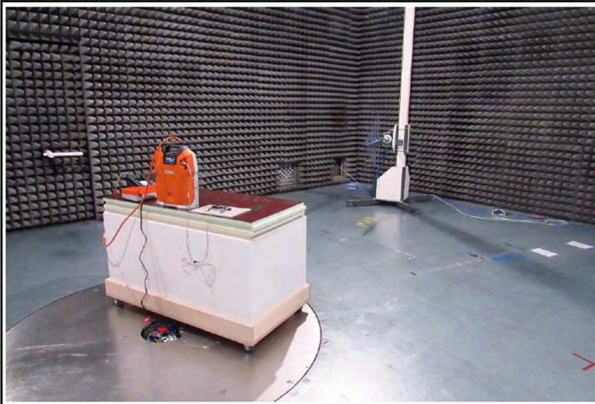
Radiated emission Tx - 200 MHz to 1 GHz
