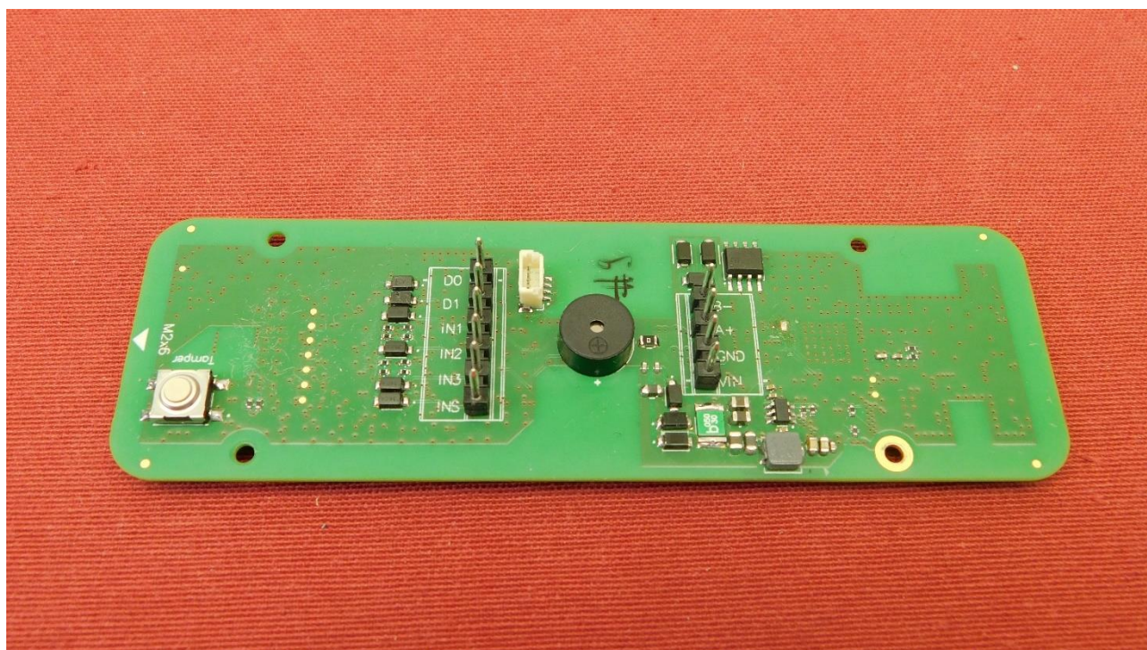
Picture 6: EUT – bottom side
