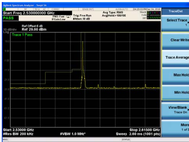
LTE Band 38 QPSK 20MHz CH-Low, 100%RB
