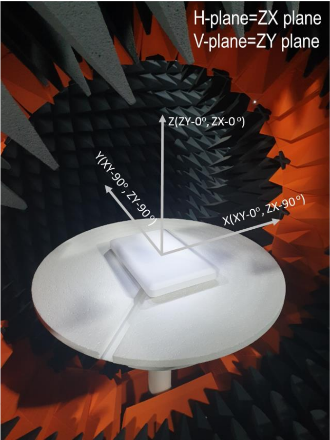
V-Pol Pattern
