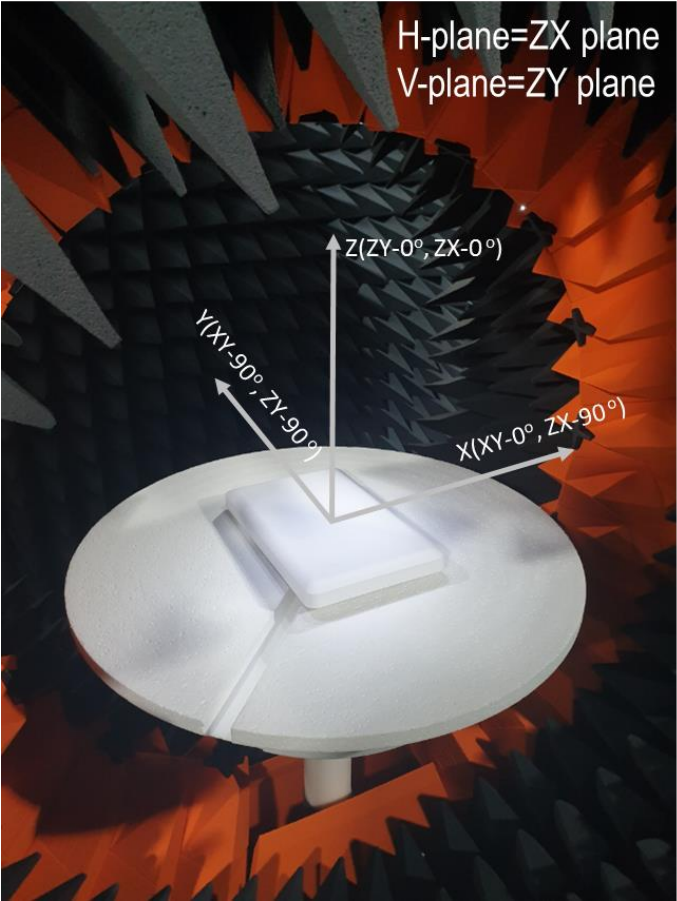
H-Pol Pattern
