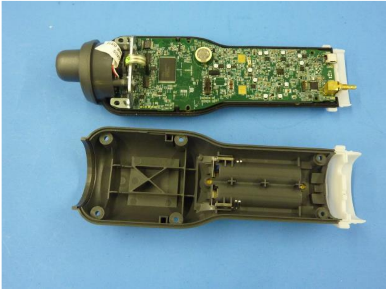
EUT Back cover open
