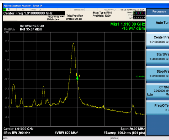
Band2-10MHz-16QAM-19150-27RB#0
