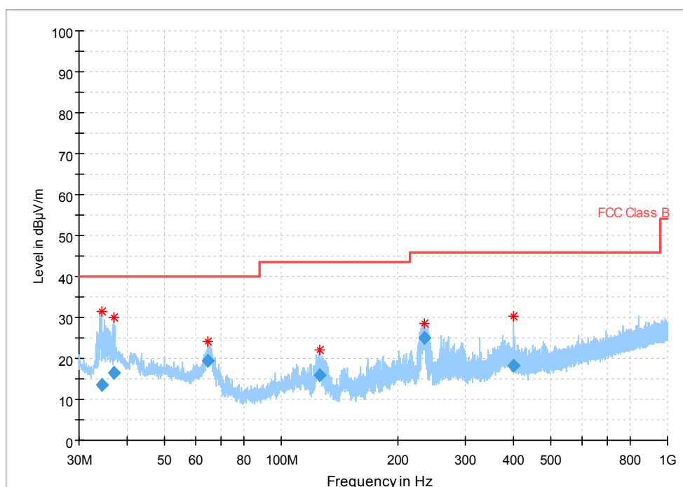
Fig. 28 Radiated Spurious Emission (802.11n-HT40, Ch151, 30 MHz-1 GHz)
