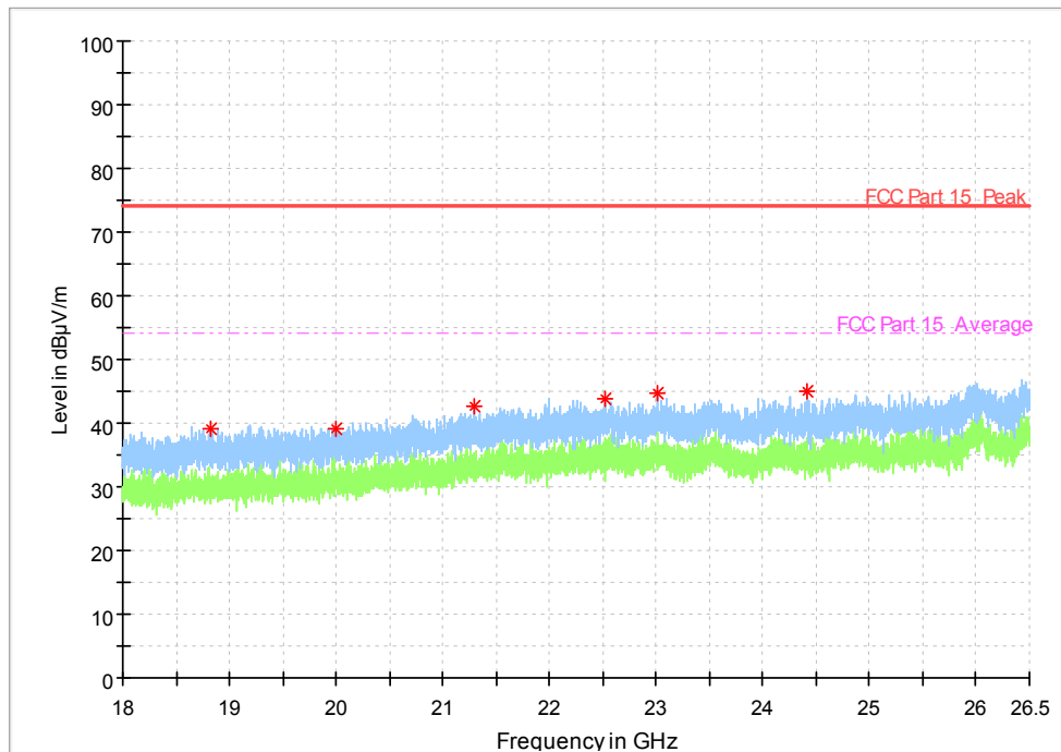
Fig. 21 Radiated Spurious Emission (802.11a, Ch141, 18 GHz-26.5 GHz)
