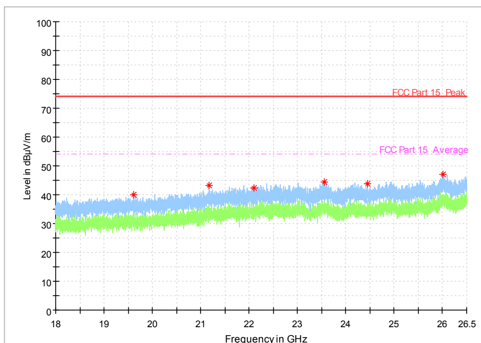
Fig. 26 Radiated Spurious Emission (802.11n-HT20, Ch149, 18 GHz-26.5 GHz)
