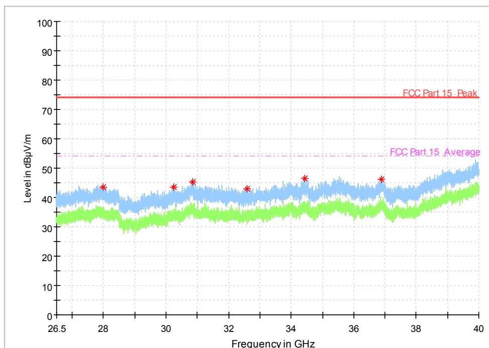
Fig. 27 Radiated emission: 802.11n, (802.11n-HT20, Ch149, 26.5 GHz - 40 GHz)
