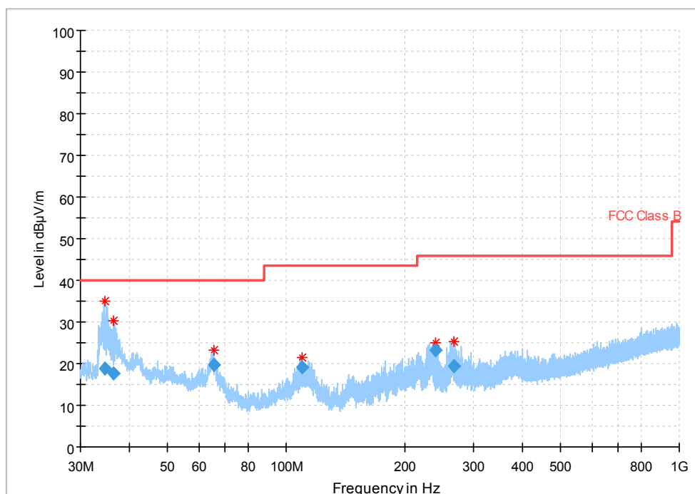
Fig. 23 Radiated Spurious Emission (802.11n-HT20, Ch149, 30 MHz-1 GHz)
