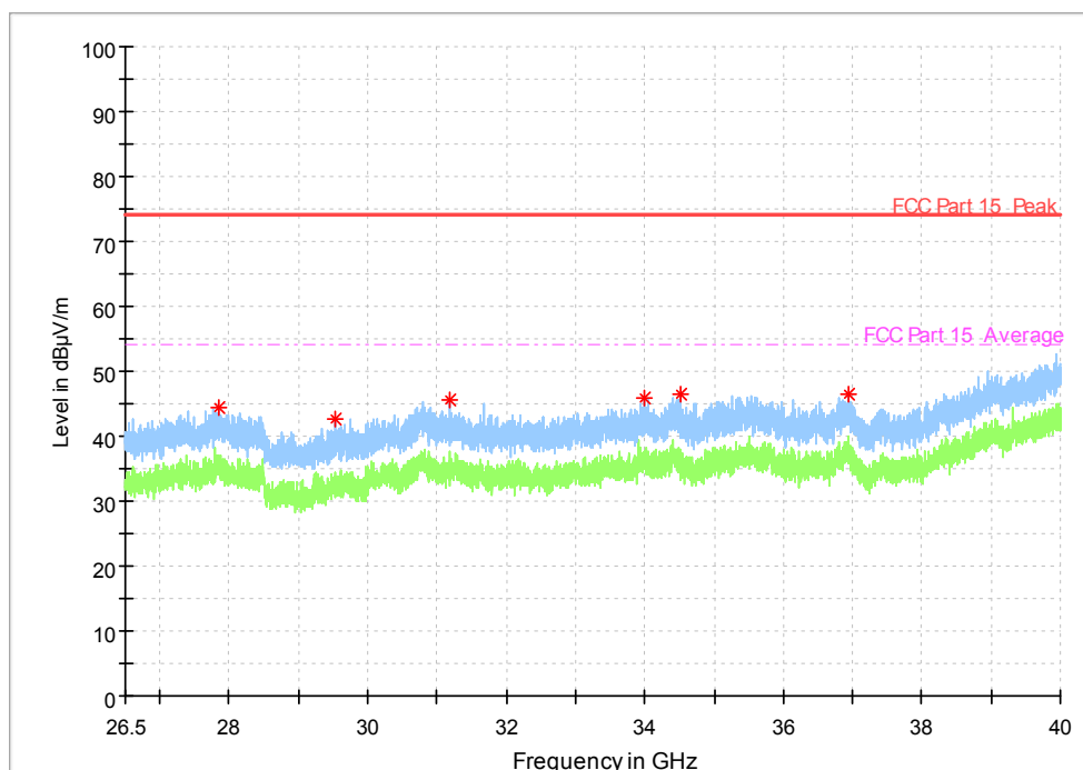
Fig. 32 Radiated emission: 802.11n, (802.11n-HT40, Ch151, 26.5 GHz - 40 GHz)
