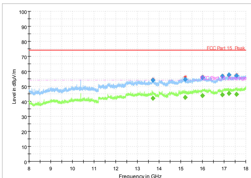
Fig. 30 Radiated Spurious Emission (802.11n-HT40, Ch151, 8 GHz-18 GHz)
