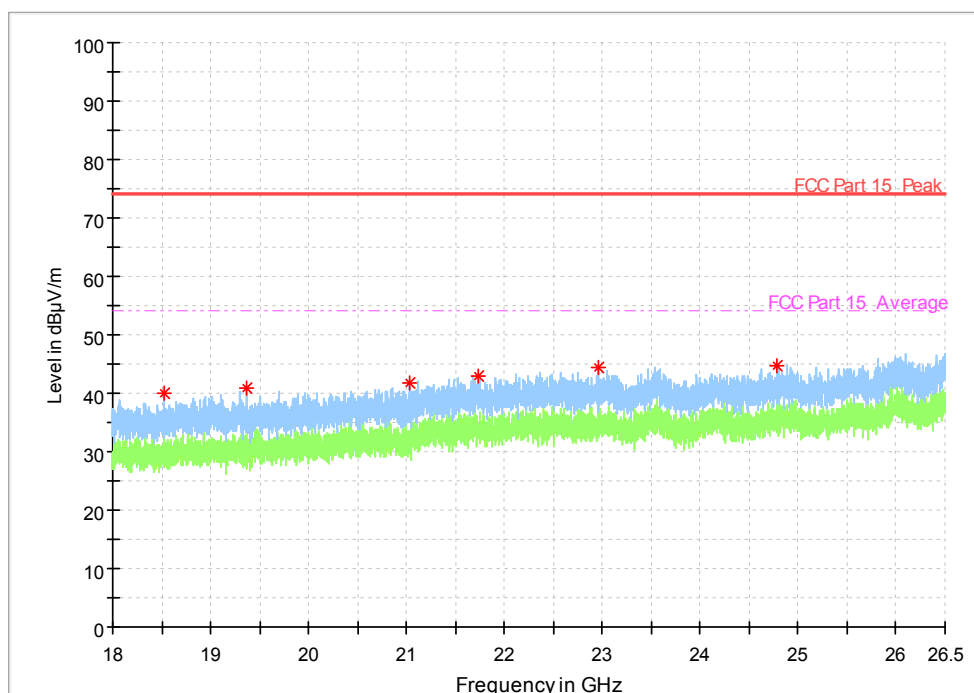
Fig. 31 Radiated Spurious Emission (802.11n-HT40, Ch151 18 GHz-26.5 GHz)
