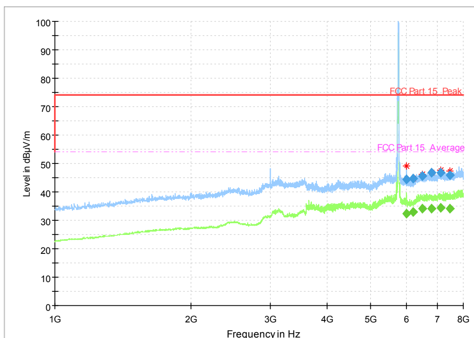
Fig. 24 Radiated Spurious Emission (802.11n-HT20, Ch149, 1 GHz-8 GHz)
