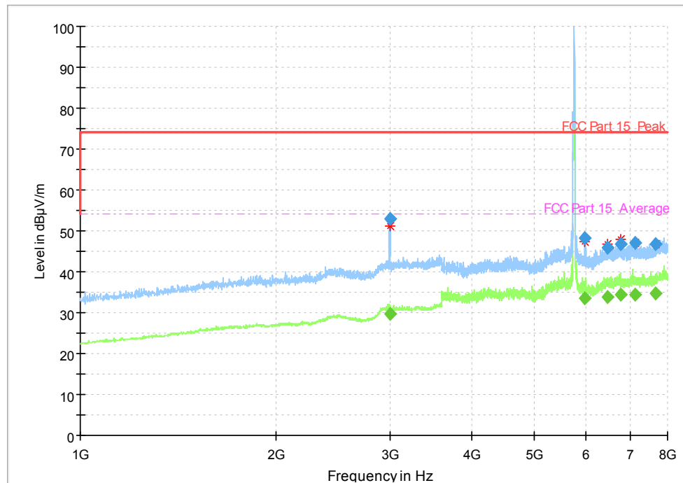
Fig. 19 Radiated Spurious Emission (802.11a, Ch141, 1 GHz-8 GHz)
