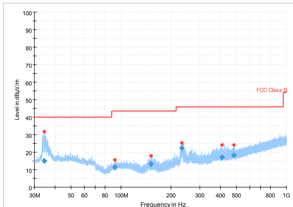
Fig. 18 Radiated Spurious Emission (802.11a, Ch141, 30 MHz-1 GHz)
