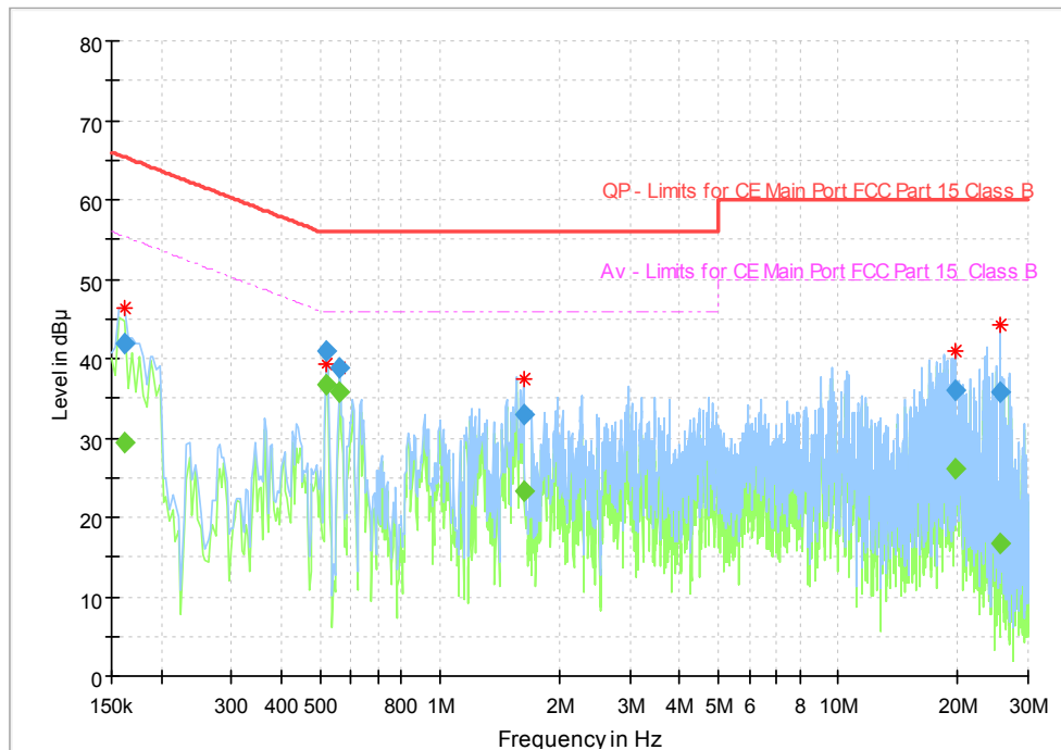
Fig. 39 AC Powerline Conducted Emission-802.11a
