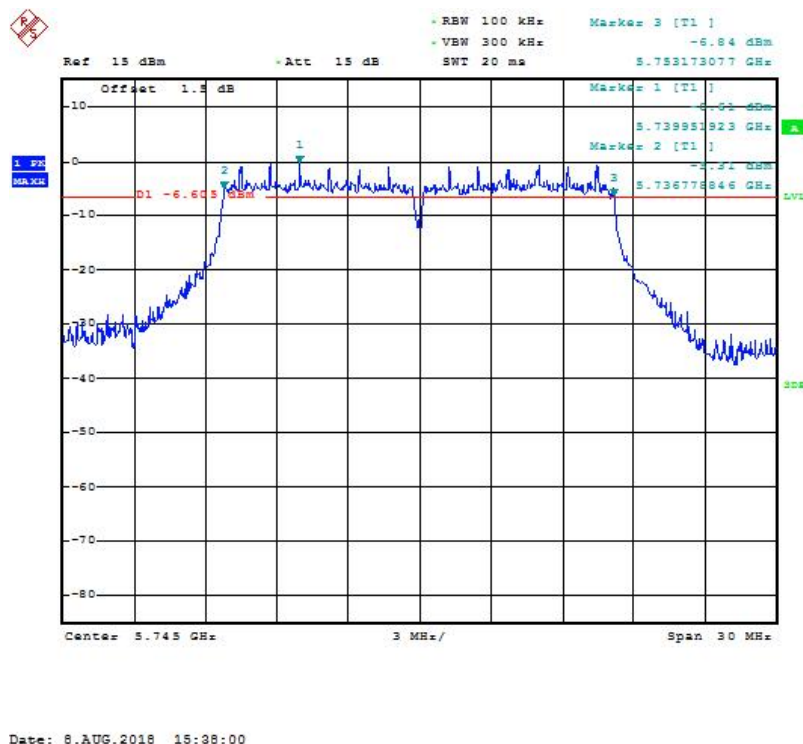
Fig. 1 Occupied 6dB Bandwidth (802.11a, Ch 149)
