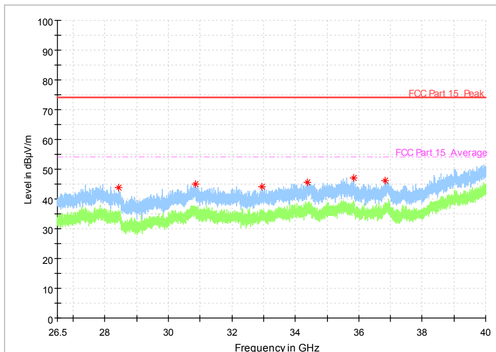
Fig. 22 Radiated emission: 802.11n, (802.11a, Ch141, 26.5 GHz - 40 GHz)
