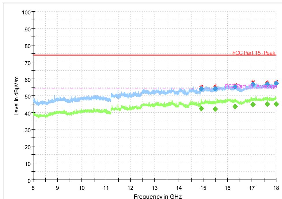
Fig. 20 Radiated Spurious Emission (802.11a, Ch141, 8 GHz-18 GHz)
