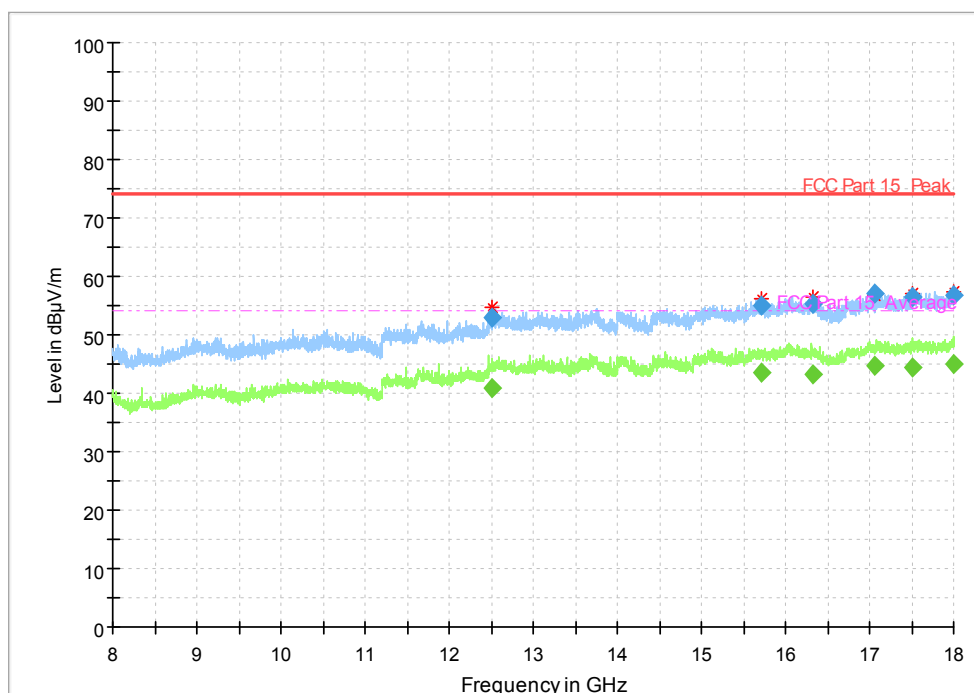
Fig. 25 Radiated Spurious Emission (802.11n-HT20, Ch149, 8 GHz-18 GHz)
