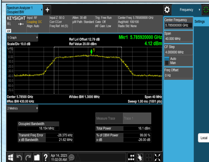
11N20SISO-Ant1-5785
