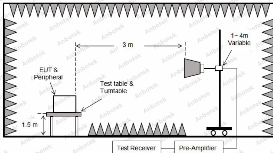
Figure 3. Above 1 GHz
