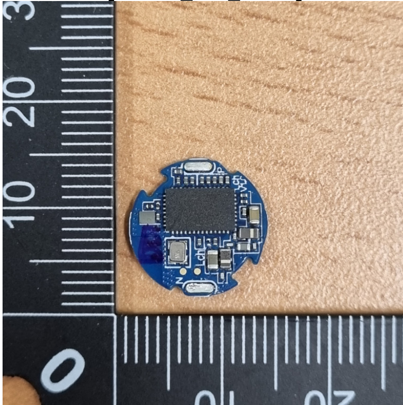
[Earbud_Left_Board]
