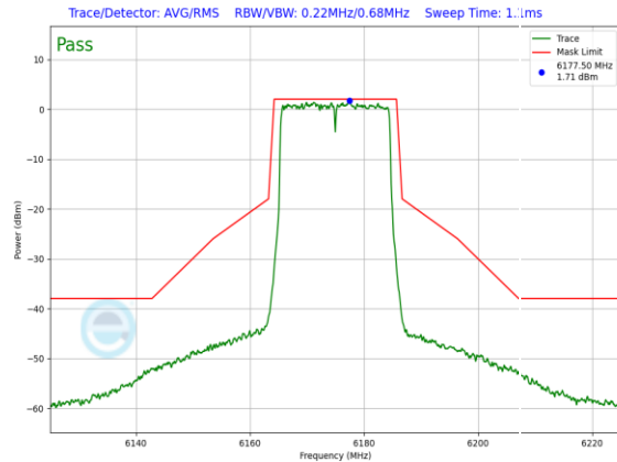
Plot 7-722. In-Band Emission Plot SDM Antenna WF7a Standard Power (20MHz 802.11ax (UNII Band 5) – Ch. 45, MCS2)
