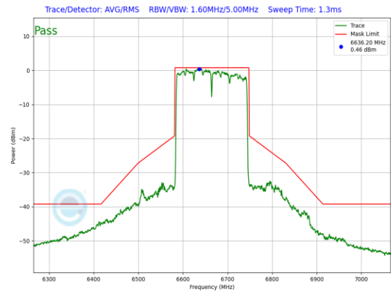
Plot 7-768. In-Band Emission Plot CDD Antenna WF7a Standard Power (160MHz 802.11ax (UNII Band 7) – Ch. 143, MCS11)
