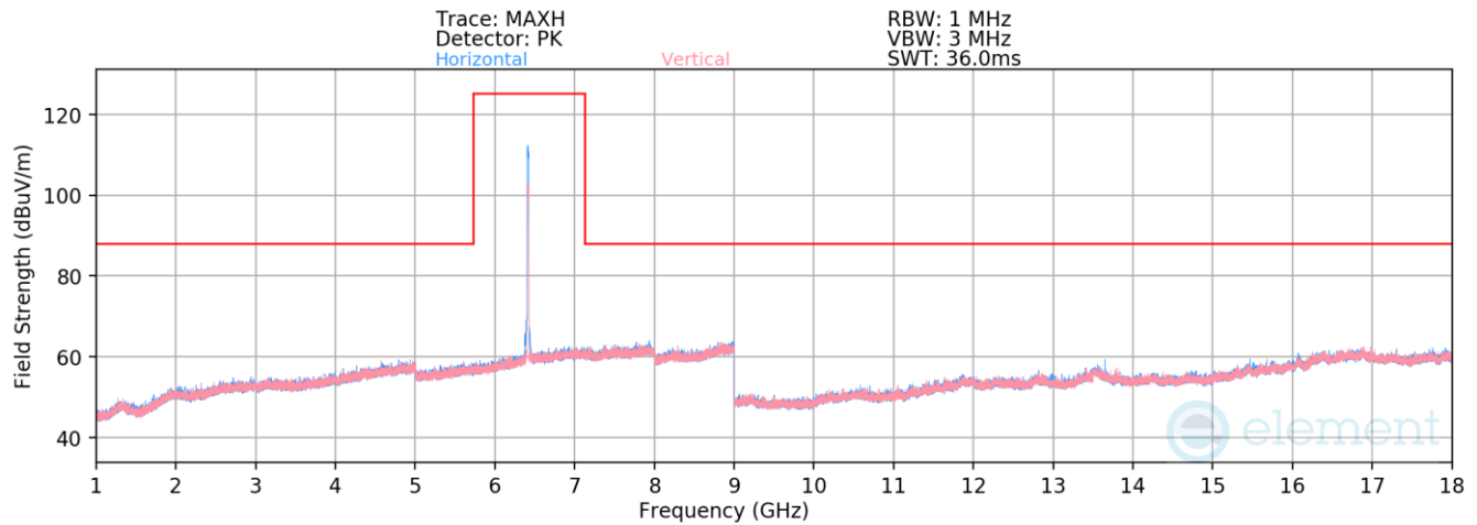
Plot 7-807. Radiated Spurious Emissions above 1GHz Antenna WF8 (802.11ax – Ch. 93)
