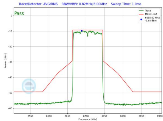
Plot 7-710. In-Band Emission Plot SDM Antenna WF7a Low Power Indoor (80MHz 802.11ax (UNII Band 7) – Ch. 151, MCS11)
