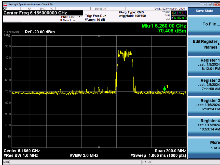
Plot 7-804. 160MHz Bandwidth – AWGN Signal Injected at High End – Channel 47
