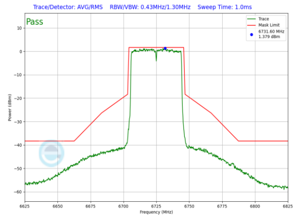
Plot 7-731. In-Band Emission Plot CDD Antenna WF8 Standard Power (40MHz 802.11ax (UNII Band 7) – Ch. 155, MCS2)
