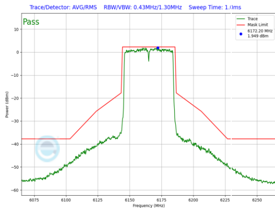
Plot 7-739. In-Band Emission Plot SDM Antenna WF8 Standard Power (40MHz 802.11ax (UNII Band 5) – Ch. 43, MCS4)
