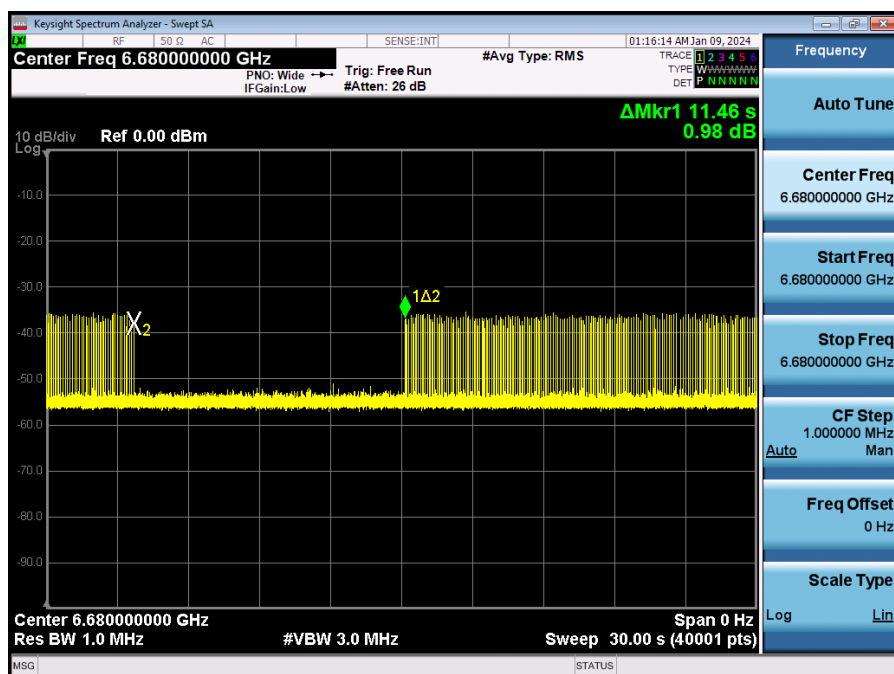
Plot 7-795. Contention Based Protocol Timing Plot – UNII 7 – 160MHz Channel 143 – Mid
