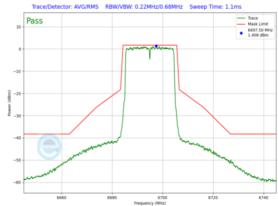
Plot 7-730. In-Band Emission Plot SDM Antenna WF7a Standard Power (20MHz 802.11ax (UNII Band 7) – Ch. 149, MCS2)
