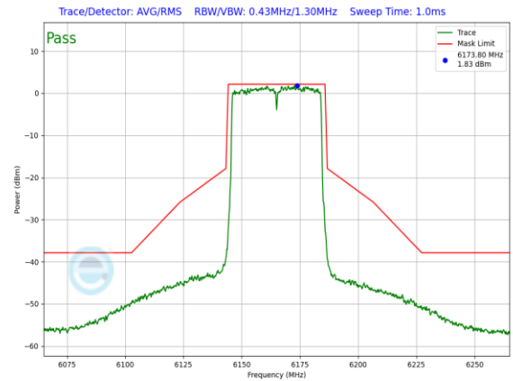
Plot 7-724. In-Band Emission Plot SDM Antenna WF7a Standard Power (40MHz 802.11ax (UNII Band 5) – Ch. 43, MCS2)
