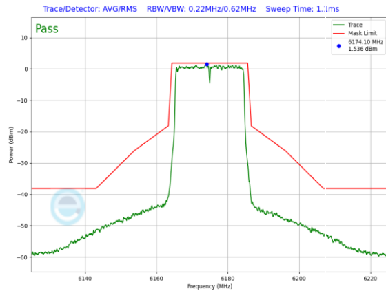
Plot 7-721. In-Band Emission Plot SDM Antenna WF8 Standard Power (20MHz 802.11ax (UNII Band 5) – Ch. 45, MCS2)
