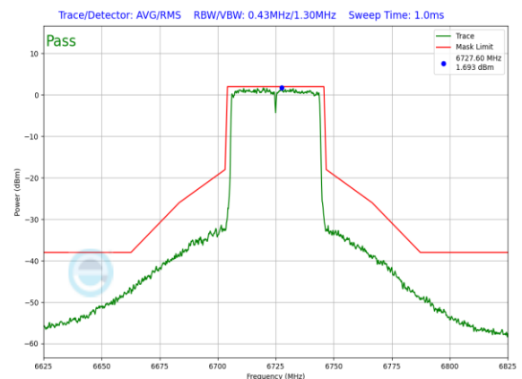
Plot 7-748. In-Band Emission Plot CDD Antenna WF7a Standard Power (40MHz 802.11ax (UNII Band 7) – Ch. 155, MCS4)
