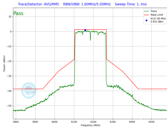
Plot 7-743. In-Band Emission Plot CDD Antenna WF8 Standard Power (160MHz 802.11ax (UNII Band 5) – Ch. 47, MCS4)
