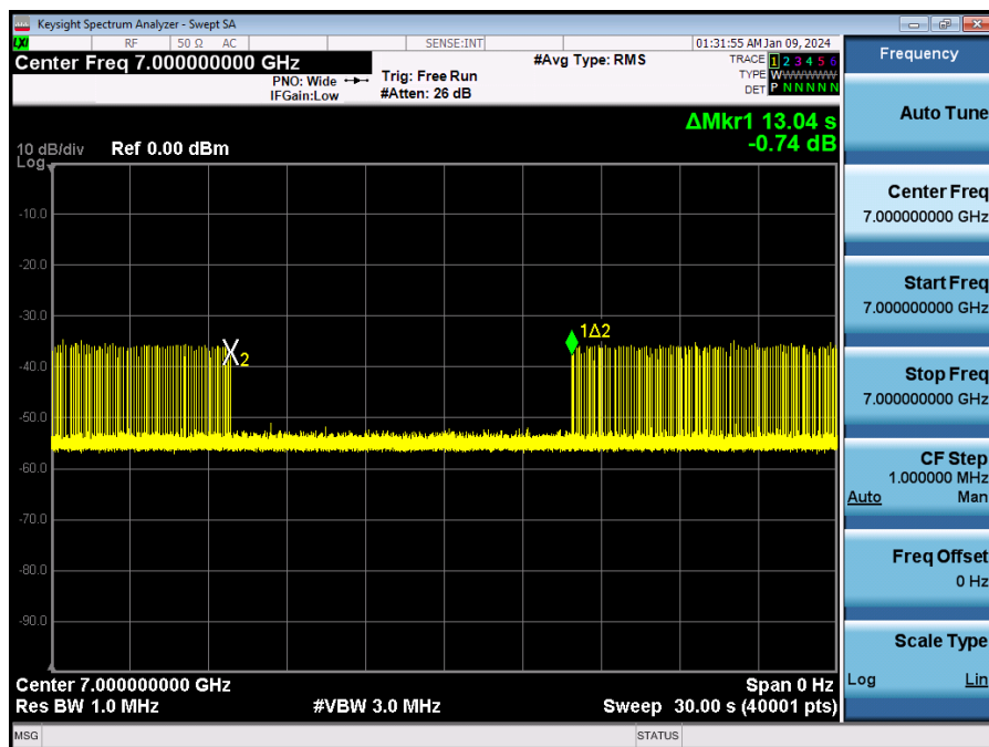
Plot 7-800. Contention Based Protocol Timing Plot – UNII 8 – 160MHz Channel 207 – High
