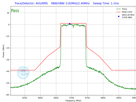
Plot 7-749. In-Band Emission Plot CDD Antenna WF8 Standard Power (80MHz 802.11ax (UNII Band 7) – Ch. 151, MCS4)
