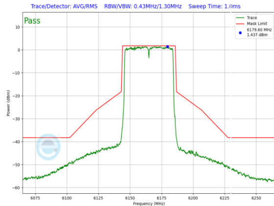
Plot 7-723. In-Band Emission Plot SDM Antenna WF8 Standard Power (40MHz 802.11ax (UNII Band 5) – Ch. 43, MCS2)
