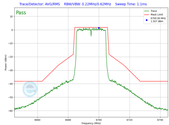
Plot 7-746. In-Band Emission Plot SDM Antenna WF7a Standard Power (20MHz 802.11ax (UNII Band 7) – Ch. 149, MCS4)
