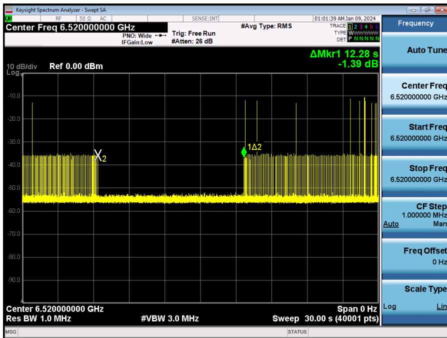
Plot 7-790. Contention Based Protocol Timing Plot – UNII 6 – 160MHz Channel 111 – Low
