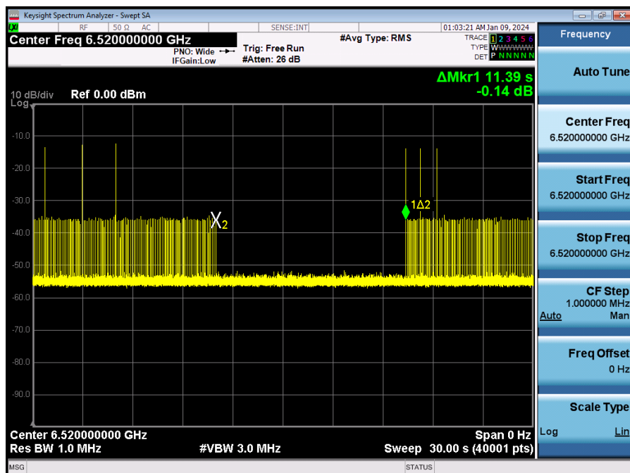
Plot 7-791. Contention Based Protocol Timing Plot – UNII 6 – 160MHz Channel 111 – Mid
