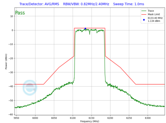
Plot 7-757. In-Band Emission Plot CDD Antenna WF8 Standard Power (80MHz 802.11ax (UNII Band 5) – Ch. 39, MCS11)
