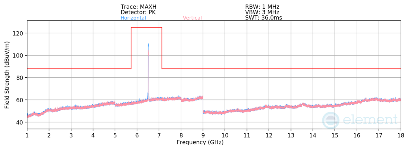
Plot 7-810. Radiated Spurious Emissions above 1GHz Antenna WF8 (802.11ax – Ch. 113)
