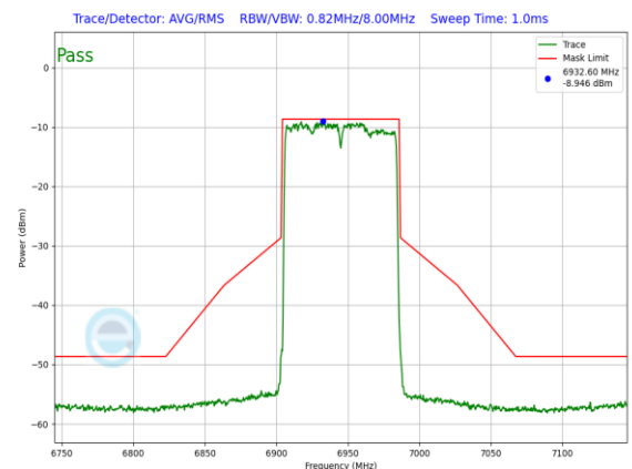
Plot 7-718. In-Band Emission Plot SDM Antenna WF7a Low Power Indoor (80MHz 802.11ax (UNII Band 8) – Ch. 199, MCS11)
