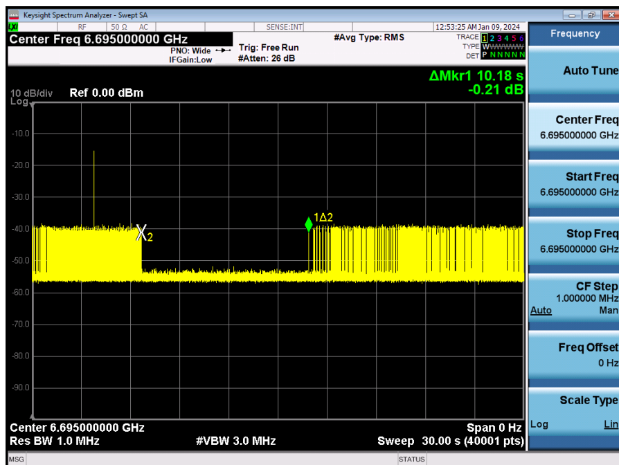
Plot 7-793. Contention Based Protocol Timing Plot – UNII 7 – 20MHz Channel 149
