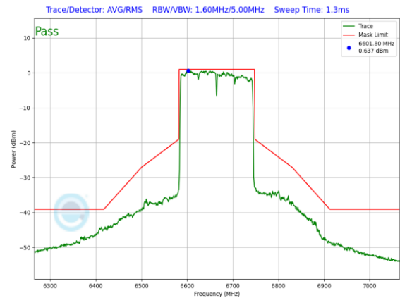
Plot 7-752. In-Band Emission Plot CDD Antenna WF7a Standard Power (160MHz 802.11ax (UNII Band 7) – Ch. 143, MCS4)
