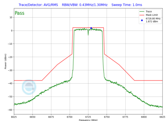
Plot 7-732. In-Band Emission Plot CDD Antenna WF7a Standard Power (40MHz 802.11ax (UNII Band 7) – Ch. 155, MCS2)
