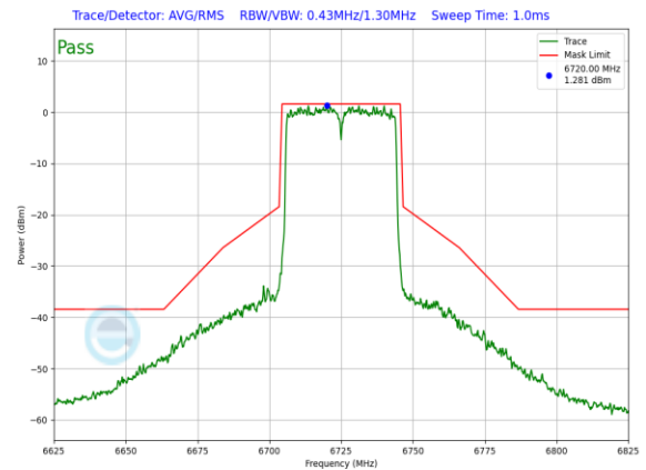
Plot 7-763. In-Band Emission Plot CDD Antenna WF8 Standard Power (40MHz 802.11ax (UNII Band 7) – Ch. 155, MCS11)
