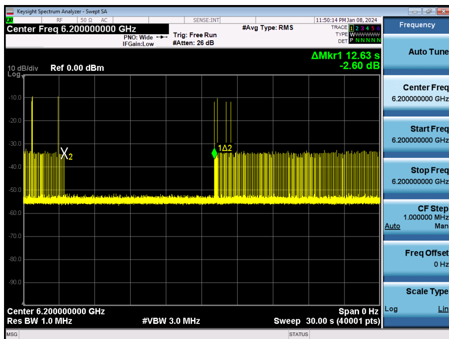
Plot 7-786. Contention Based Protocol Timing Plot – UNII 5 – 160MHz Channel 47 – Low
