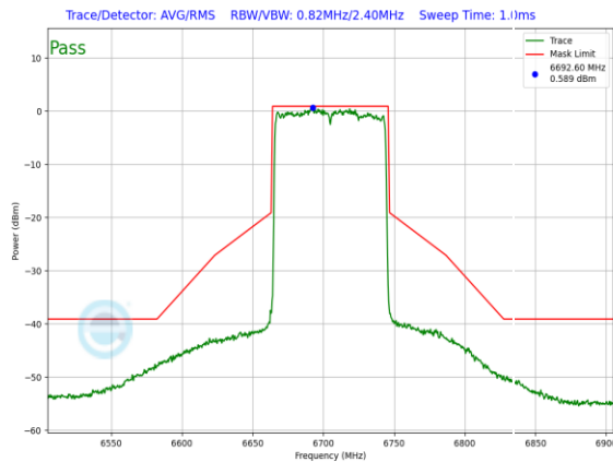
Plot 7-733. In-Band Emission Plot CDD Antenna WF8 Standard Power (80MHz 802.11ax (UNII Band 7) – Ch. 151, MCS2)
