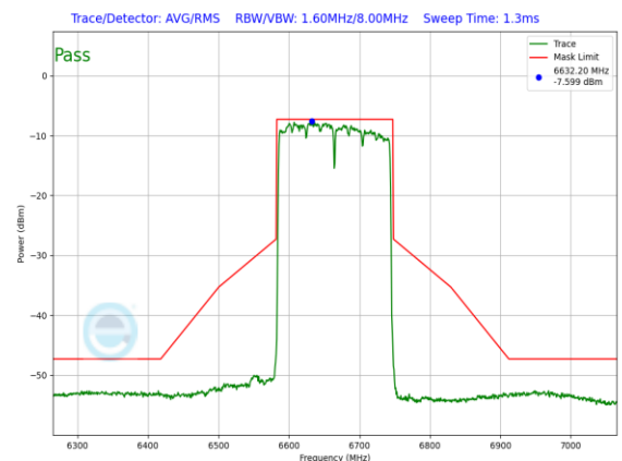
Plot 7-712. In-Band Emission Plot SDM Antenna WF7a Low Power Indoor (160MHz 802.11ax (UNII Band 7) – Ch. 143, MCS11)
