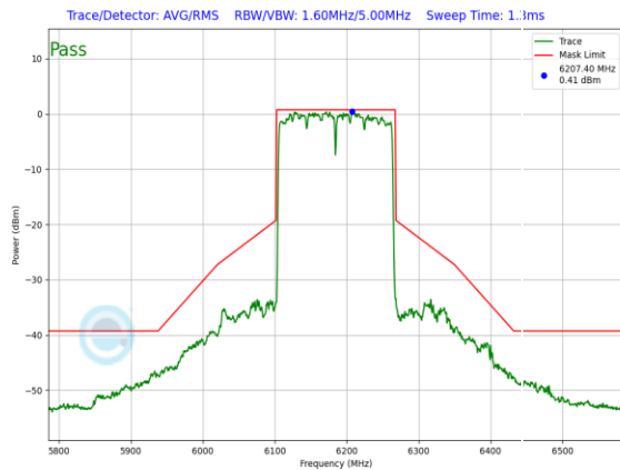
Plot 7-759. In-Band Emission Plot CDD Antenna WF8 Standard Power (160MHz 802.11ax (UNII Band 5) – Ch. 47, MCS11)
