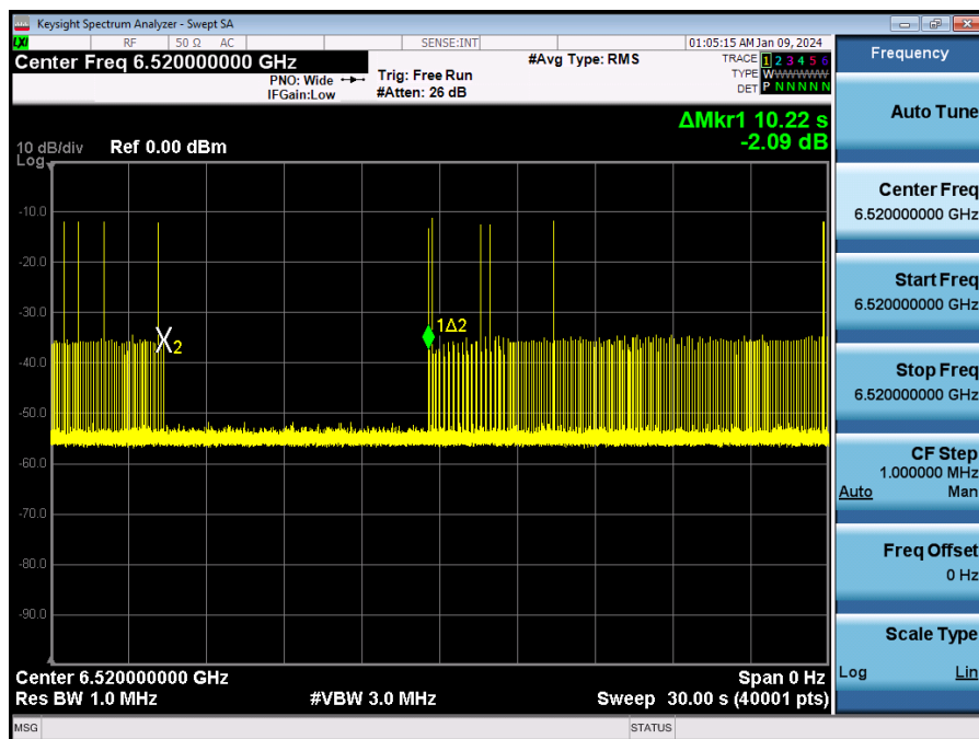
Plot 7-792. Contention Based Protocol Timing Plot – UNII 6 – 160MHz Channel 111 – High
