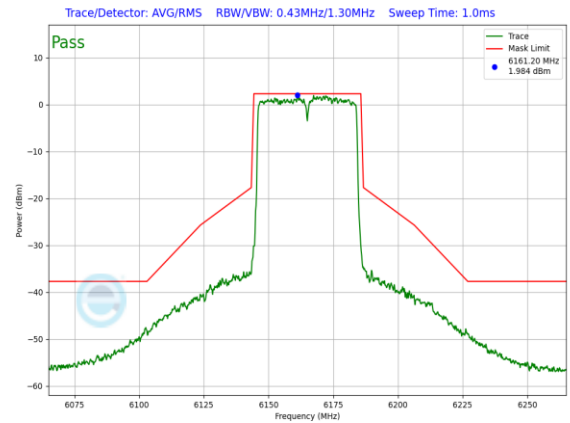
Plot 7-740. In-Band Emission Plot SDM Antenna WF7a Standard Power (40MHz 802.11ax (UNII Band 5) – Ch. 43, MCS4)
