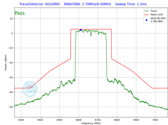
Plot 7-767. In-Band Emission Plot CDD Antenna WF8 Standard Power (160MHz 802.11ax (UNII Band 7) – Ch. 143, MCS11)
