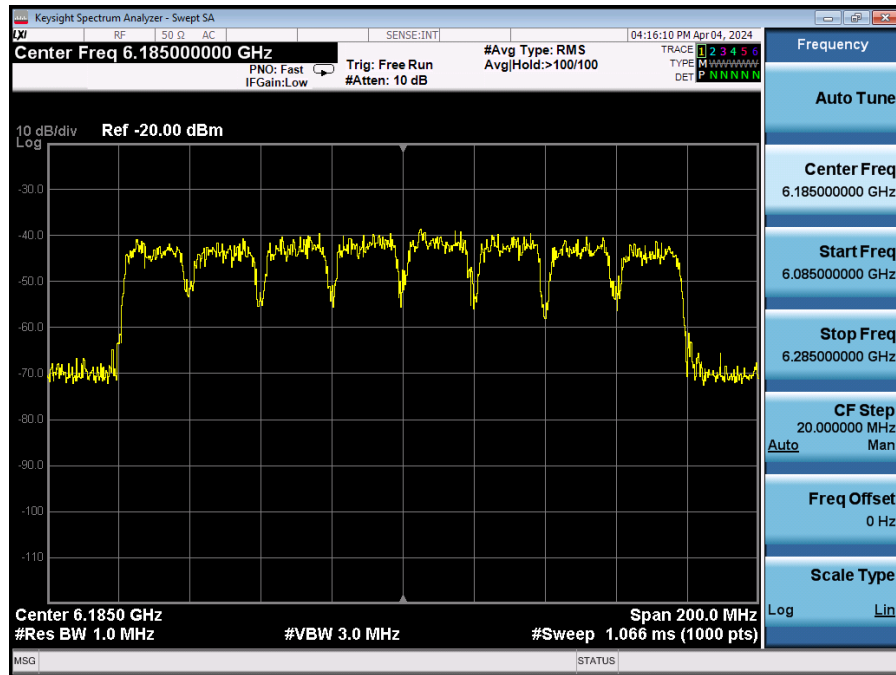
Plot 7-801. 160MHz Bandwidth – Before AWGN Signal Injected – Channel 47
