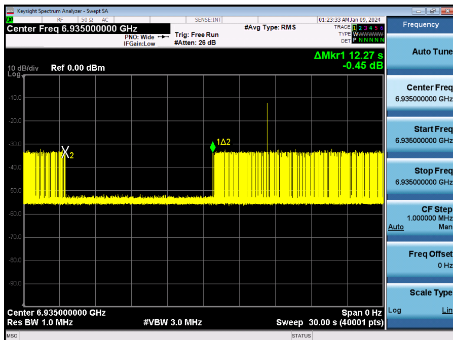
Plot 7-797. Contention Based Protocol Timing Plot – UNII 8 – 20MHz Channel 197
