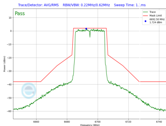
Plot 7-745. In-Band Emission Plot SDM Antenna WF8 Standard Power (20MHz 802.11ax (UNII Band 7) – Ch. 149, MCS4)
