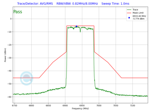
Plot 7-717. In-Band Emission Plot SDM Antenna WF8 Low Power Indoor (80MHz 802.11ax (UNII Band 8) – Ch. 199, MCS11)
