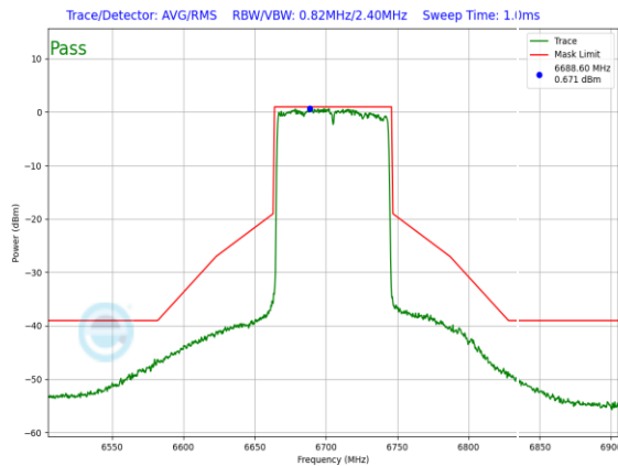
Plot 7-734. In-Band Emission Plot CDD Antenna WF7a Standard Power (80MHz 802.11ax (UNII Band 7) – Ch. 151, MCS2)
