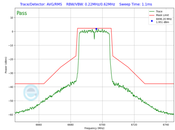
Plot 7-762. In-Band Emission Plot SDM Antenna WF7a Standard Power (20MHz 802.11ax (UNII Band 7) – Ch. 149, MCS11)
