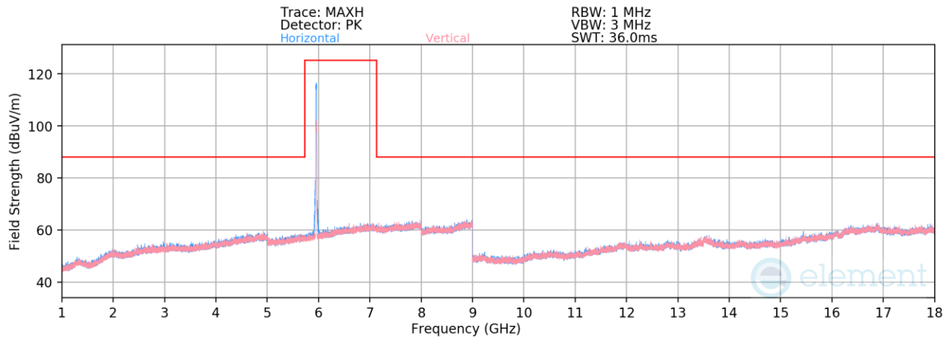
Plot 7-805. Radiated Spurious Emissions above 1GHz Antenna WF8 (802.11ax – Ch. 1)
