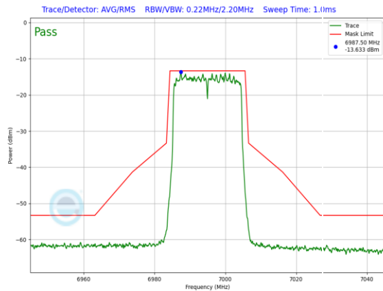
Plot 7-714. In-Band Emission Plot SDM Antenna WF7a Low Power Indoor (20MHz 802.11ax (UNII Band 8) – Ch. 209, MCS11)
