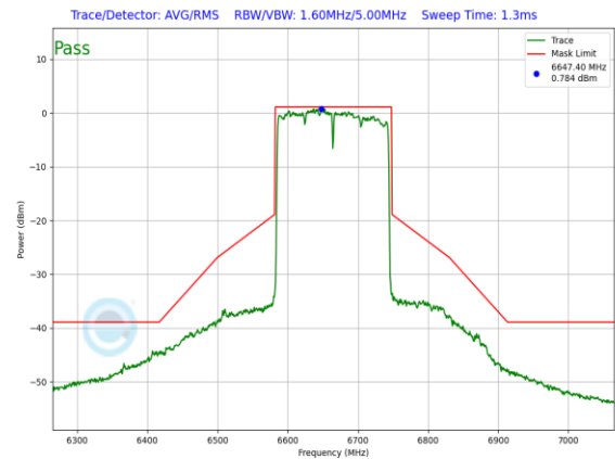
Plot 7-751. In-Band Emission Plot CDD Antenna WF8 Standard Power (160MHz 802.11ax (UNII Band 7) – Ch. 143, MCS4)
