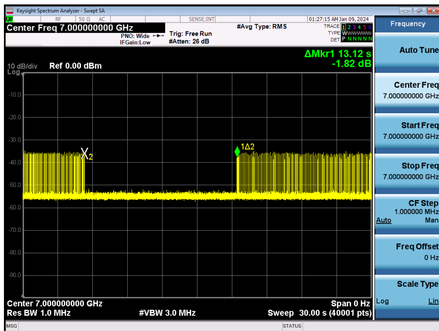
Plot 7-798. Contention Based Protocol Timing Plot – UNII 8 – 160MHz Channel 207 – Low
