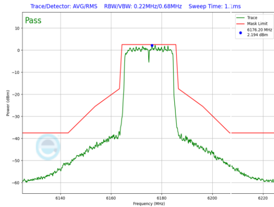
Plot 7-753. In-Band Emission Plot SDM Antenna WF8 Standard Power (20MHz 802.11ax (UNII Band 5) – Ch. 45, MCS11)
