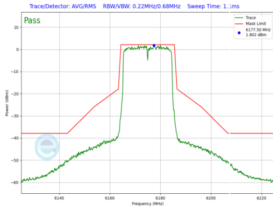
Plot 7-737. In-Band Emission Plot SDM Antenna WF8 Standard Power (20MHz 802.11ax (UNII Band 5) – Ch. 45, MCS4)
