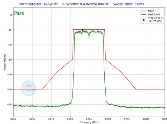
Plot 7-707. In-Band Emission Plot SDM Antenna WF8 Low Power Indoor (40MHz 802.11ax (UNII Band 7) – Ch. 155, MCS11)
