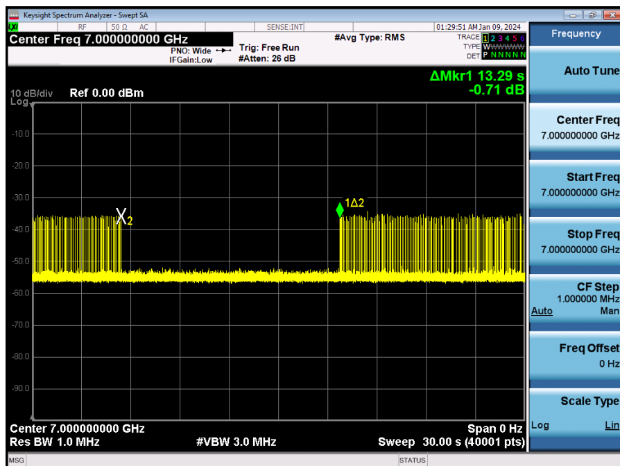
Plot 7-799. Contention Based Protocol Timing Plot – UNII 8 – 160MHz Channel 207 – Mid
