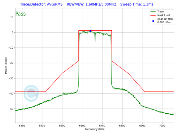
Plot 7-736. In-Band Emission Plot CDD Antenna WF7a Standard Power (160MHz 802.11ax (UNII Band 7) – Ch. 143, MCS2)
