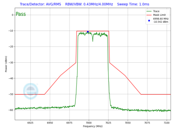
Plot 7-716. In-Band Emission Plot SDM Antenna WF7a Low Power Indoor (40MHz 802.11ax (UNII Band 8) – Ch. 211, MCS11)
