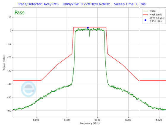
Plot 7-738. In-Band Emission Plot SDM Antenna WF7a Standard Power (20MHz 802.11ax (UNII Band 5) – Ch. 45, MCS4)
