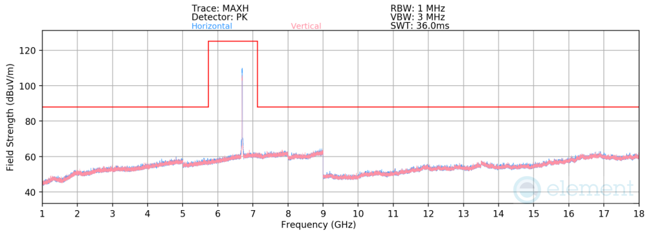
Plot 7-812. Radiated Spurious Emissions above 1GHz Antenna WF8 (802.11ax – Ch. 149, MCS0)
