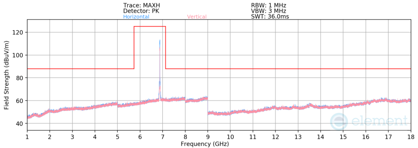
Plot 7-813. Radiated Spurious Emissions above 1GHz Antenna WF8 (802.11ax – Ch. 185)
