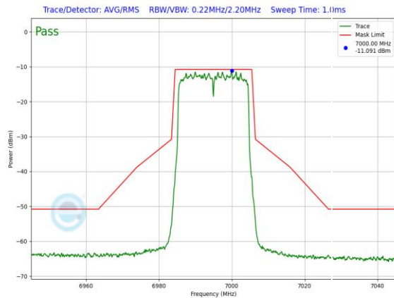
Plot 7-713. In-Band Emission Plot SDM Antenna WF8 Low Power Indoor (20MHz 802.11ax (UNII Band 8) – Ch. 209, MCS11)
