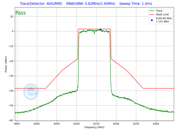
Plot 7-725. In-Band Emission Plot CDD Antenna WF8 Standard Power (80MHz 802.11ax (UNII Band 5) – Ch. 39, MCS2)
