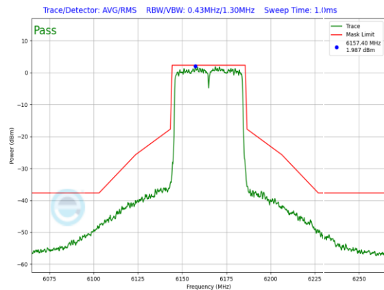
Plot 7-755. In-Band Emission Plot SDM Antenna WF8 Standard Power (40MHz 802.11ax (UNII Band 5) – Ch. 43, MCS11)
