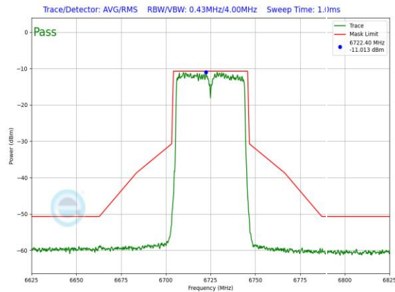
Plot 7-708. In-Band Emission Plot SDM Antenna WF7a Low Power Indoor (40MHz 802.11ax (UNII Band 7) – Ch. 155, MCS11)
