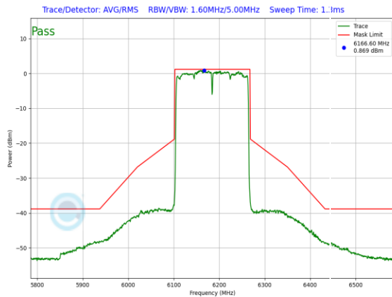
Plot 7-728. In-Band Emission Plot CDD Antenna WF7a Standard Power (160MHz 802.11ax (UNII Band 5) – Ch. 47, MCS2)
