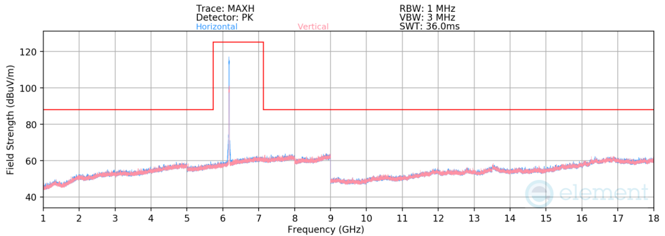
Plot 7-806. Radiated Spurious Emissions above 1GHz Antenna WF8 (802.11ax – Ch. 45, MCS0)
