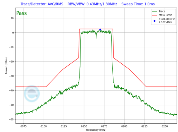
Plot 7-756. In-Band Emission Plot SDM Antenna WF7a Standard Power (40MHz 802.11ax (UNII Band 5) – Ch. 43, MCS11)
