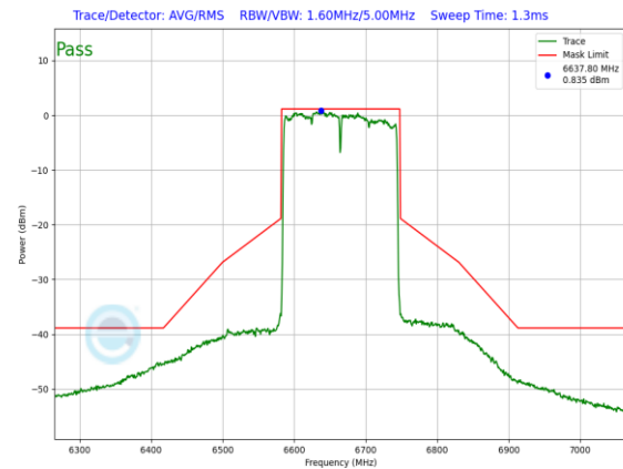
Plot 7-735. In-Band Emission Plot CDD Antenna WF8 Standard Power (160MHz 802.11ax (UNII Band 7) – Ch. 143, MCS2)
