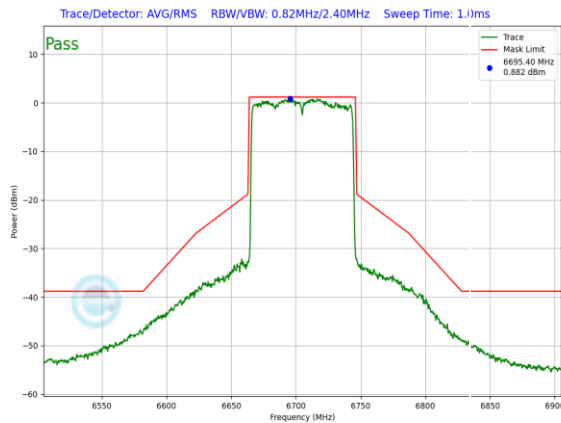
Plot 7-750. In-Band Emission Plot CDD Antenna WF7a Standard Power (80MHz 802.11ax (UNII Band 7) – Ch. 151, MCS4)
