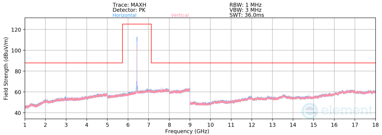
Plot 7-808. Radiated Spurious Emissions above 1GHz Antenna WF8 (802.11ax – Ch. 97)
