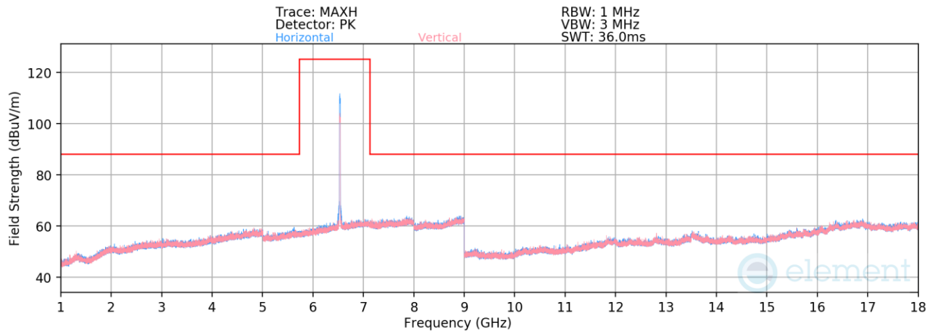
Plot 7-811. Radiated Spurious Emissions above 1GHz Antenna WF8 (802.11ax – Ch. 117)
