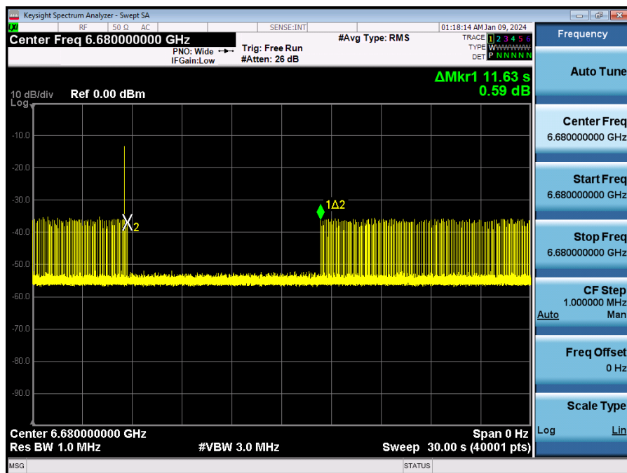
Plot 7-796. Contention Based Protocol Timing Plot – UNII 7 – 160MHz Channel 143 – High
