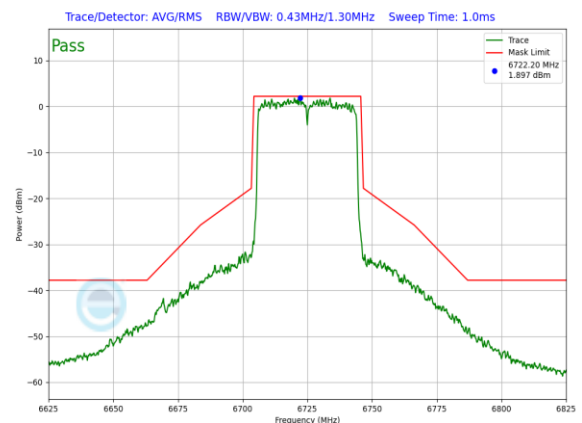
Plot 7-764. In-Band Emission Plot CDD Antenna WF7a Standard Power (40MHz 802.11ax (UNII Band 7) – Ch. 155, MCS11)
