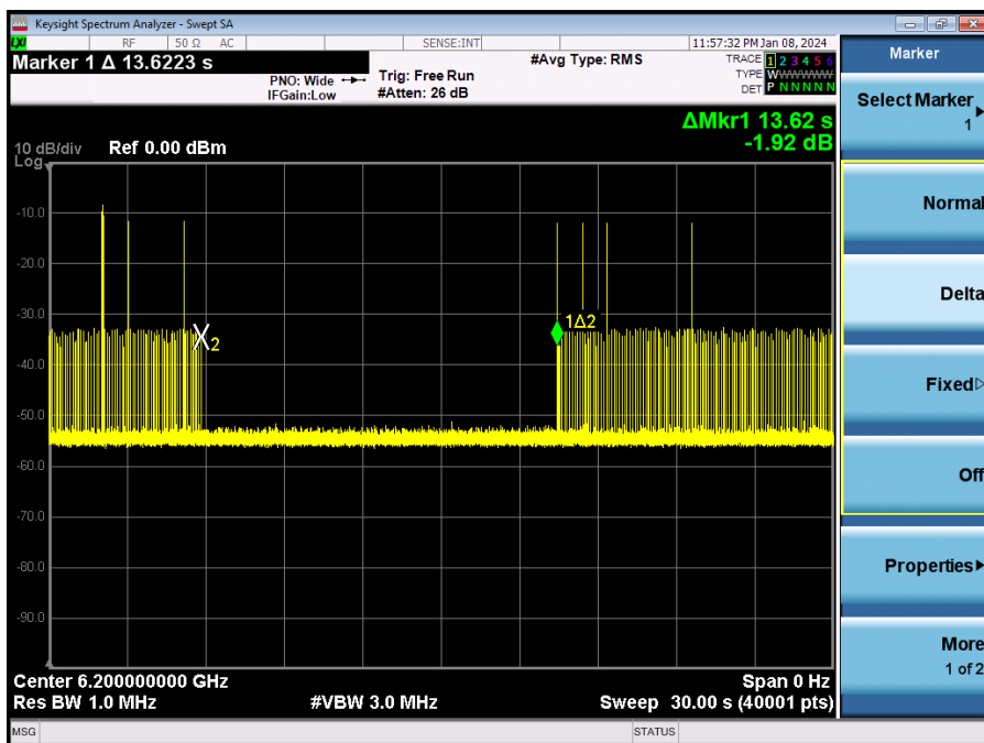
Plot 7-788. Contention Based Protocol Timing Plot – UNII 5 – 160MHz Channel 47 – High
