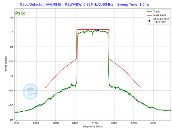
Plot 7-742. In-Band Emission Plot CDD Antenna WF7a Standard Power (80MHz 802.11ax (UNII Band 5) – Ch. 39, MCS4)
