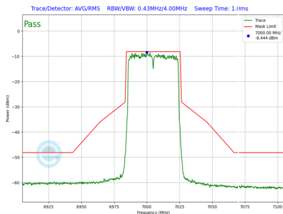
Plot 7-715. In-Band Emission Plot SDM Antenna WF8 Low Power Indoor (40MHz 802.11ax (UNII Band 8) – Ch. 211, MCS11)
