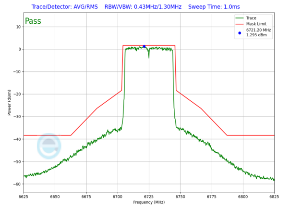
Plot 7-747. In-Band Emission Plot CDD Antenna WF8 Standard Power (40MHz 802.11ax (UNII Band 7) – Ch. 155, MCS4)
