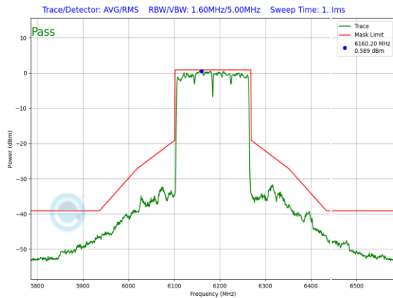
Plot 7-760. In-Band Emission Plot CDD Antenna WF7a Standard Power (160MHz 802.11ax (UNII Band 5) – Ch. 47, MCS11)
