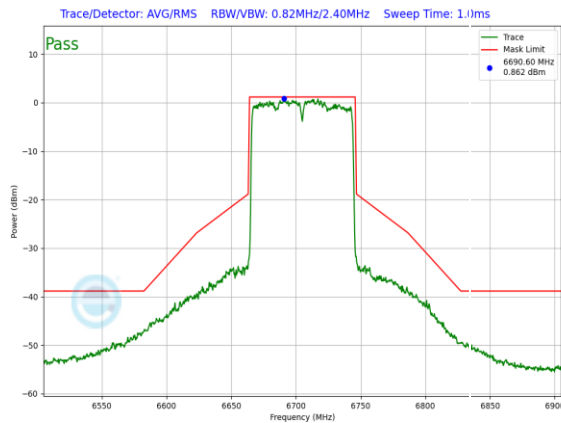
Plot 7-766. In-Band Emission Plot CDD Antenna WF7a Standard Power (80MHz 802.11ax (UNII Band 7) – Ch. 151, MCS11)
