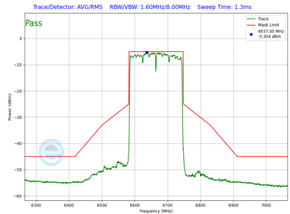
Plot 7-711. In-Band Emission Plot SDM Antenna WF8 Low Power Indoor (160MHz 802.11ax (UNII Band 7) – Ch. 143, MCS11)
