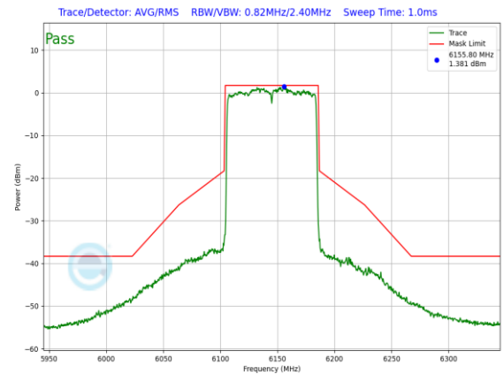
Plot 7-741. In-Band Emission Plot CDD Antenna WF8 Standard Power (80MHz 802.11ax (UNII Band 5) – Ch. 39, MCS4)
