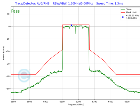
Plot 7-744. In-Band Emission Plot CDD Antenna WF7a Standard Power (160MHz 802.11ax (UNII Band 5) – Ch. 47, MCS4)
