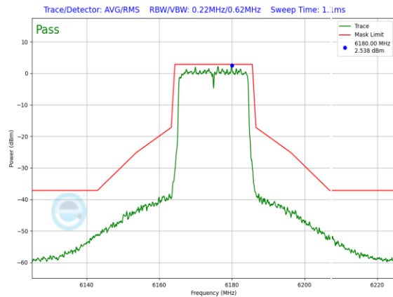
Plot 7-754. In-Band Emission Plot SDM Antenna WF7a Standard Power (20MHz 802.11ax (UNII Band 5) – Ch. 45, MCS11)
