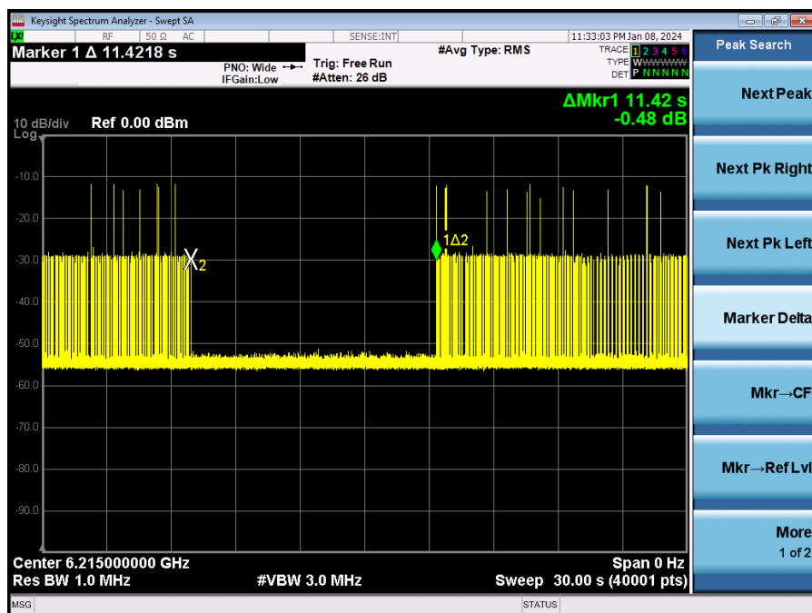
Plot 7-785. Contention Based Protocol Timing Plot – UNII 5 – 20MHz Channel 53
