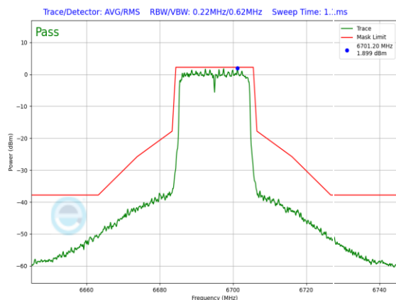
Plot 7-761. In-Band Emission Plot SDM Antenna WF8 Standard Power (20MHz 802.11ax (UNII Band 7) – Ch. 149, MCS11)
