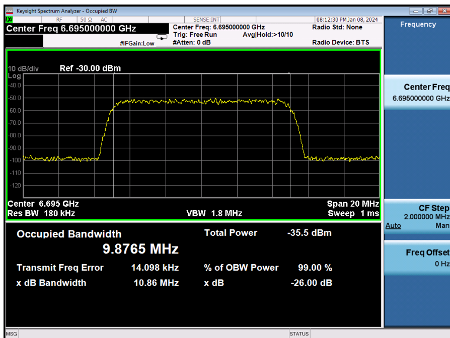
Plot 7-777. AWGN Signal – UNII 7 – 20MHz
