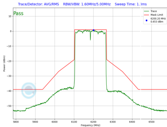
Plot 7-727. In-Band Emission Plot CDD Antenna WF8 Standard Power (160MHz 802.11ax (UNII Band 5) – Ch. 47, MCS2)
