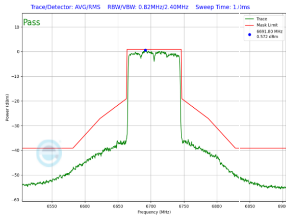
Plot 7-765. In-Band Emission Plot CDD Antenna WF8 Standard Power (80MHz 802.11ax (UNII Band 7) – Ch. 151, MCS11)
