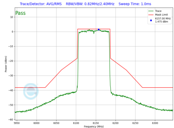
Plot 7-726. In-Band Emission Plot CDD Antenna WF7a Standard Power (80MHz 802.11ax (UNII Band 5) – Ch. 39, MCS2)
