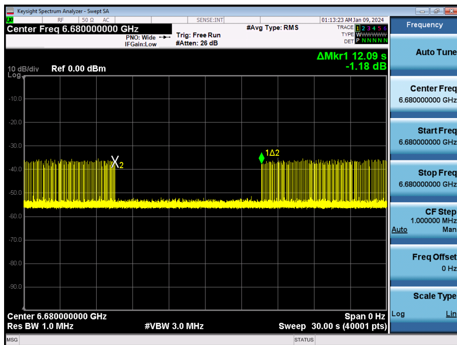
Plot 7-794. Contention Based Protocol Timing Plot – UNII 7 – 160MHz Channel 143 – Low
