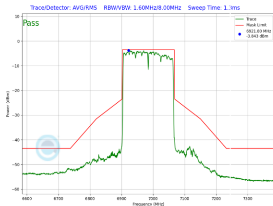
Plot 7-719. In-Band Emission Plot SDM Antenna WF8 Low Power Indoor (160MHz 802.11ax (UNII Band 8) – Ch. 207, MCS11)
