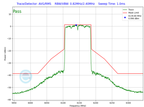
Plot 7-758. In-Band Emission Plot CDD Antenna WF7a Standard Power (80MHz 802.11ax (UNII Band 5) – Ch. 39, MCS11)
