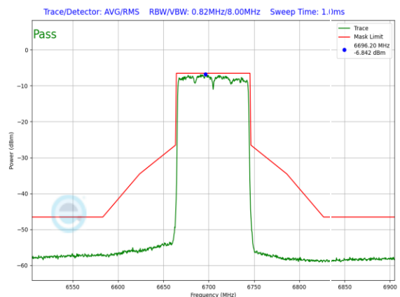
Plot 7-709. In-Band Emission Plot SDM Antenna WF8 Low Power Indoor (80MHz 802.11ax (UNII Band 7) – Ch. 151, MCS11)
