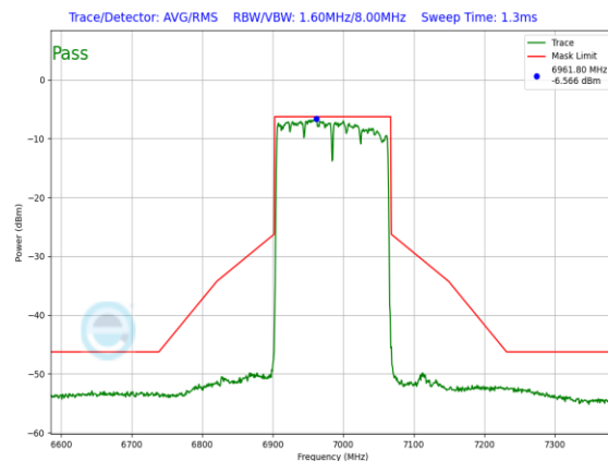
Plot 7-720. In-Band Emission Plot SDM Antenna WF7a Low Power Indoor (160MHz 802.11ax (UNII Band 8) – Ch. 207, MCS11)
