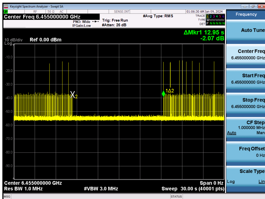
Plot 7-789. Contention Based Protocol Timing Plot – UNII 6 – 20MHz Channel 101
