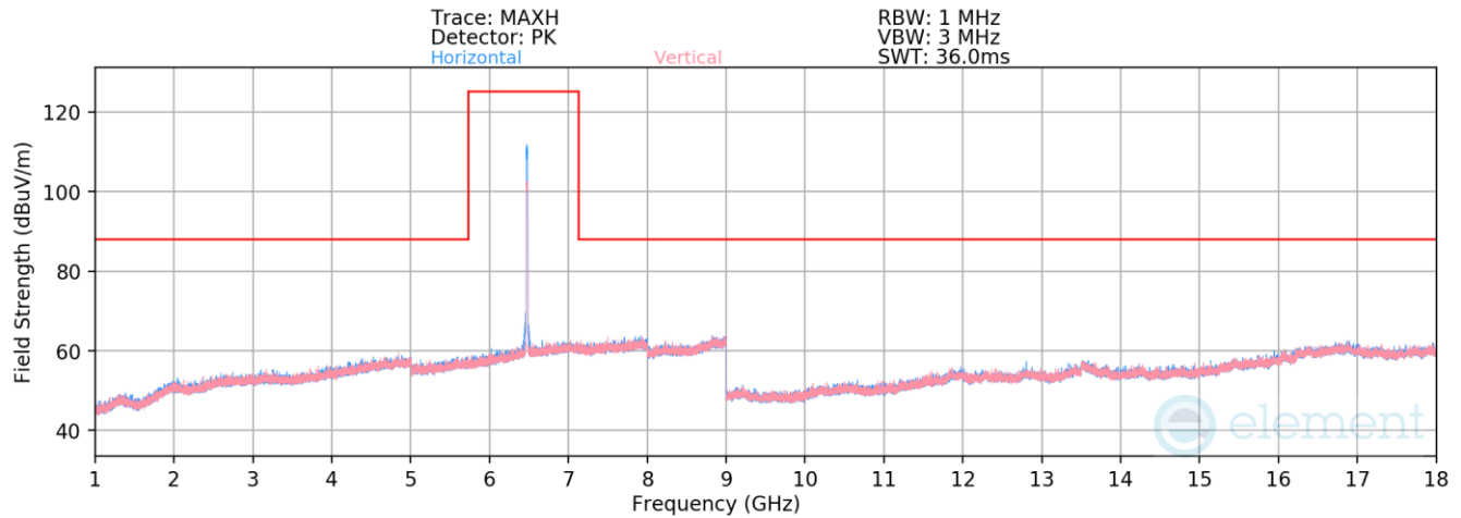
Plot 7-809. Radiated Spurious Emissions above 1GHz Antenna WF8 (802.11ax – Ch. 105, MCS0)
