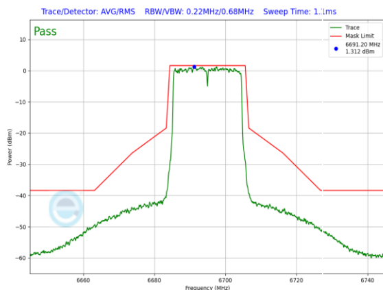
Plot 7-729. In-Band Emission Plot SDM Antenna WF8 Standard Power (20MHz 802.11ax (UNII Band 7) – Ch. 149, MCS2)
