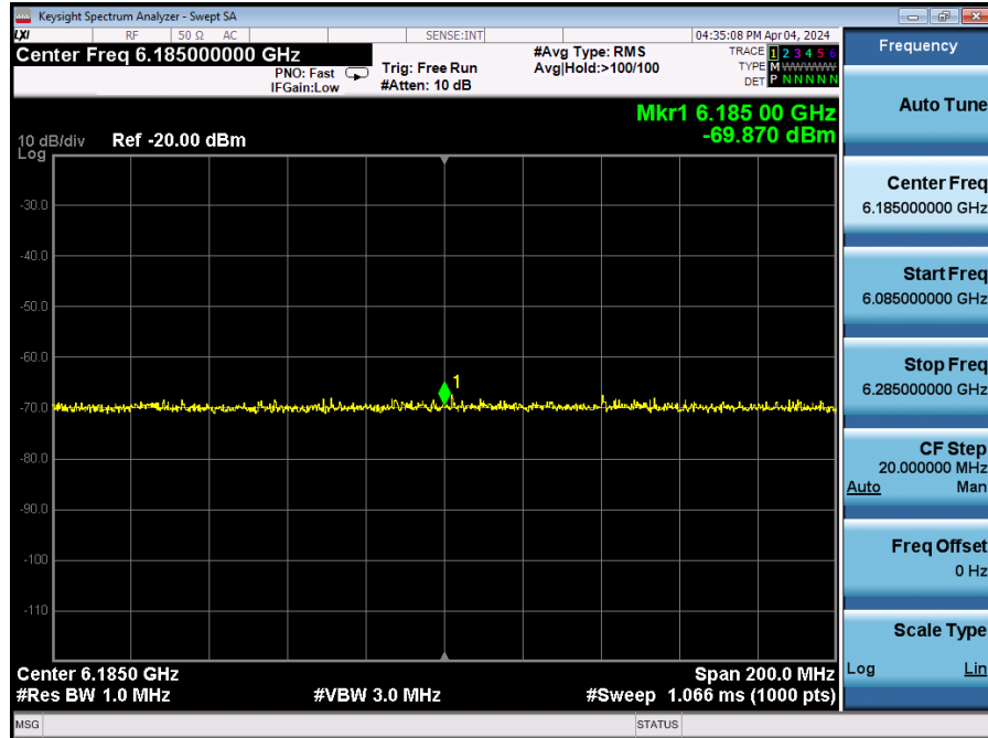
Plot 7-803. 160MHz Bandwidth – AWGN Signal Injected at Center – Channel 47
