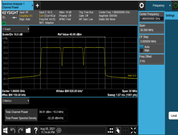
Plot 7-355. Conducted Average Output Power Plot (B2_5M+5M+5M_3C_256QAM - Mid Channel, Port 2)
