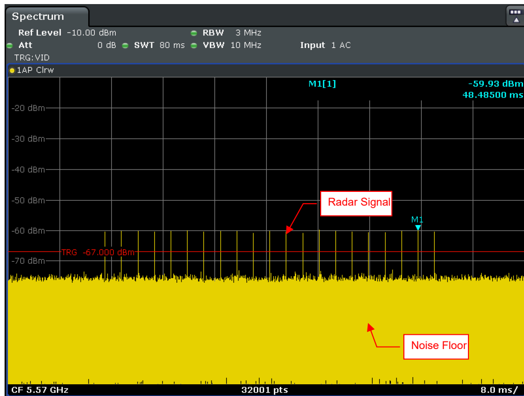
Radar Signal 1 (Test A)
