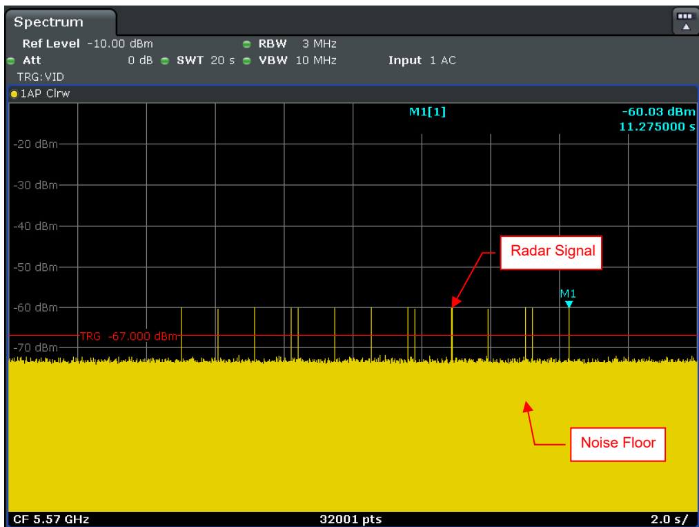
Single Burst of Radar Signal 4
