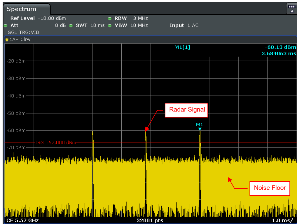
Single Burst of Radar Signal 5
