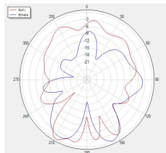
Phi=0 freq=2450MHz
