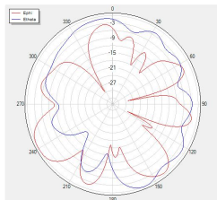
Phi=90 freq=2450MHz
