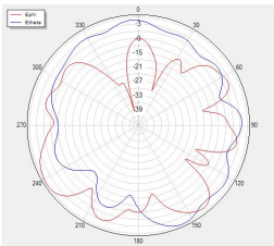
Phi=90 freq=2400MHz
