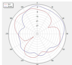
Theta=90 freq=2450MHz
