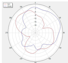
Theta=90 freq=2480MHz
