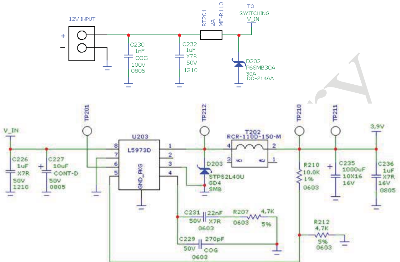
Switching regulator
