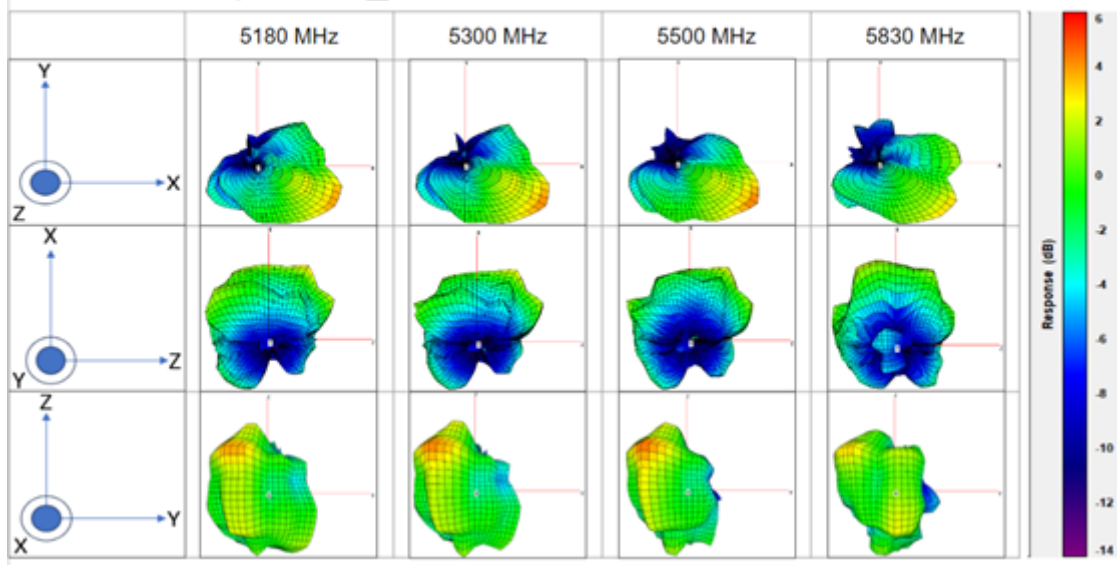
Radiation pattern _ ANT1
