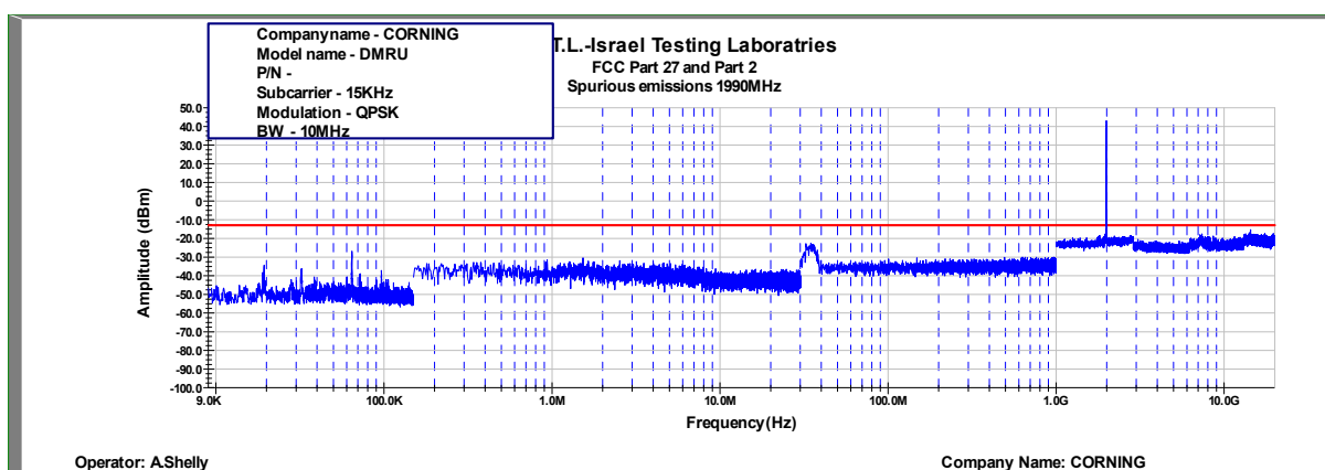
Figure 445: Spurious Emissions at Antenna Terminal QPSK, 1990MHz, B.W. 10MHz, Sub Carrier 15kHz
