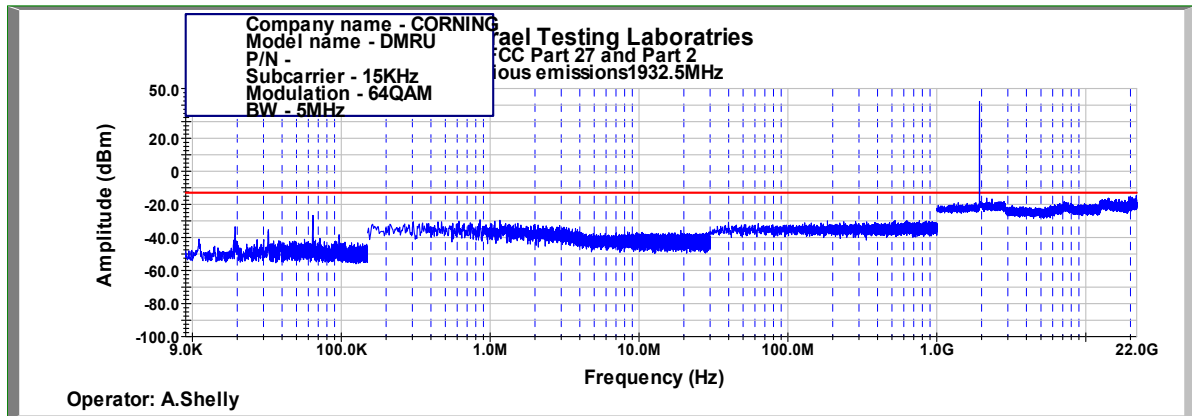
Figure 401: Spurious Emissions at Antenna Terminal 64QAM, 1932.5MHz, B.W. 5MHz, Sub Carrier 15kHz
