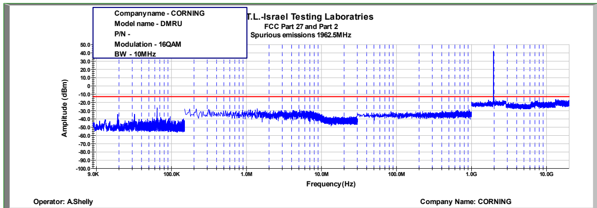
Figure 390: Spurious Emissions at Antenna Terminal 16QAM, 1962.5MHz, B.W. 10MHz, Sub Carrier 15kHz
