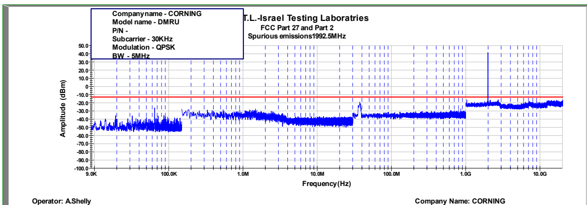
Figure 442: Spurious Emissions at Antenna Terminal QPSK, 1992.5MHz, B.W. 5MHz, Sub Carrier 30kHz
