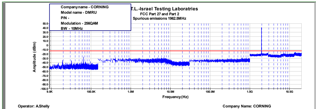
Figure 426: Spurious Emissions at Antenna Terminal 256QAM, 1962.5MHz, B.W. 10MHz, Sub Carrier 15kHz
