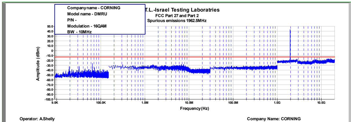
Figure 393: Spurious Emissions at Antenna Terminal 16QAM, 1962.5MHz, B.W. 10MHz, Sub Carrier 30kHz
