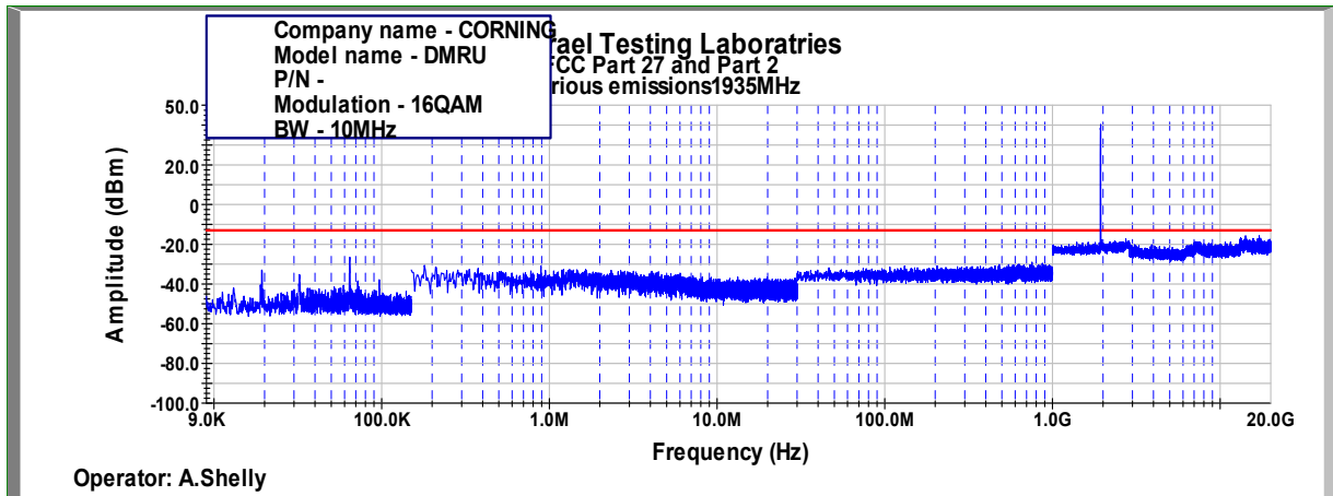
Figure 389: Spurious Emissions at Antenna Terminal 16QAM, 1935MHz, B.W. 10MHz, Sub Carrier 15kHz
