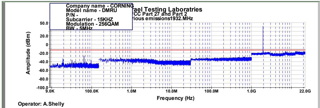
Figure 419: Spurious Emissions at Antenna Terminal 256QAM, 1932.5MHz, B.W. 5MHz, Sub Carrier 15kHz
