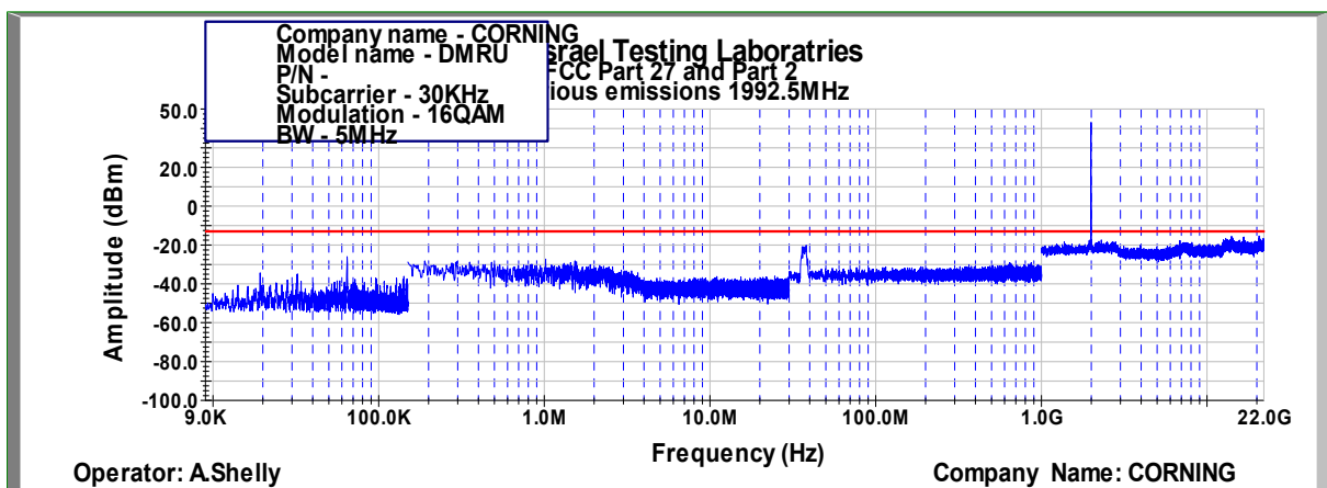
Figure 388: Spurious Emissions at Antenna Terminal 16QAM, 1992.5MHz, B.W. 5MHz, Sub Carrier 30kHz
