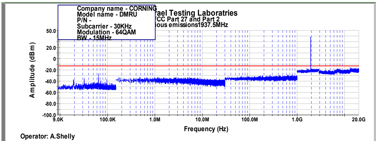
Figure 416: Spurious Emissions at Antenna Terminal 64QAM, 1937.5MHz, B.W. 15MHz, Sub Carrier 30kHz
