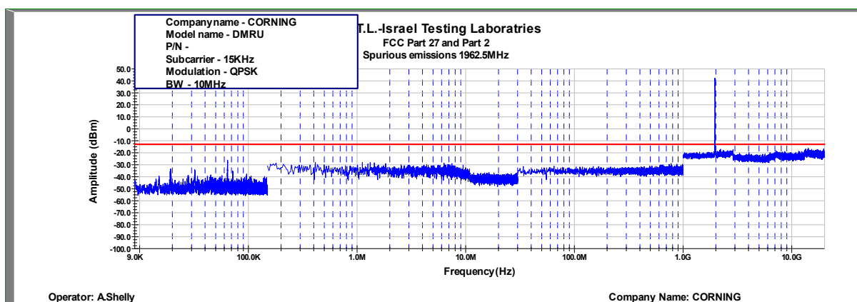
Figure 444: Spurious Emissions at Antenna Terminal QPSK, 1962.5MHz, B.W. 10MHz, Sub Carrier 15kHz
