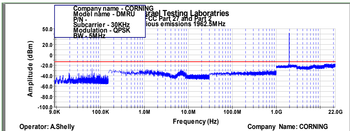
Figure 441: Spurious Emissions at Antenna Terminal QPSK, 1962.5MHz, B.W. 5MHz, Sub Carrier 30kHz
