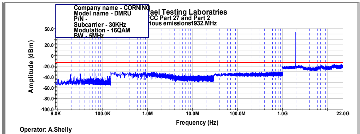
Figure 386: Spurious Emissions at Antenna Terminal 16QAM, 1932.5MHz, B.W. 5MHz, Sub Carrier 30kHz
