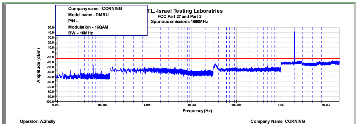
Figure 391: Spurious Emissions at Antenna Terminal 16QAM, 1990MHz, B.W. 10MHz, Sub Carrier 15kHz
