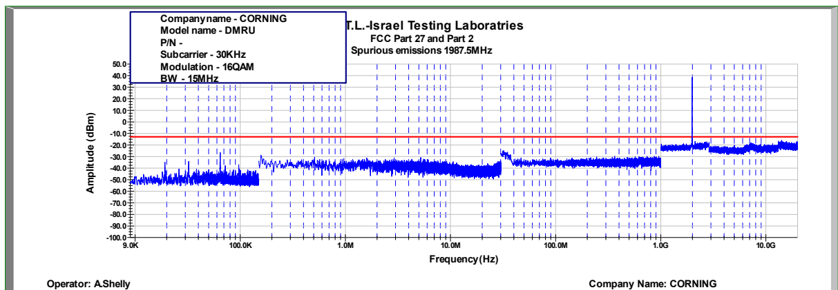
Figure 400: Spurious Emissions at Antenna Terminal 16QAM, 1987.5MHz, B.W. 15MHz, Sub Carrier 30kHz
