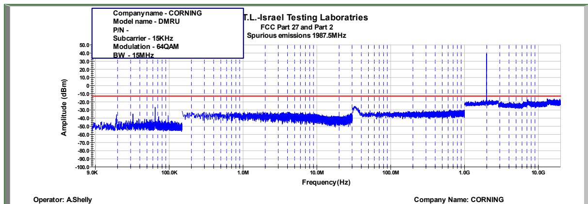
Figure 415: Spurious Emissions at Antenna Terminal 64QAM, 1987.5MHz, B.W. 15MHz, Sub Carrier 15kHz
