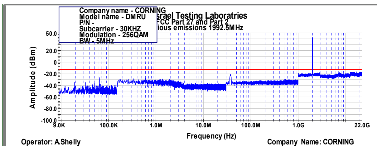
Figure 424: Spurious Emissions at Antenna Terminal 256QAM, 1992.5MHz, B.W. 5MHz, Sub Carrier 30kHz
