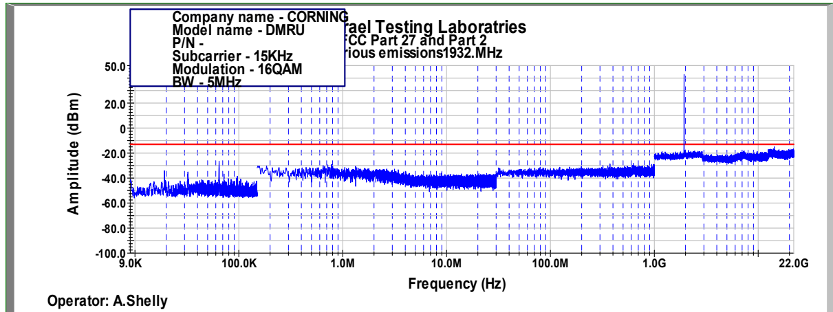
Figure 383: Spurious Emissions at Antenna Terminal 16QAM, 1932.5MHz, B.W. 5MHz, Sub Carrier 15kHz
