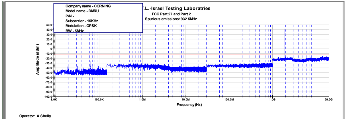
Figure 437: Spurious Emissions at Antenna Terminal QPSK, 1932.5MHz, B.W. 5MHz, Sub Carrier 15kHz
