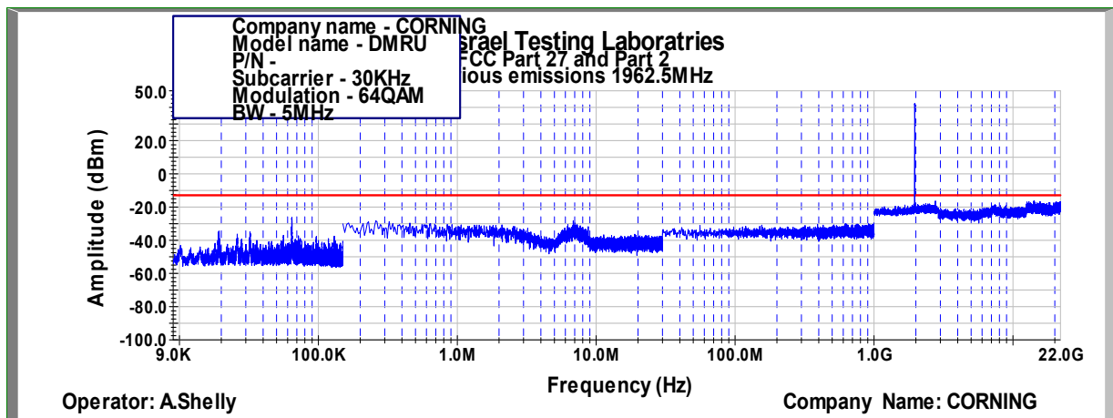
Figure 405: Spurious Emissions at Antenna Terminal 64QAM, 1962.5MHz, B.W. 5MHz, Sub Carrier 30kHz
