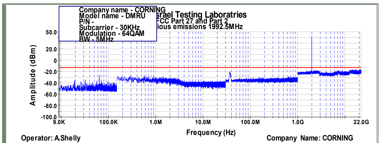
Figure 406: Spurious Emissions at Antenna Terminal 64QAM, 1992.5MHz, B.W. 5MHz, Sub Carrier 30kHz
