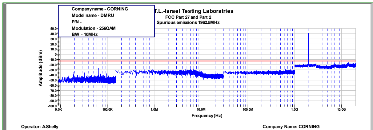
Figure 429: Spurious Emissions at Antenna Terminal 256QAM, 1962.5MHz, B.W. 10MHz, Sub Carrier 30kHz
