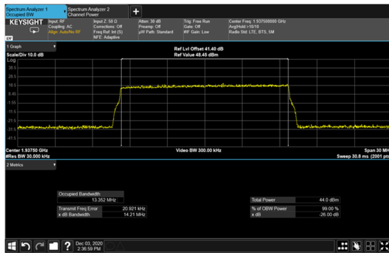
Figure 380: QPSK 15MHz B.W.; 1937.5MHz Output – 4G
