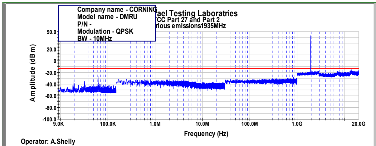
Figure 446: Spurious Emissions at Antenna Terminal QPSK, 1935MHz, B.W. 10MHz, Sub Carrier 30kHz
