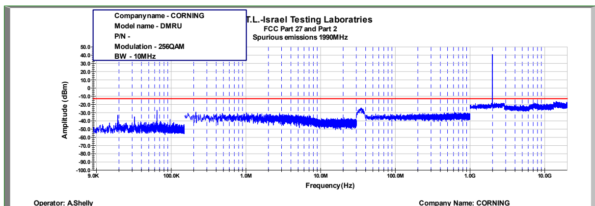
Figure 430: Spurious Emissions at Antenna Terminal 256QAM, 1990MHz, B.W. 10MHz, Sub Carrier 30kHz
