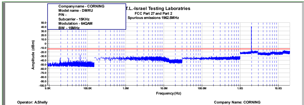
Figure 414: Spurious Emissions at Antenna Terminal 64QAM, 1962.5MHz, B.W. 15MHz, Sub Carrier 15kHz
