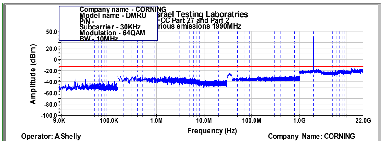
Figure 412: Spurious Emissions at Antenna Terminal 64QAM, 1990MHz, B.W. 10MHz, Sub Carrier 30kHz
