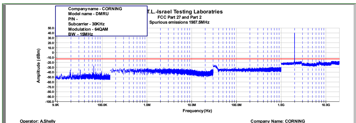
Figure 418: Spurious Emissions at Antenna Terminal 64QAM, 1987.5MHz, B.W. 15MHz, Sub Carrier 30kHz
