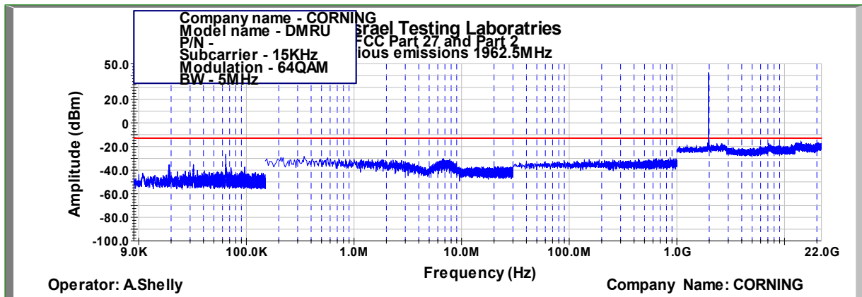
Figure 402: Spurious Emissions at Antenna Terminal 64QAM, 1962.5MHz, B.W. 5MHz, Sub Carrier 15kHz
