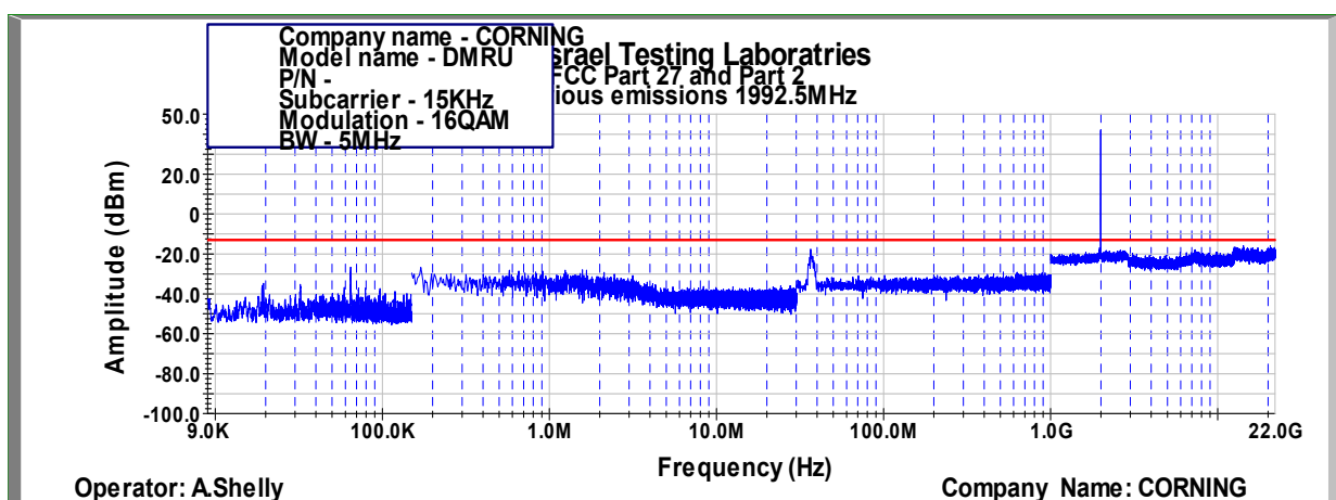
Figure 385: Spurious Emissions at Antenna Terminal 16QAM, 1992.5MHz, B.W. 5MHz, Sub Carrier 15kHz
