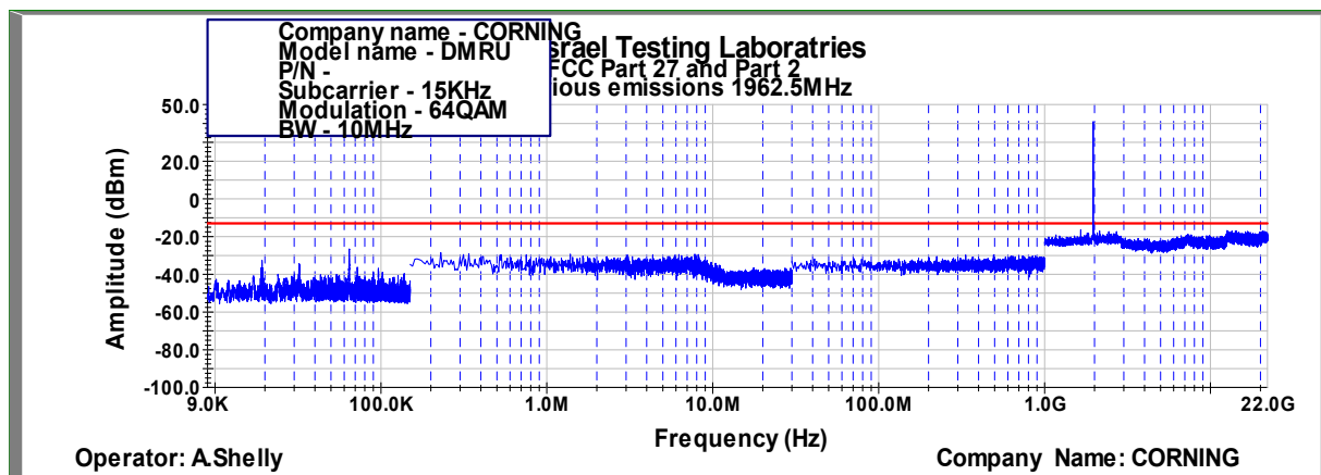
Figure 408: Spurious Emissions at Antenna Terminal 64QAM, 1962.5MHz, B.W. 10MHz, Sub Carrier 15kHz
