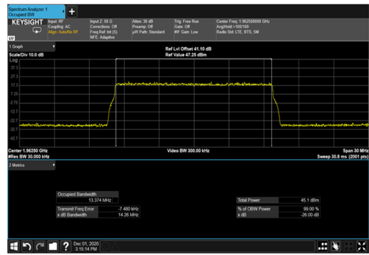
Figure 381: QPSK 15MHz B.W.; 1962.5MHz Output – 4G
