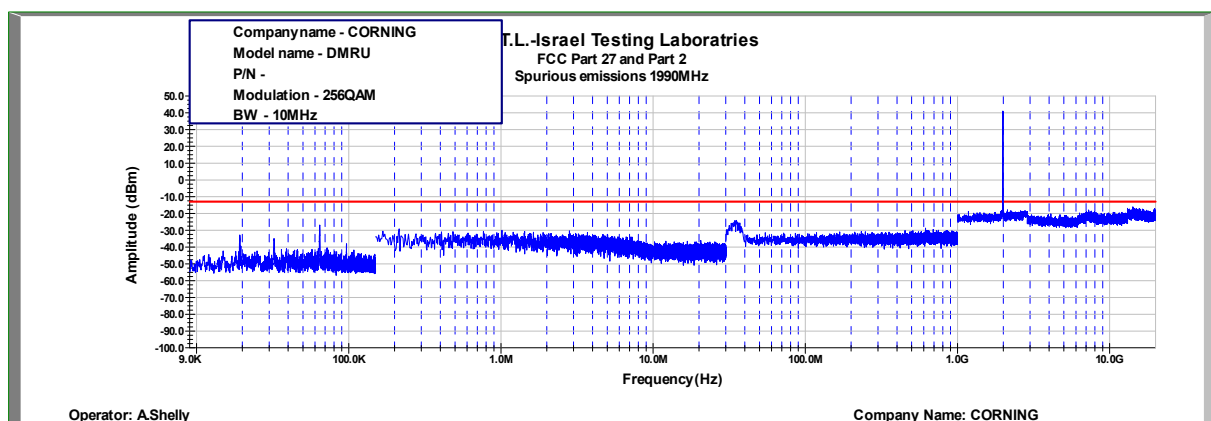
Figure 427: Spurious Emissions at Antenna Terminal 256QAM, 1990MHz, B.W. 10MHz, Sub Carrier 15kHz
