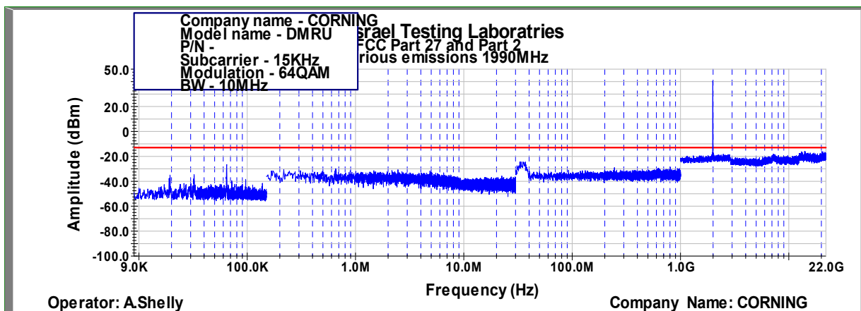
Figure 409: Spurious Emissions at Antenna Terminal 64QAM, 1990MHz, B.W. 10MHz, Sub Carrier 15kHz
