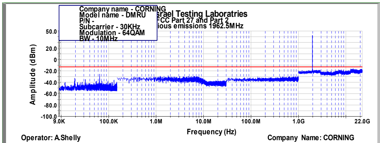
Figure 411: Spurious Emissions at Antenna Terminal 64QAM, 1962.5MHz, B.W. 10MHz, Sub Carrier 30kHz
