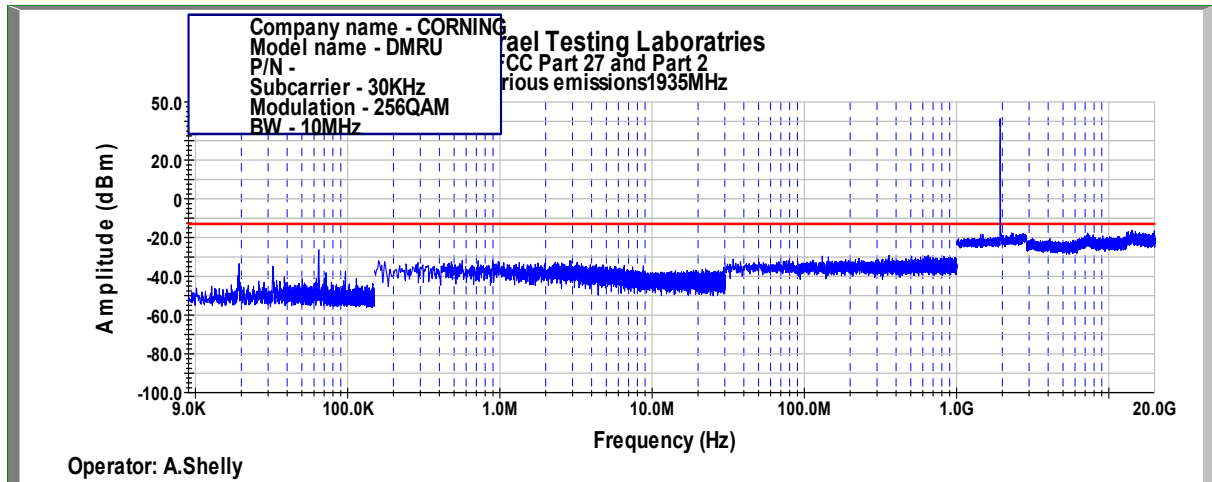
Figure 428: Spurious Emissions at Antenna Terminal 256QAM, 1935MHz, B.W. 10MHz, Sub Carrier 30kHz
