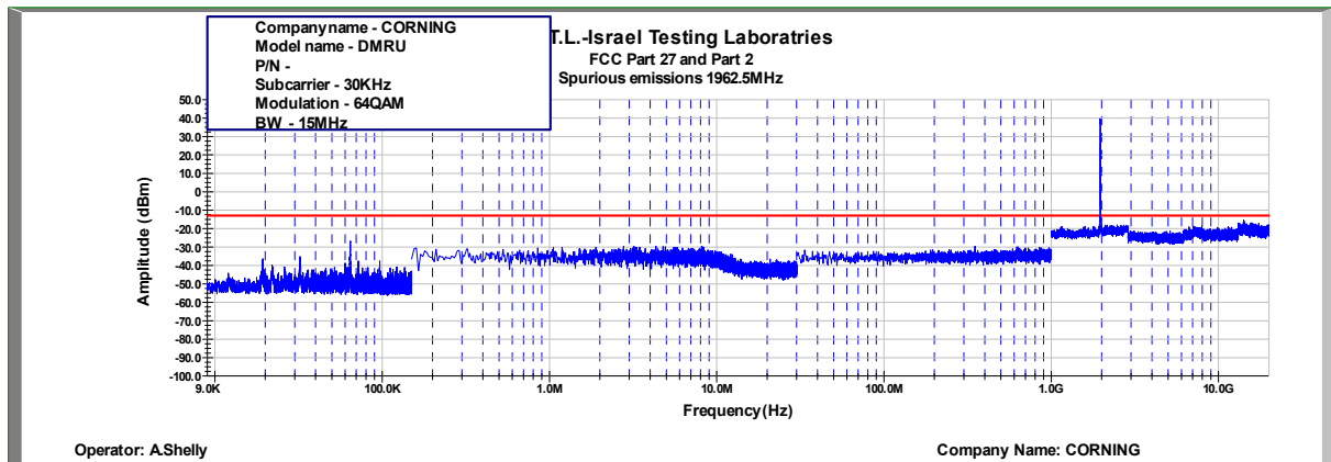
Figure 417: Spurious Emissions at Antenna Terminal 64QAM, 1962.5MHz, B.W. 15MHz, Sub Carrier 30kHz
