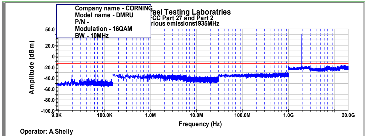
Figure 392: Spurious Emissions at Antenna Terminal 16QAM, 1935MHz, B.W. 10MHz, Sub Carrier 30kHz
