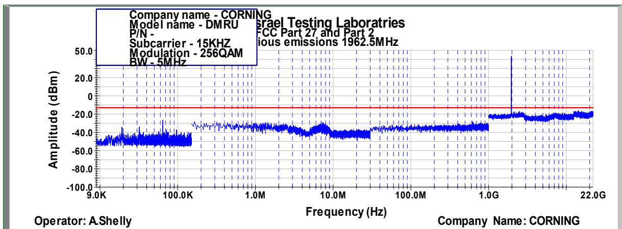
Figure 420: Spurious Emissions at Antenna Terminal 256QAM, 1962.5MHz, B.W. 5MHz, Sub Carrier 15kHz
