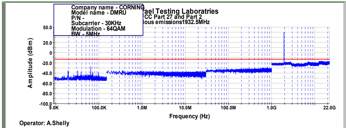
Figure 404: Spurious Emissions at Antenna Terminal 64QAM, 1932.5MHz, B.W. 5MHz, Sub Carrier 30kHz
