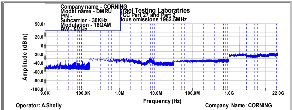
Figure 387: Spurious Emissions at Antenna Terminal 16QAM, 1962.5MHz, B.W. 5MHz, Sub Carrier 30kHz
