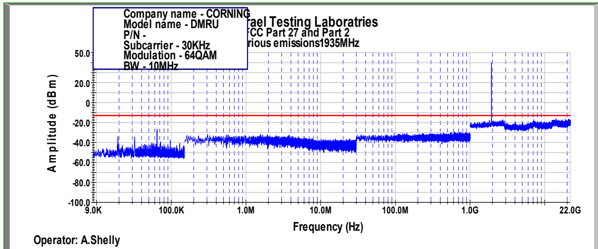
Figure 410: Spurious Emissions at Antenna Terminal 64QAM, 1935MHz, B.W. 10MHz, Sub Carrier 30kHz
