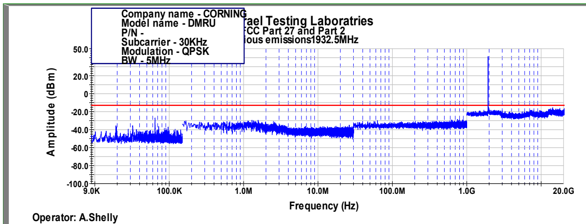
Figure 440: Spurious Emissions at Antenna Terminal QPSK, 1932.5MHz, B.W. 5MHz, Sub Carrier 30kHz
