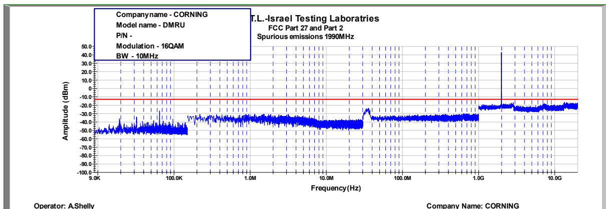
Figure 394: Spurious Emissions at Antenna Terminal 16QAM, 1990MHz, B.W. 10MHz, Sub Carrier 30kHz
