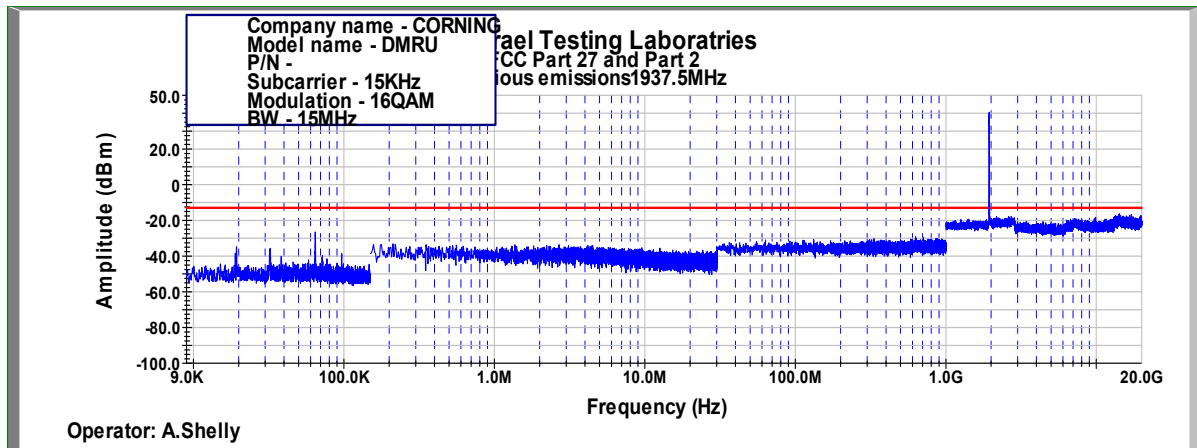
Figure 395: Spurious Emissions at Antenna Terminal 16QAM, 1937.5MHz, B.W. 15MHz, Sub Carrier 15kHz
