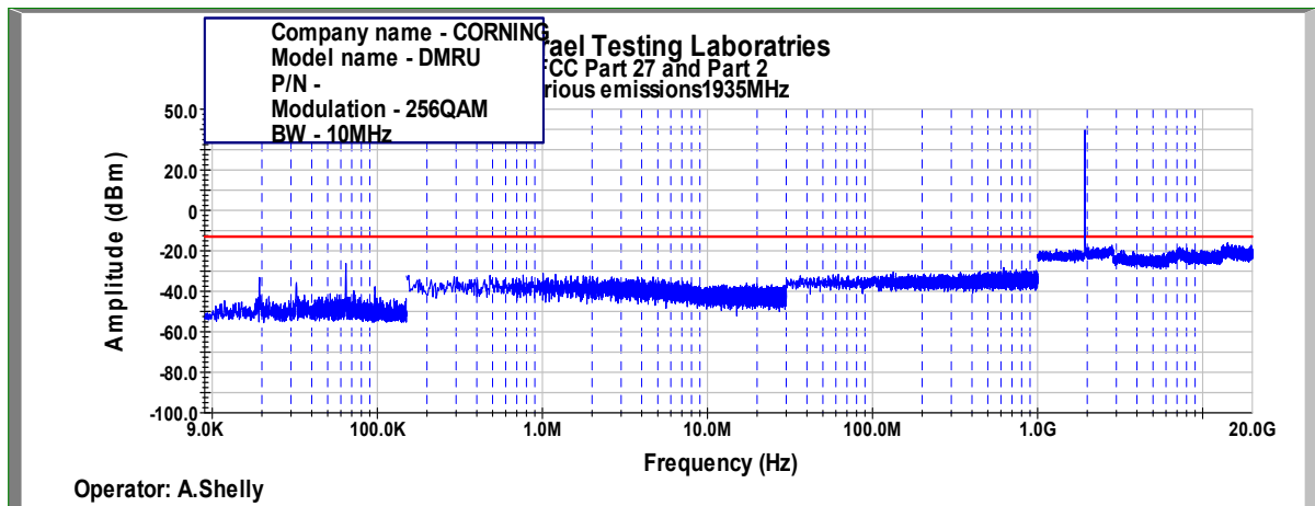
Figure 425: Spurious Emissions at Antenna Terminal 256QAM, 1935MHz, B.W. 10MHz, Sub Carrier 15kHz
