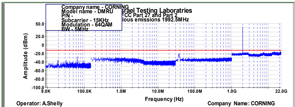
Figure 403: Spurious Emissions at Antenna Terminal 64QAM, 1992.5MHz, B.W. 5MHz, Sub Carrier 15kHz
