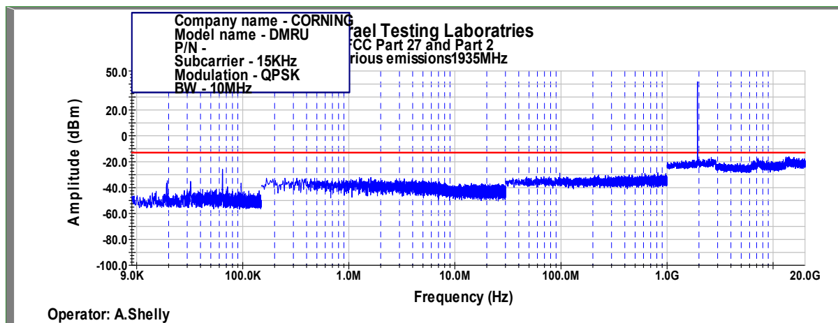
Figure 443: Spurious Emissions at Antenna Terminal QPSK, 1935MHz, B.W. 10MHz, Sub Carrier 15kHz
