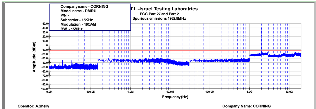
Figure 396: Spurious Emissions at Antenna Terminal 16QAM, 1962.5MHz, B.W. 15MHz, Sub Carrier 15kHz
