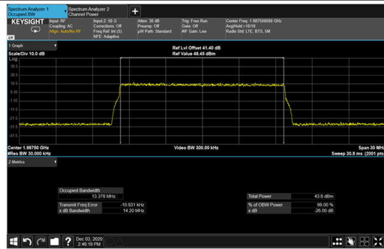
Figure 382: QPSK 15MHz B.W.; 1987.5MHz Output – 4G
