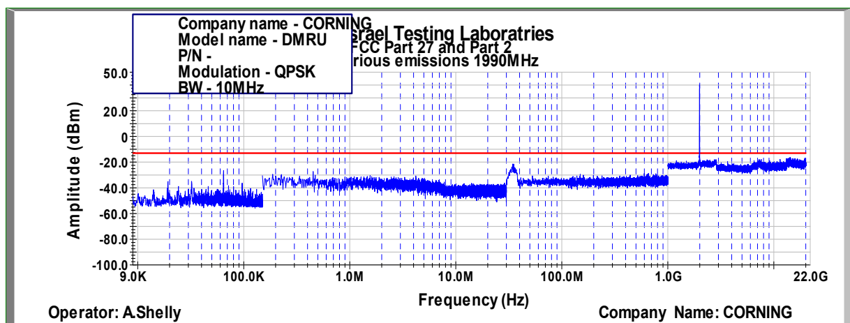
Figure 448: Spurious Emissions at Antenna Terminal QPSK, 1990MHz, B.W. 10MHz, Sub Carrier 30kHz
