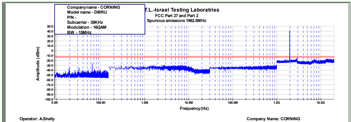
Figure 399: Spurious Emissions at Antenna Terminal 16QAM, 1962.5MHz, B.W. 15MHz, Sub Carrier 30kHz
