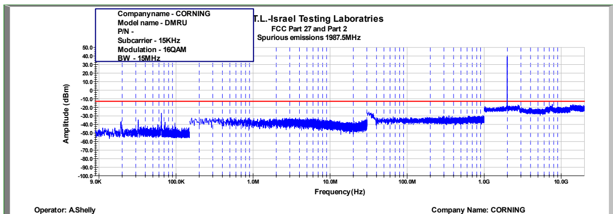
Figure 397: Spurious Emissions at Antenna Terminal 16QAM, 1987.5MHz, B.W. 15MHz, Sub Carrier 15kHz
