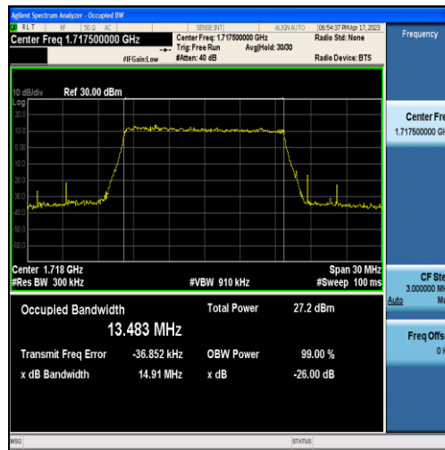
Band66-15MHz-16QAM-132047-75RB#0-13.483
