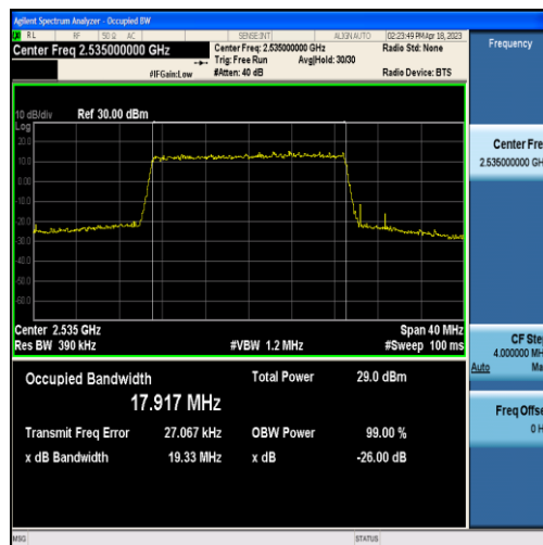
Band7-20MHz-QPSK-21100-100RB#0-17.917
