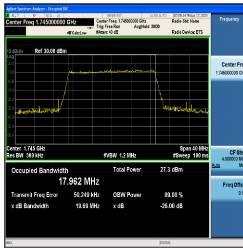
Band66-20MHz-16QAM-132322-100RB#0-17.962
