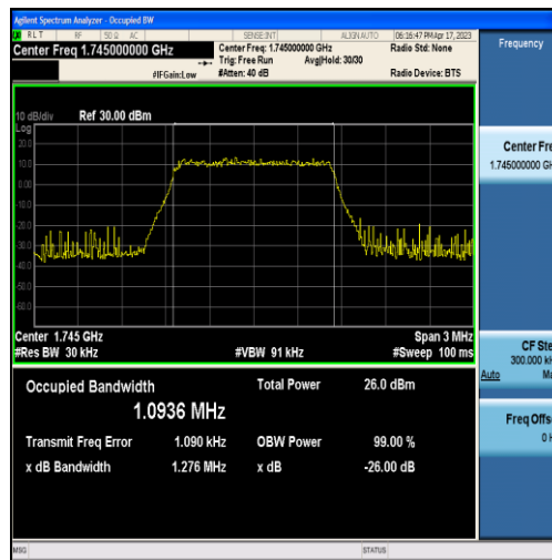
Band66-1.4MHz-16QAM-132322-6RB#0-1.0936
