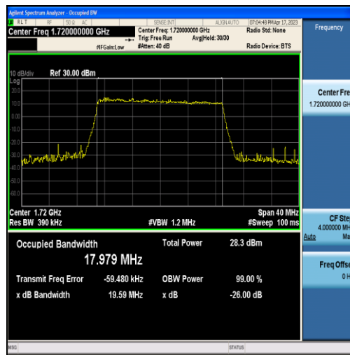
Band66-20MHz-QPSK-132072-100RB#0-17.979
