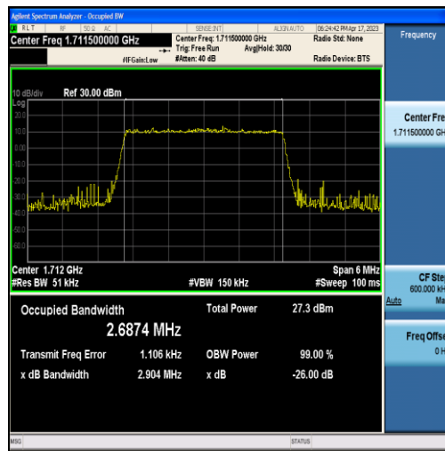
Band66-3MHz-QPSK-131987-15RB#0-2.6874
