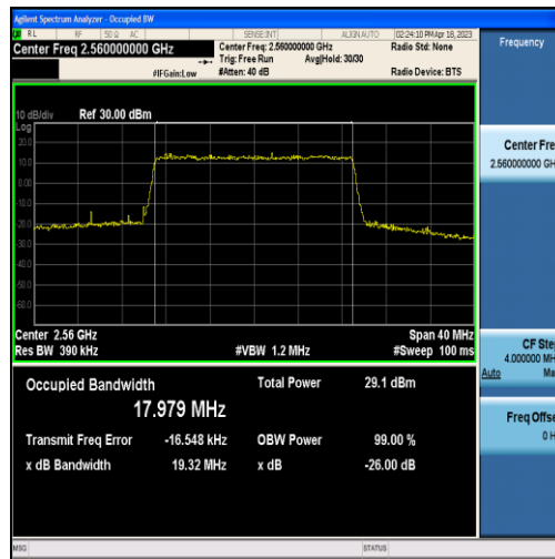
Band7-20MHz-QPSK-21350-100RB#0-17.979
