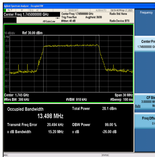
Band66-15MHz-QPSK-132322-75RB#0-13.498
