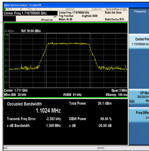
Band66-1.4MHz-16QAM-131979-6RB#0-1.1024
