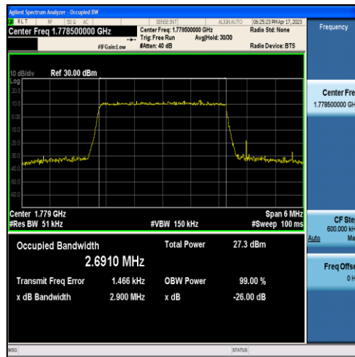
Band66-3MHz-QPSK-132657-15RB#0-2.6910
