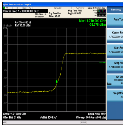
Band4-3MHz-16QAM-19965-15RB#0
