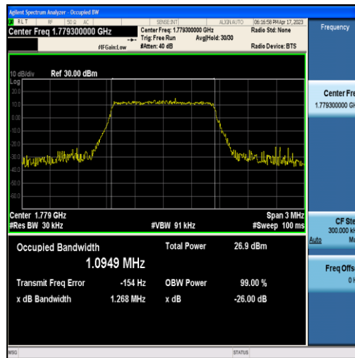
Band66-1.4MHz-QPSK-132665-6RB#0-1.0949
