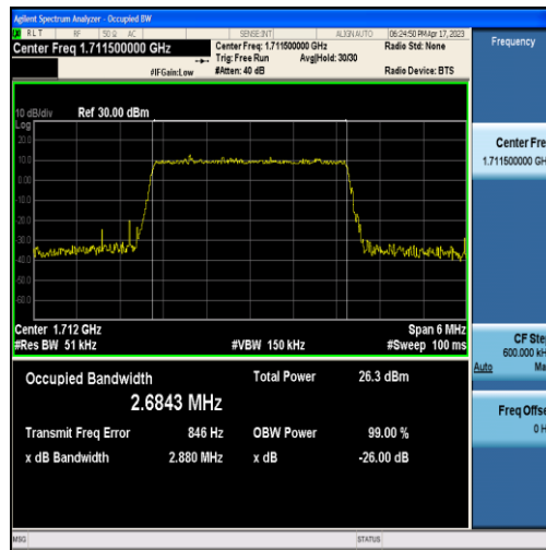
Band66-3MHz-16QAM-131987-15RB#0-2.6843
