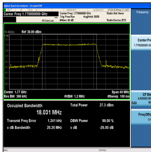
Band66-20MHz-16QAM-132572-100RB#0-18.031
