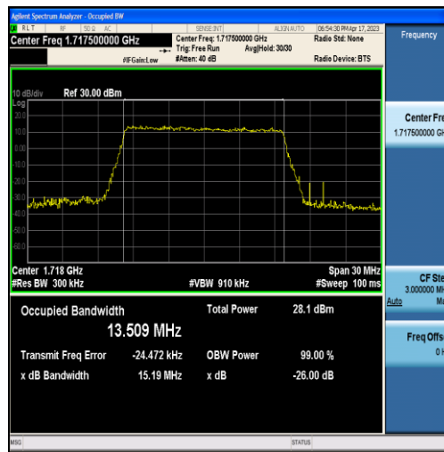
Band66-15MHz-QPSK-132047-75RB#0-13.509
