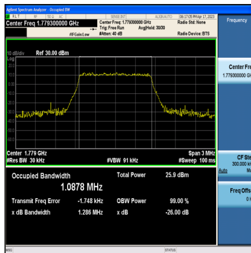
Band66-1.4MHz-16QAM-132665-6RB#0-1.0878
