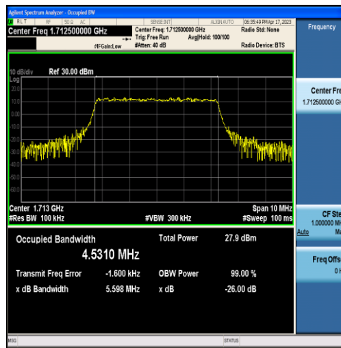
Band66-5MHz-QPSK-131997-25RB#0-4.5310
