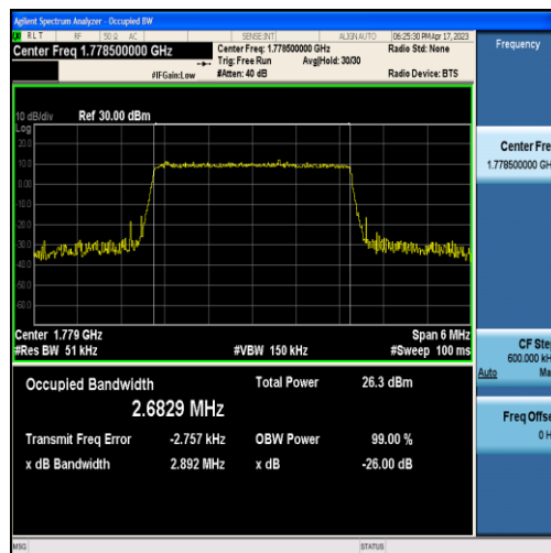
Band66-3MHz-16QAM-132657-15RB#0-2.6829
