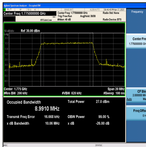
Band66-10MHz-16QAM-132622-50RB#0-8.9910
