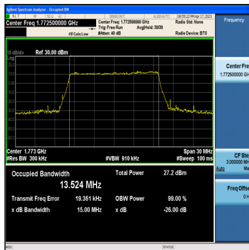
Band66-15MHz-16QAM-132597-75RB#0-13.524
