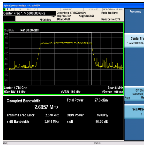
Band66-3MHz-QPSK-132322-15RB#0-2.6857
