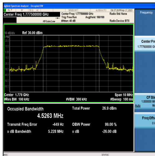
Band66-5MHz-16QAM-132647-25RB#0-4.5263
