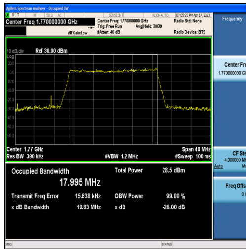
Band66-20MHz-QPSK-132572-100RB#0-17.995
