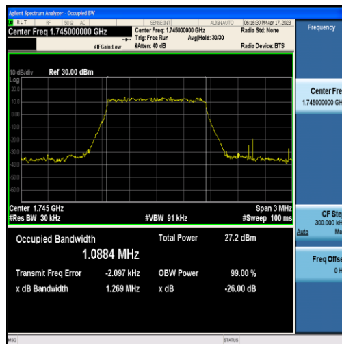
Band66-1.4MHz-QPSK-132322-6RB#0-1.0884
