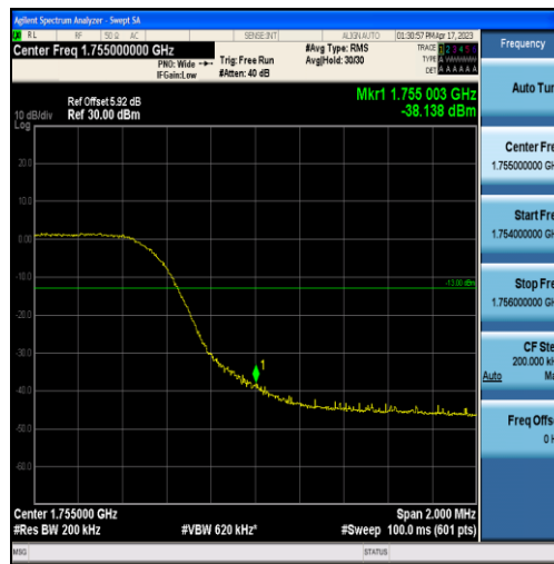
Band4-10MHz-QPSK-20350-50RB#0
