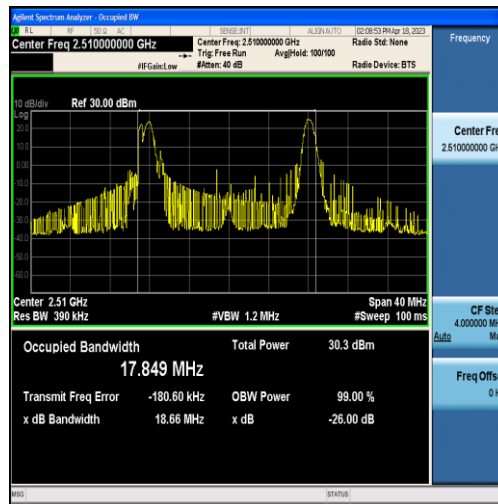
Band7-20MHz-16QAM-20850-60RB#0-17.849
