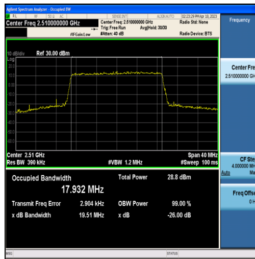
Band7-20MHz-QPSK-20850-100RB#0-17.932
