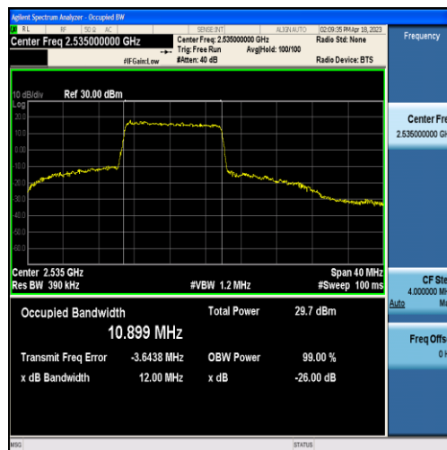
Band7-20MHz-QPSK-21100-60RB#0-10.899
