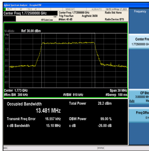
Band66-15MHz-QPSK-132597-75RB#0-13.481
