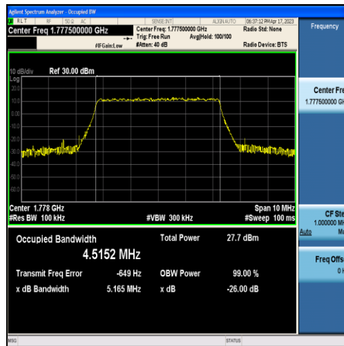
Band66-5MHz-QPSK-132647-25RB#0-4.5152
