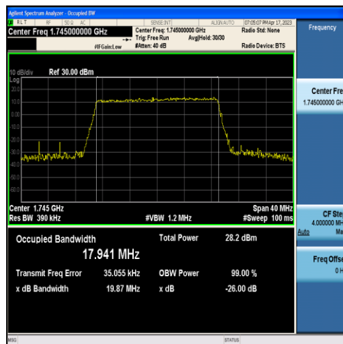
Band66-20MHz-QPSK-132322-100RB#0-17.941
