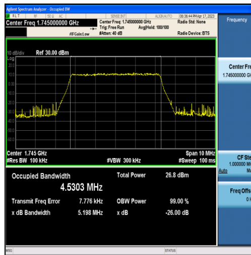
Band66-5MHz-16QAM-132322-25RB#0-4.5303
