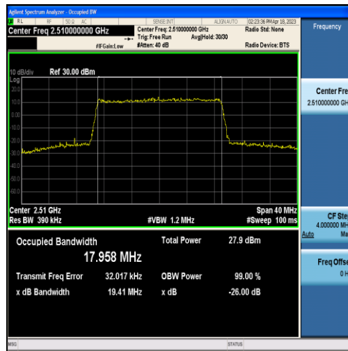
Band7-20MHz-16QAM-20850-100RB#0-17.958
