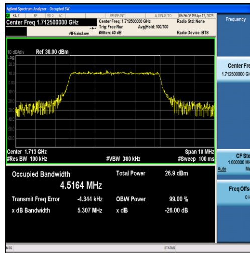
Band66-5MHz-16QAM-131997-25RB#0-4.5164
