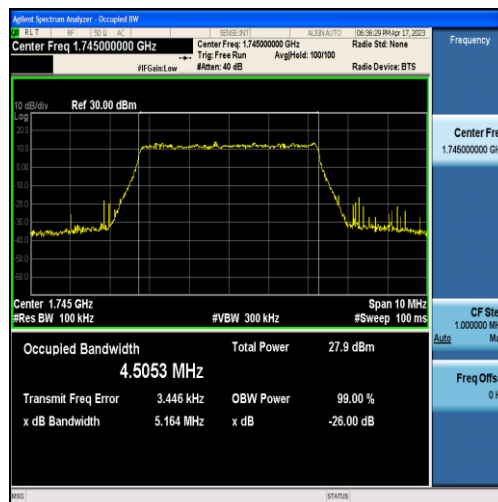
Band66-5MHz-QPSK-132322-25RB#0-4.5053
