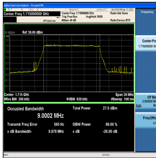
Band66-10MHz-16QAM-132022-50RB#0-9.0002
