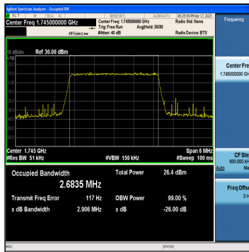
Band66-3MHz-16QAM-132322-15RB#0-2.6835
