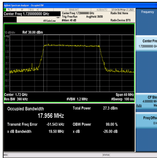
Band66-20MHz-16QAM-132072-100RB#0-17.956
